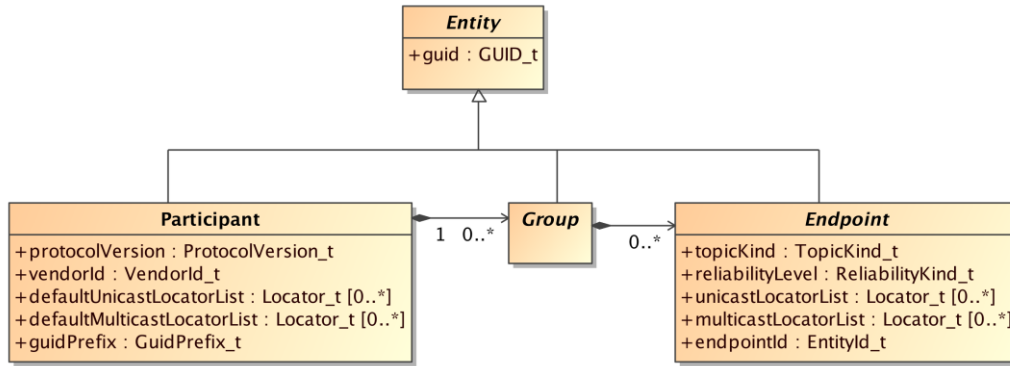
Figure 8.5 - RTPS Participant
