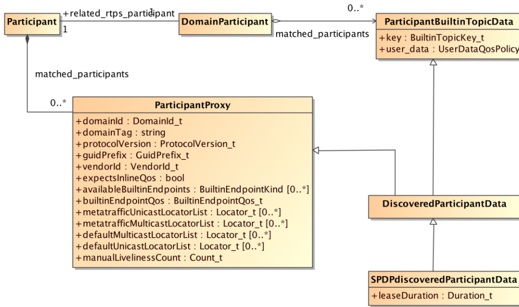
Figure 8.27 - SPDPdiscoveredParticipantData
