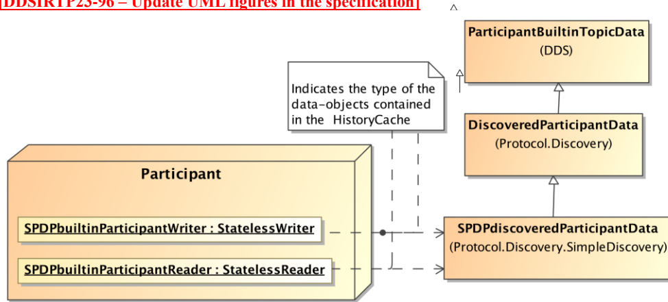
Figure 8.28 - The built-in Endpoints used by the Simple Participant Discovery Protocol
