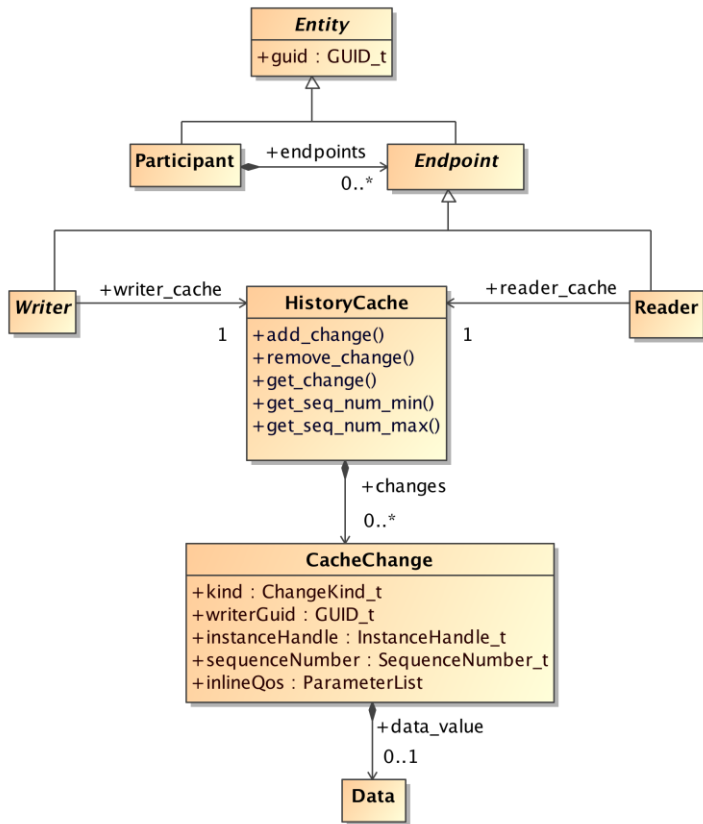
Figure 8.1 - RTPS Structure Module
