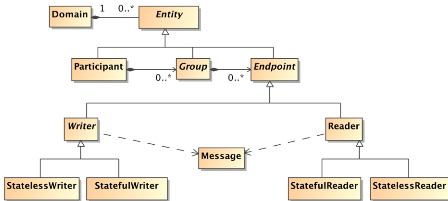
Figure 7.2 - RTPS Structure Module
