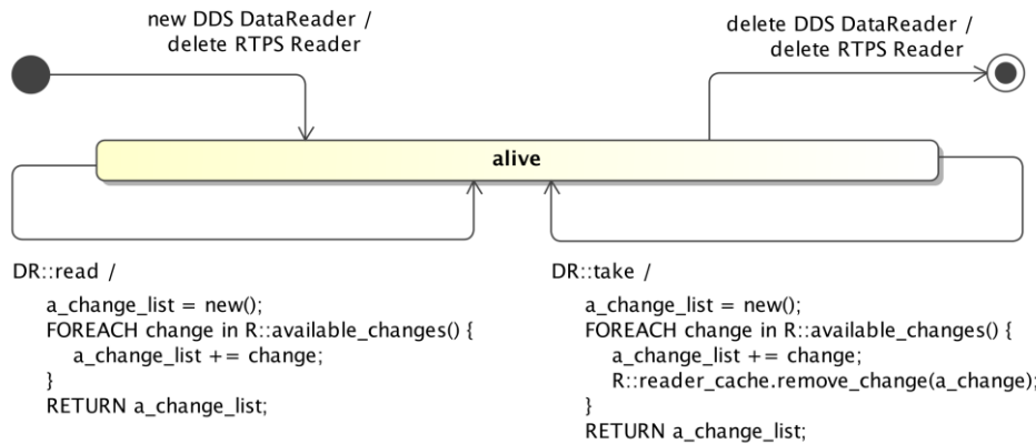
Figure 8.7 - DDS DataReader access to the HistoryCache
