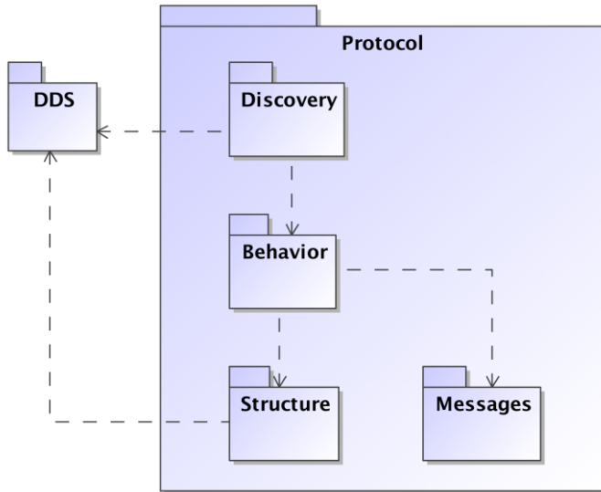
Figure 7.1 - RTPS Modules
