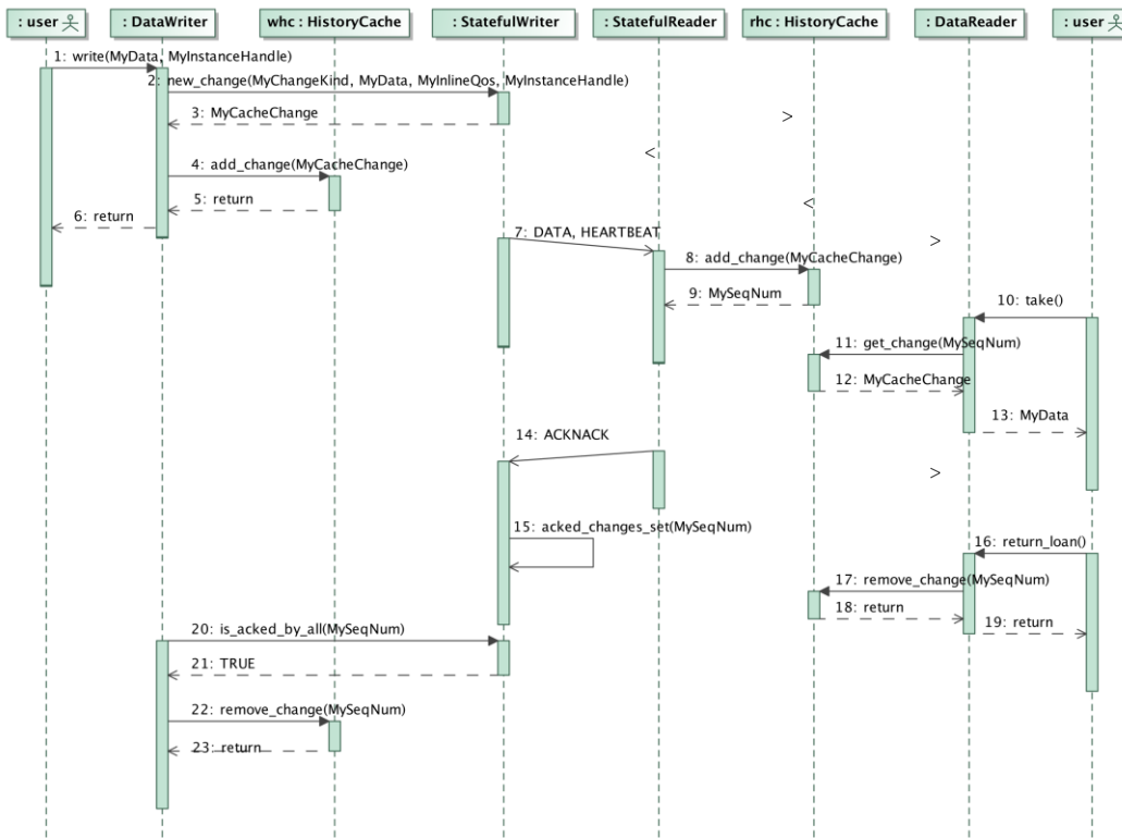
Figure 8.14 – Example Behavior
