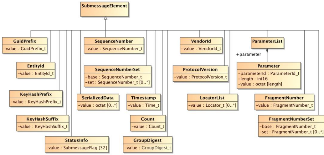
Figure 8.12 - RTPS SubmessageElements
