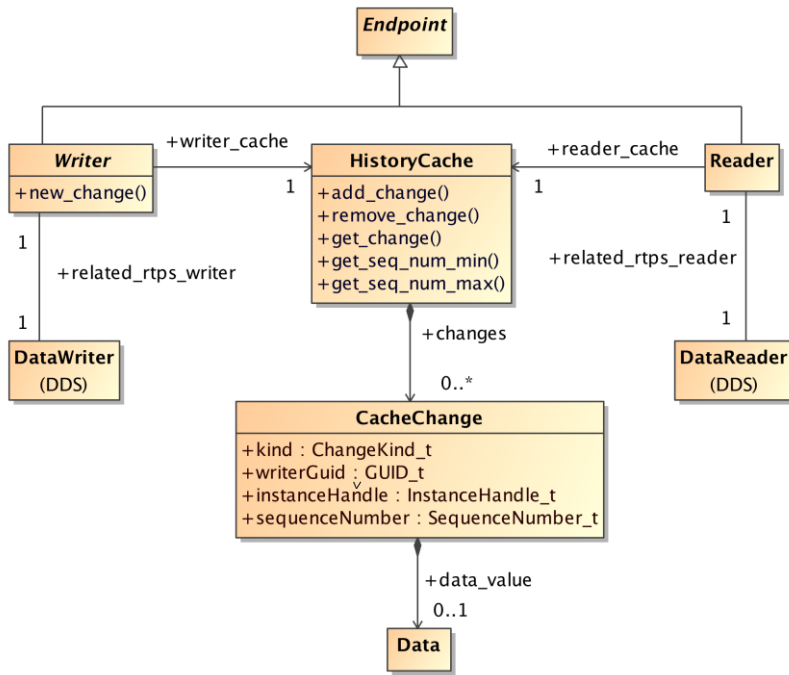
Figure 8.3 - RTPS HistoryCache
