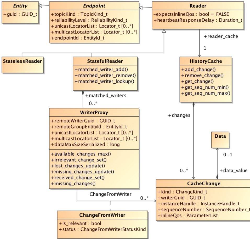
Figure 8.21 - RTPS Reader endpoints
