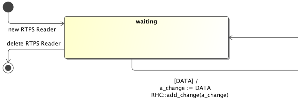
Figure 8.22 - Behavior of the Best-Effort StatelessReader
