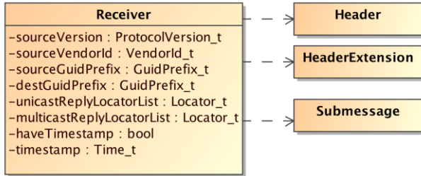
Figure 8.11 - RTPS Receiver
