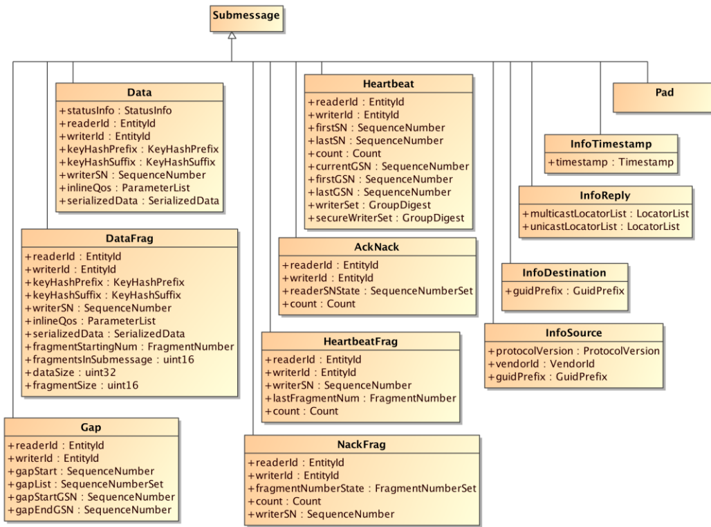
Figure 8.13 - RTPS Submessages
