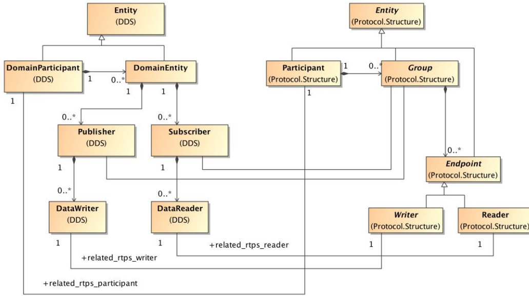
Figure 7.3 - Correspondence between RTPS and DDS Entries
