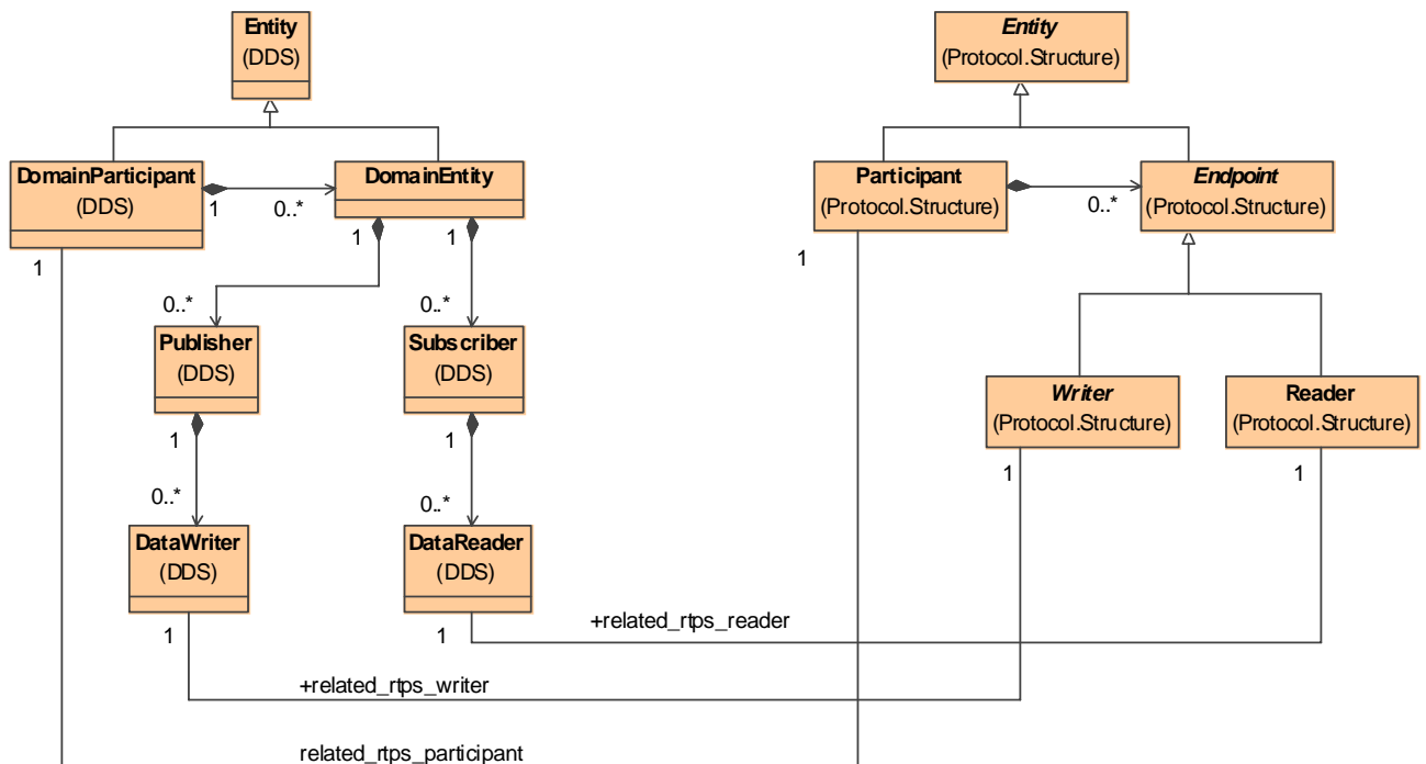
Figure 7.3 - Correspondence between RTPS and DDS Entries
