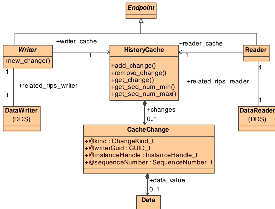
Figure 8.3 - RTPS HistoryCache
