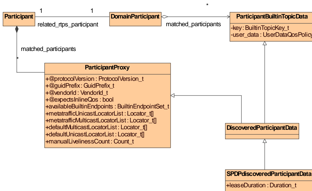
Figure 8.27 - SPDPdiscoveredParticipantData
