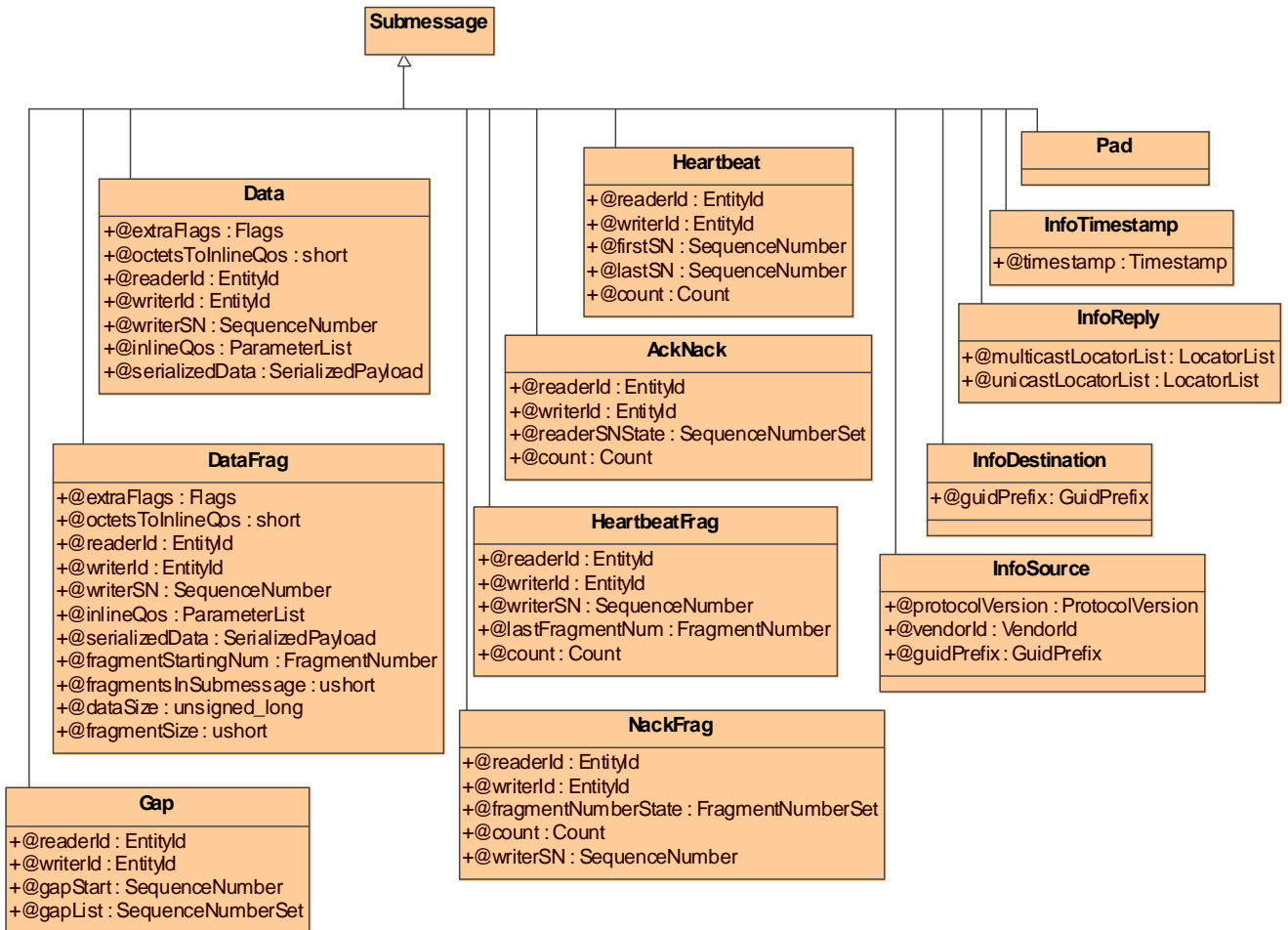
Figure 8.13 - RTPS Submessages
