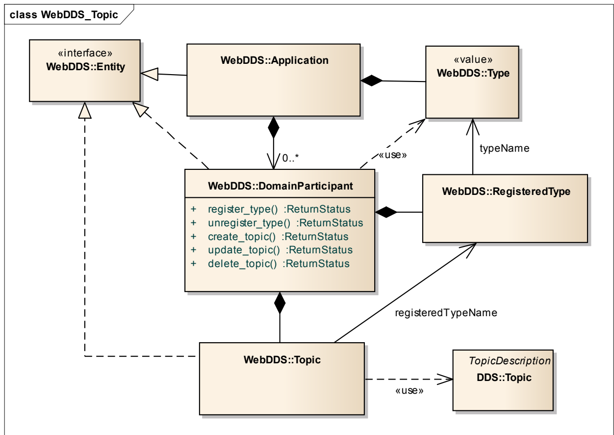
Figure 13—Participant class operations related to types and topics
