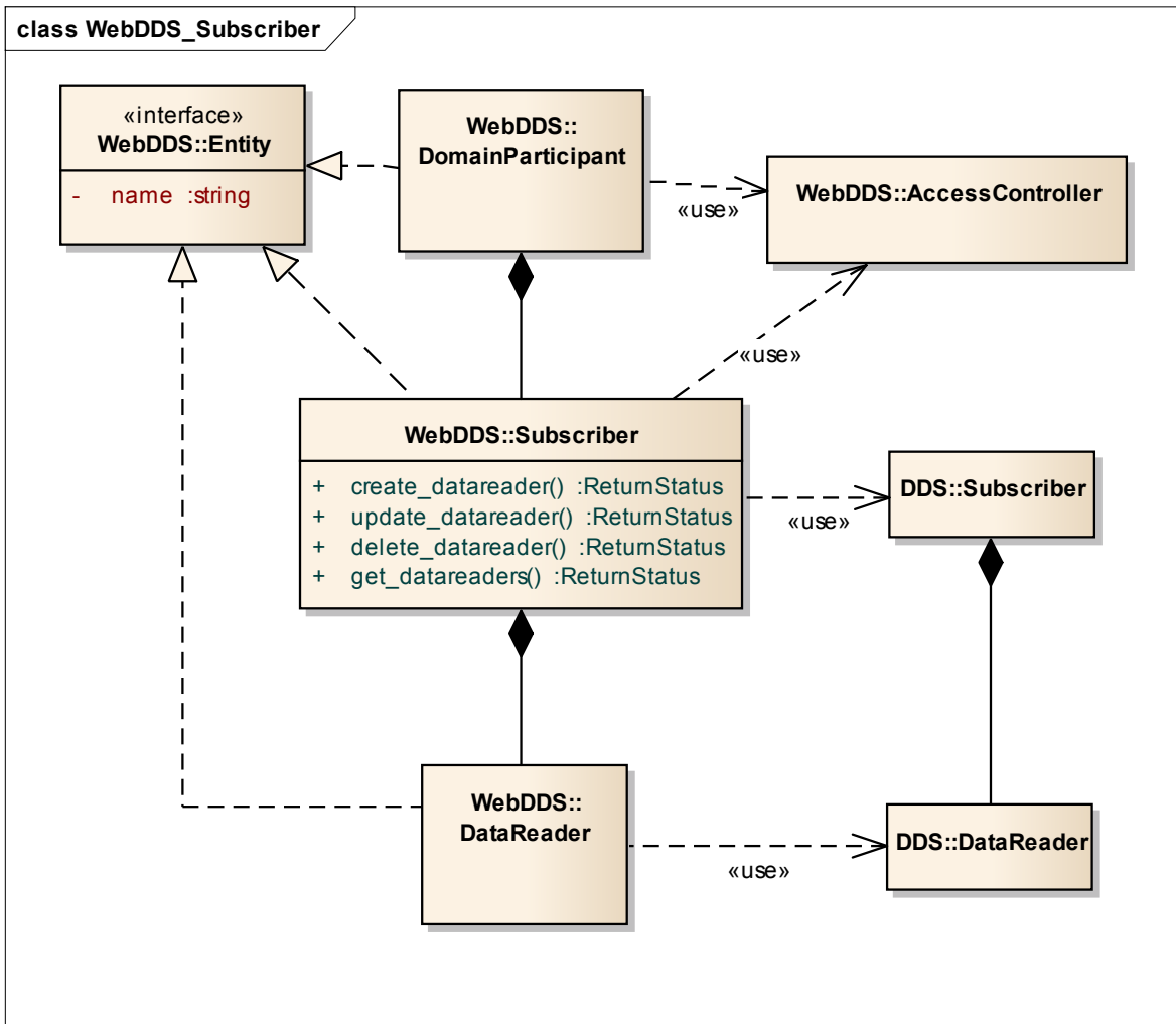
Figure 15—Subscriber class with operations
