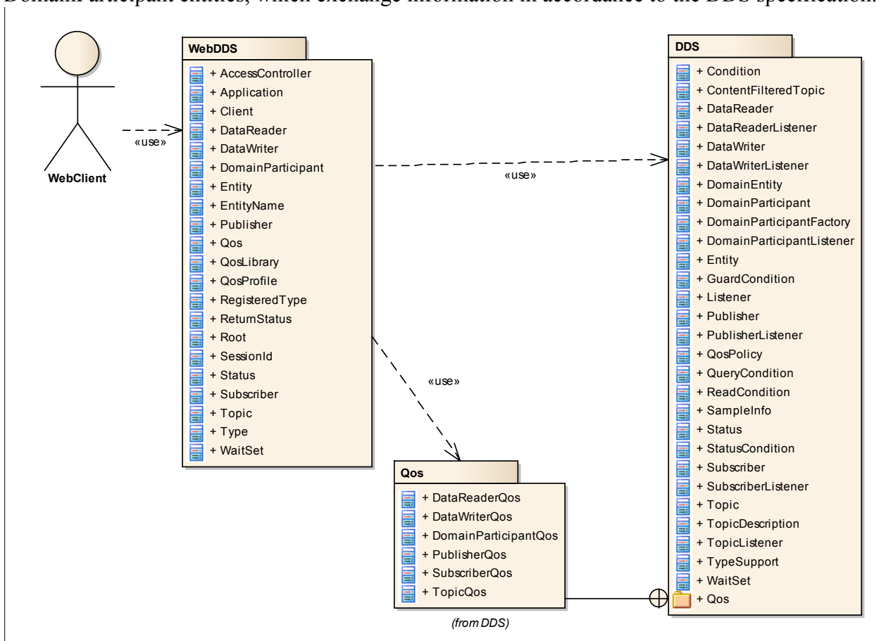
Figure 3— WebDDS Object Model Overview
