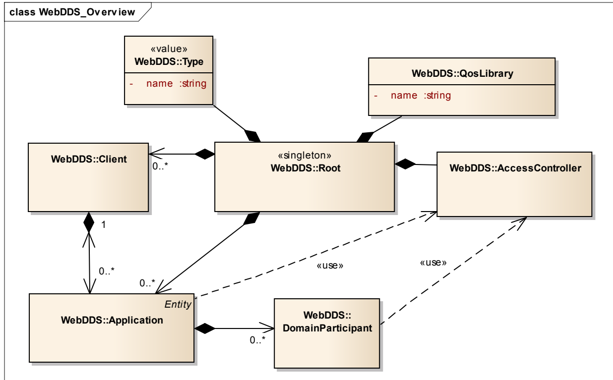
Figure 4—WebDDS Object Model Overview
