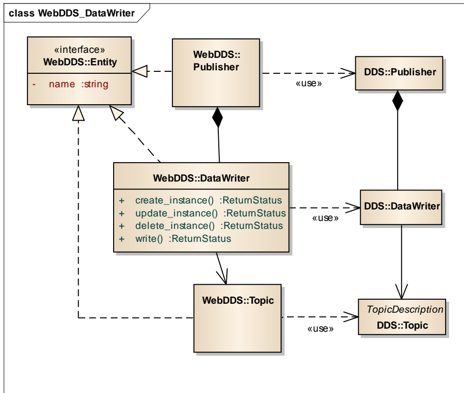
Figure 16—DataWriter class with operations
