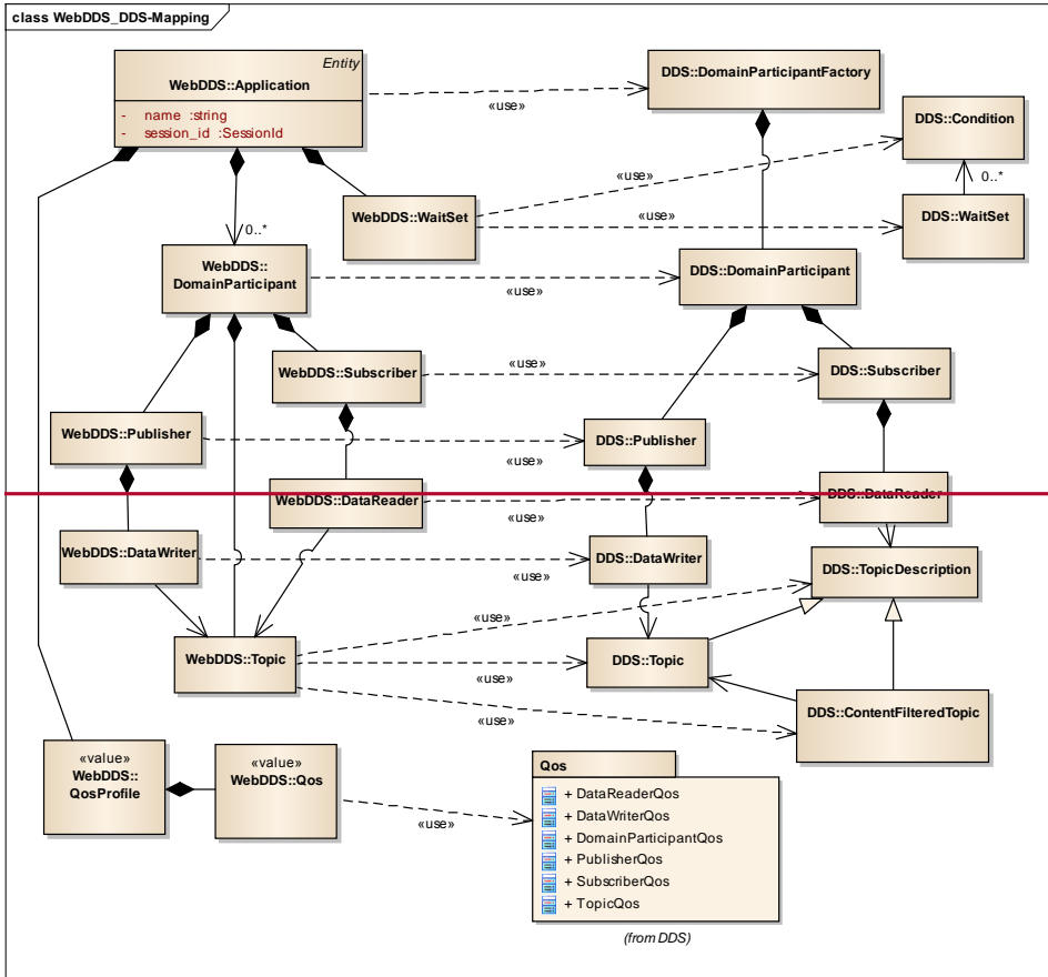
Figure 10—Mapping of WebDDS Object Model classes to DDS Object Model classes
