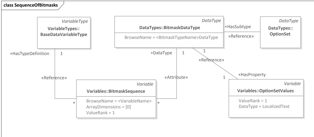
Figure 9.22: Sequence of Bitmasks Variable Definition
