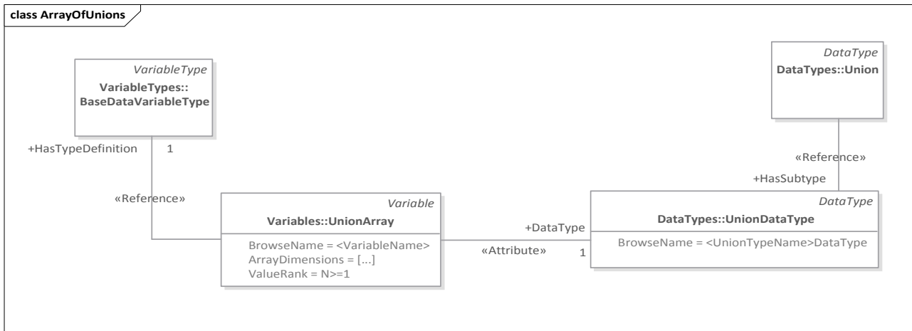
Figure 9.18: Array of Unions Mapping to OPC UA
