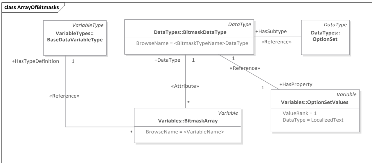
Figure 9.16: Array of Bitmasks Mapping to OPC UA
