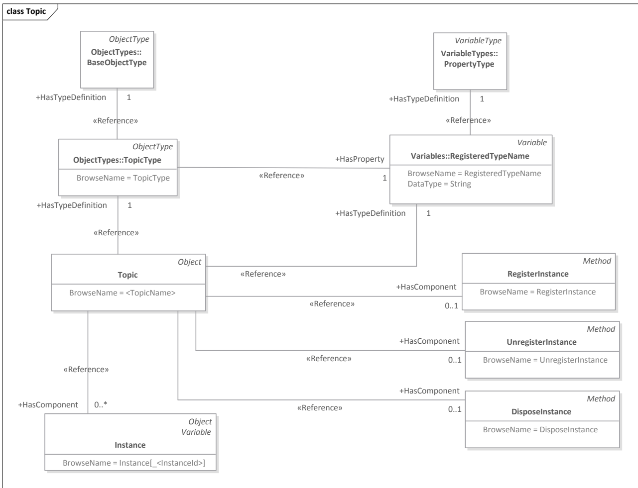
Figure 9.29: DDS Topic Mapping to OPC UA
