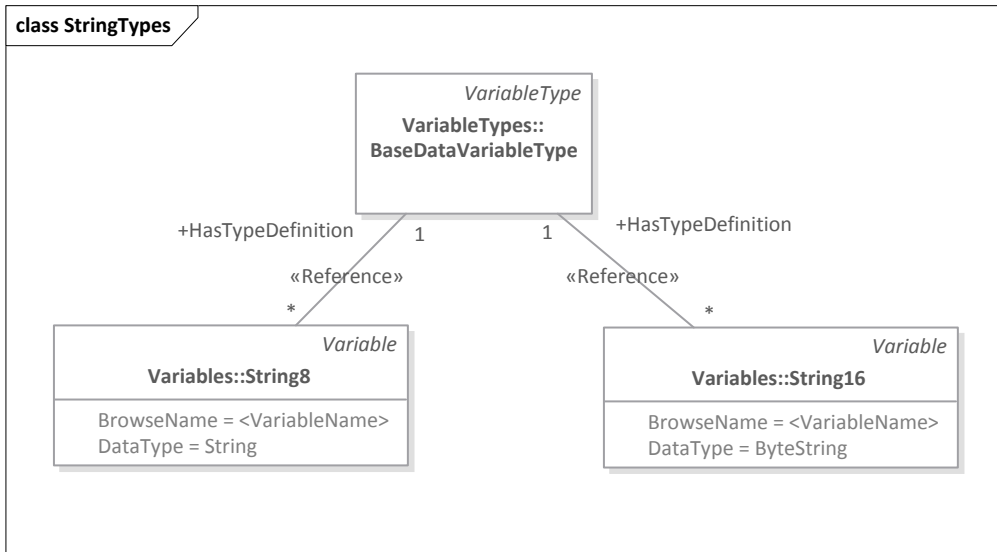
Figure 9.4: String Types Mapping to OPC UA
