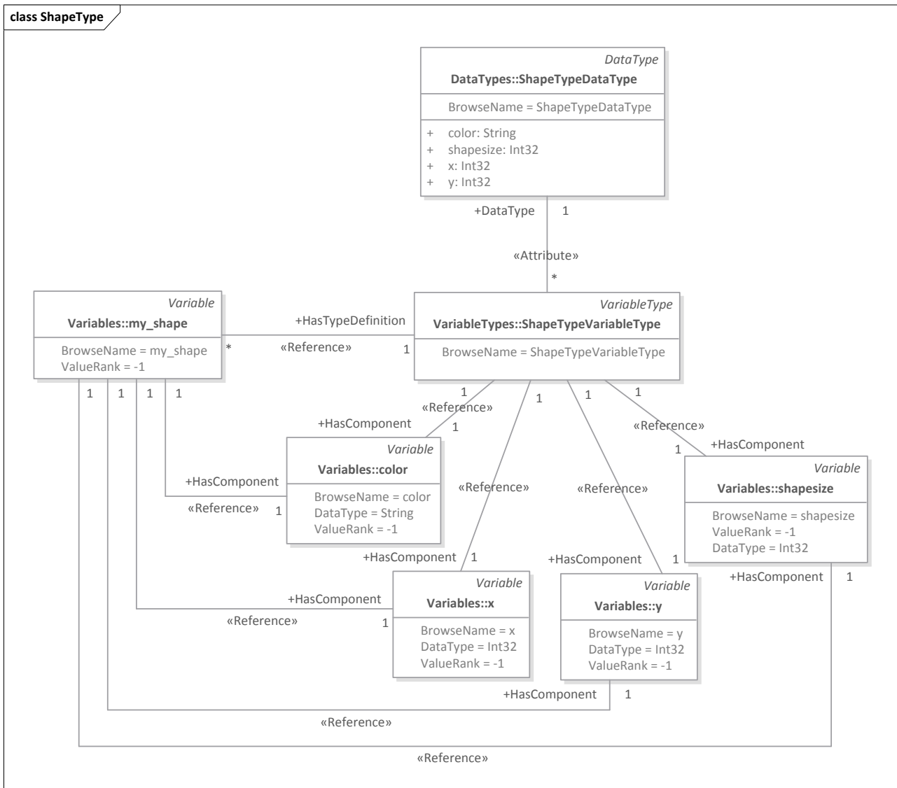
Figure 9.11: Example of Structure Type Mapping to OPC UA
