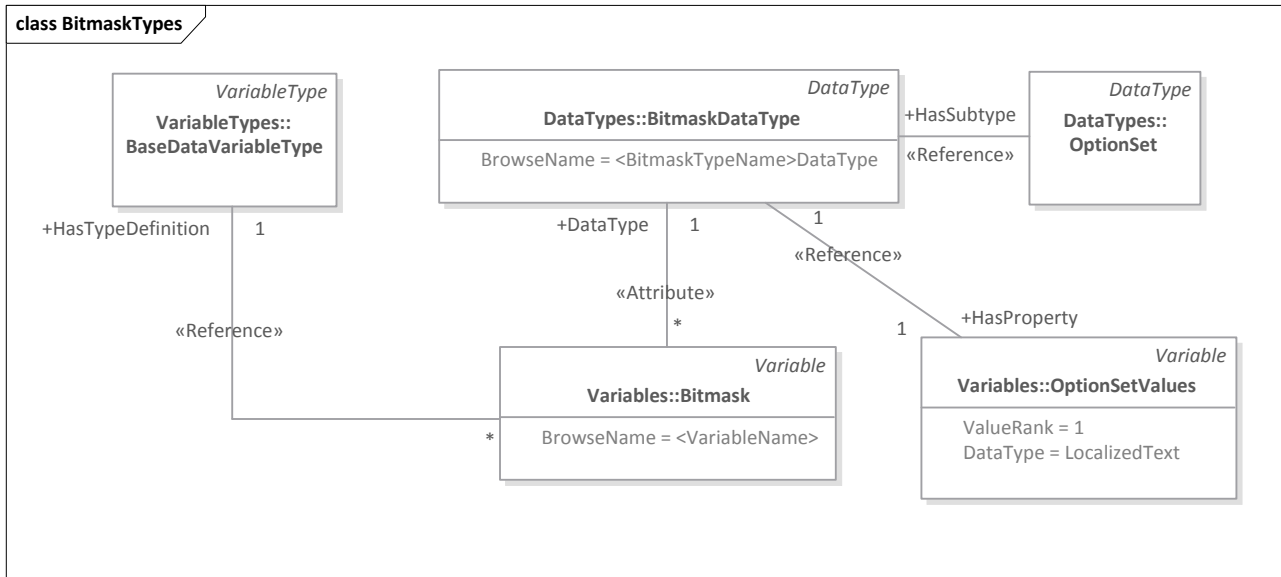
Figure 9.8: Bitmask Types Mapping to OPC UA
