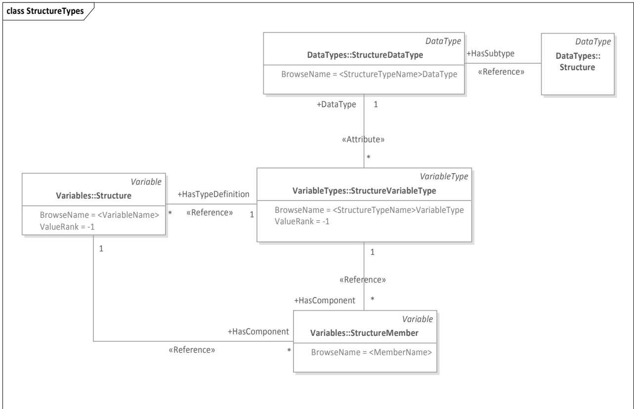
Figure 9.10: Structure Types Mapping to OPC UA
