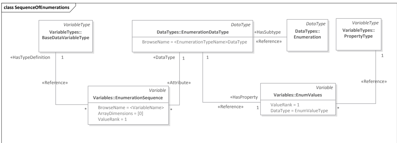
Figure 9.21: Sequence of Enumerations Mapping to OPC UA
