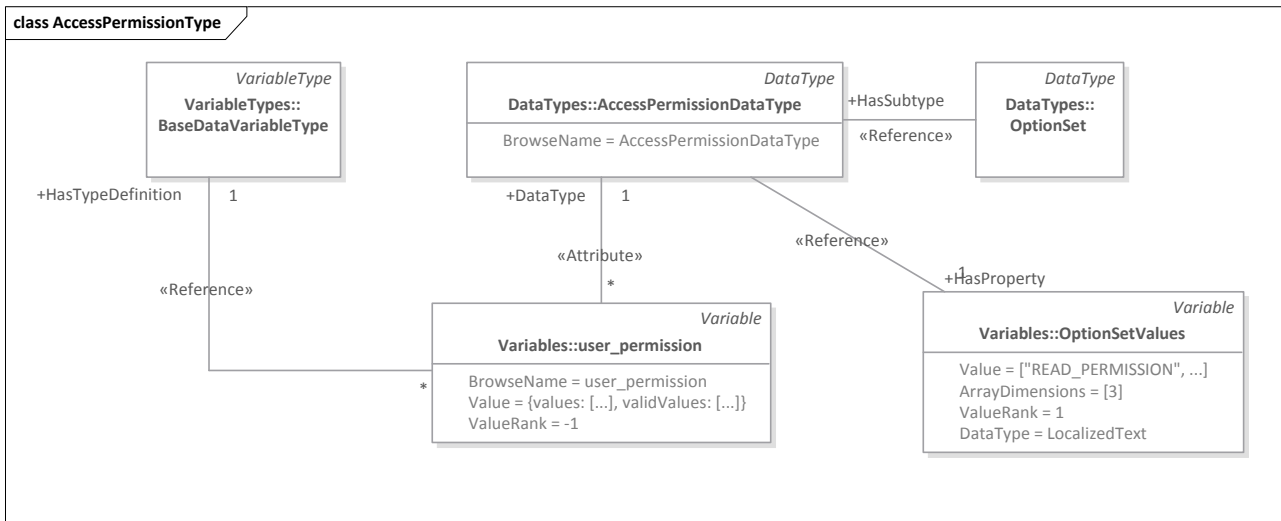
Figure 9.9: Example of Bitmask Type Mapping to OPC UA
