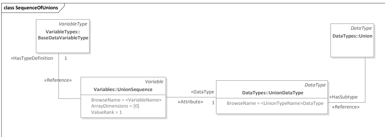
Figure 9.24: Sequence of Unions Mapping to OPC UA
