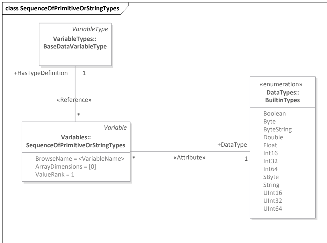
Figure 9.20: Sequence of Primitive or String Types Mapping to OPC UA
