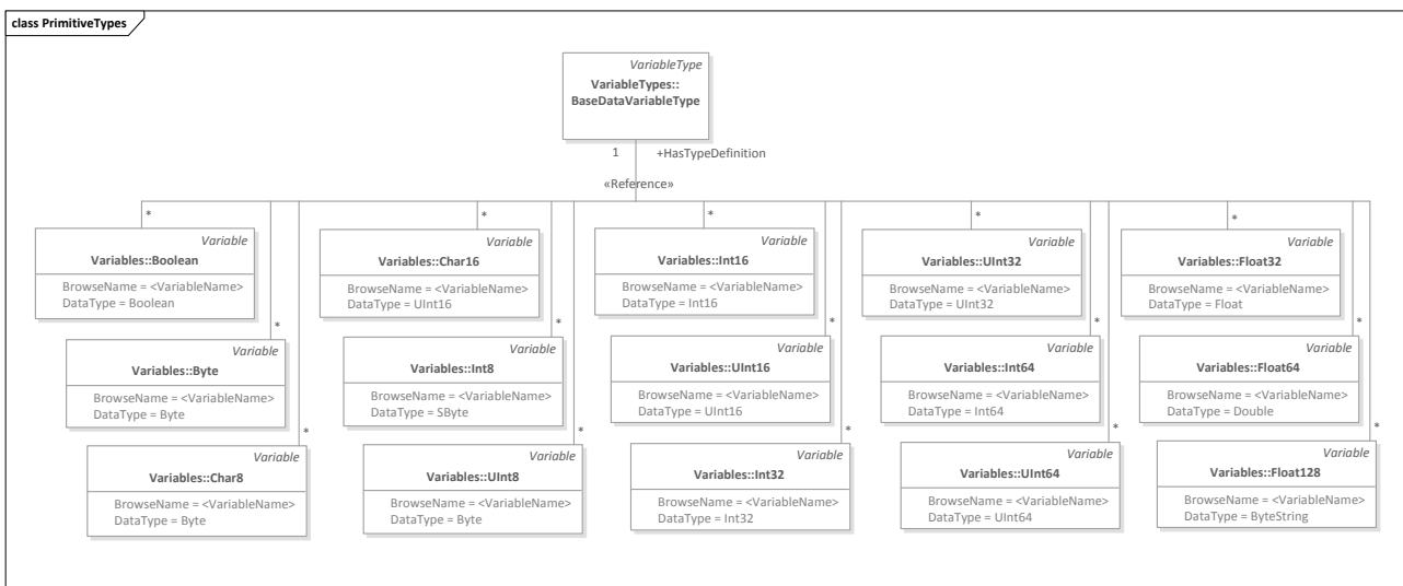
Figure 9.2: Primitive Types Mapping to OPC UA
