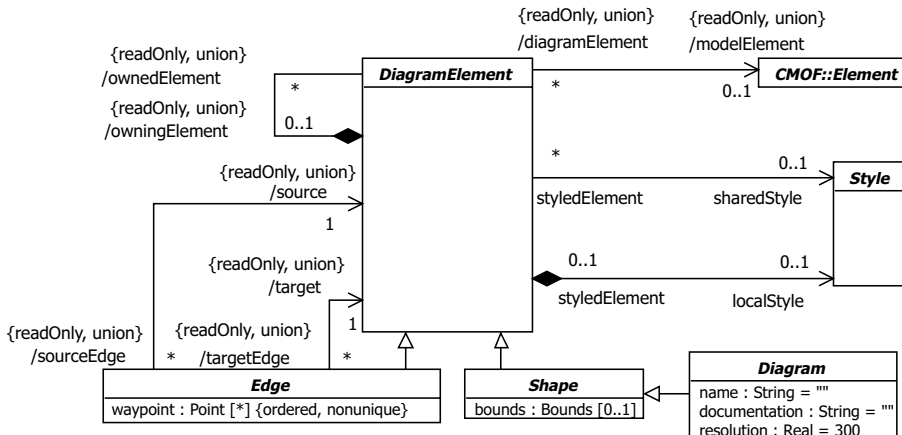
Figure 9.2 - Diagram Element
