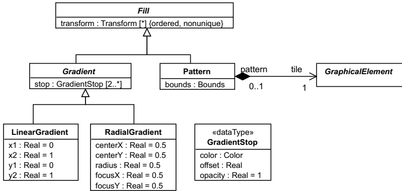
Figure 10.6 - Fills
