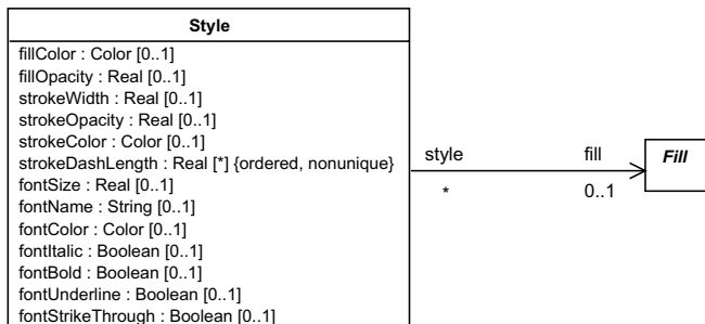
Figure 10.5 - Style
