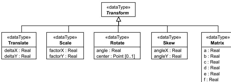
Figure 10.7 - Transforms
