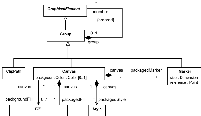
Figure 10.4 - Group Elements
