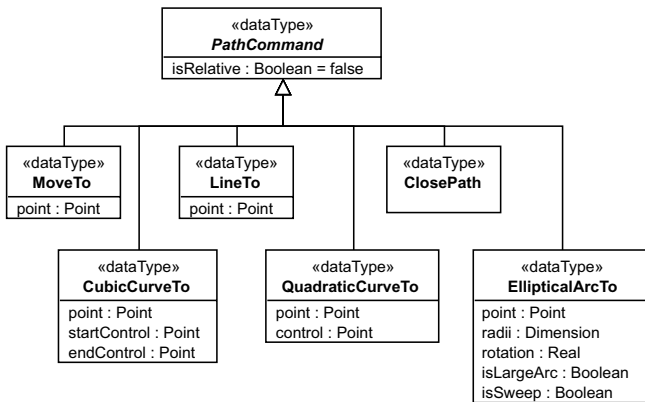
Figure 10.8 - Path Commands
