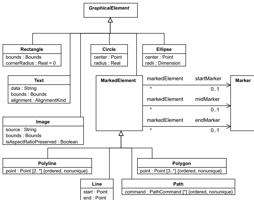
Figure 10.3 - Primitive Elements
