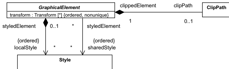
Figure 10.2 - Graphical Element
