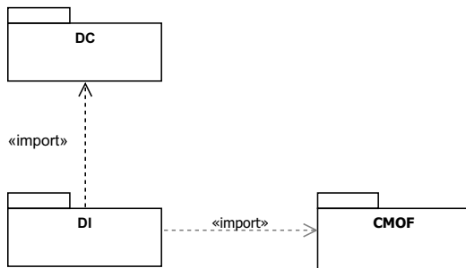
Figure 9.1 - Dependencies of the DI package
