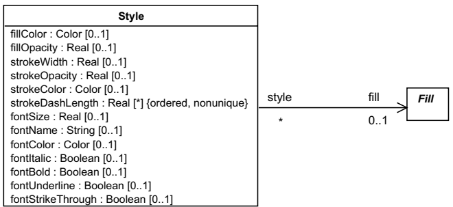
Figure 10.5 - Style
