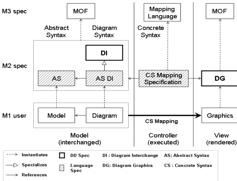
Figure 7.1 - Diagram Definition Architecture
