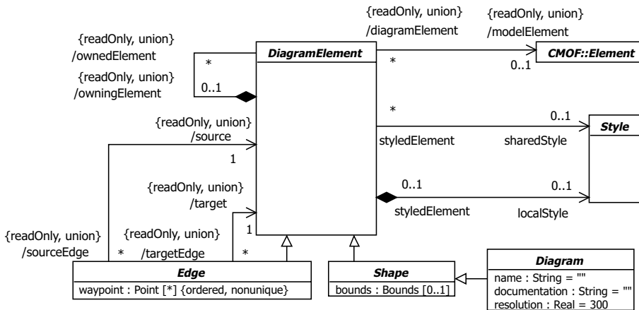
Figure 9.2 - Diagram Element
