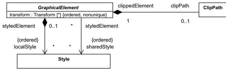
Figure 10.2 - Graphical Element
