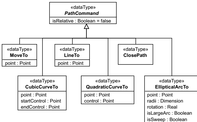
Figure 10.8 - Path Commands
