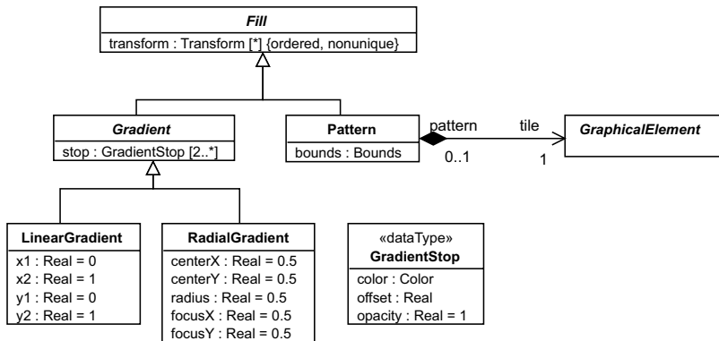
Figure 10.6 - Fills
