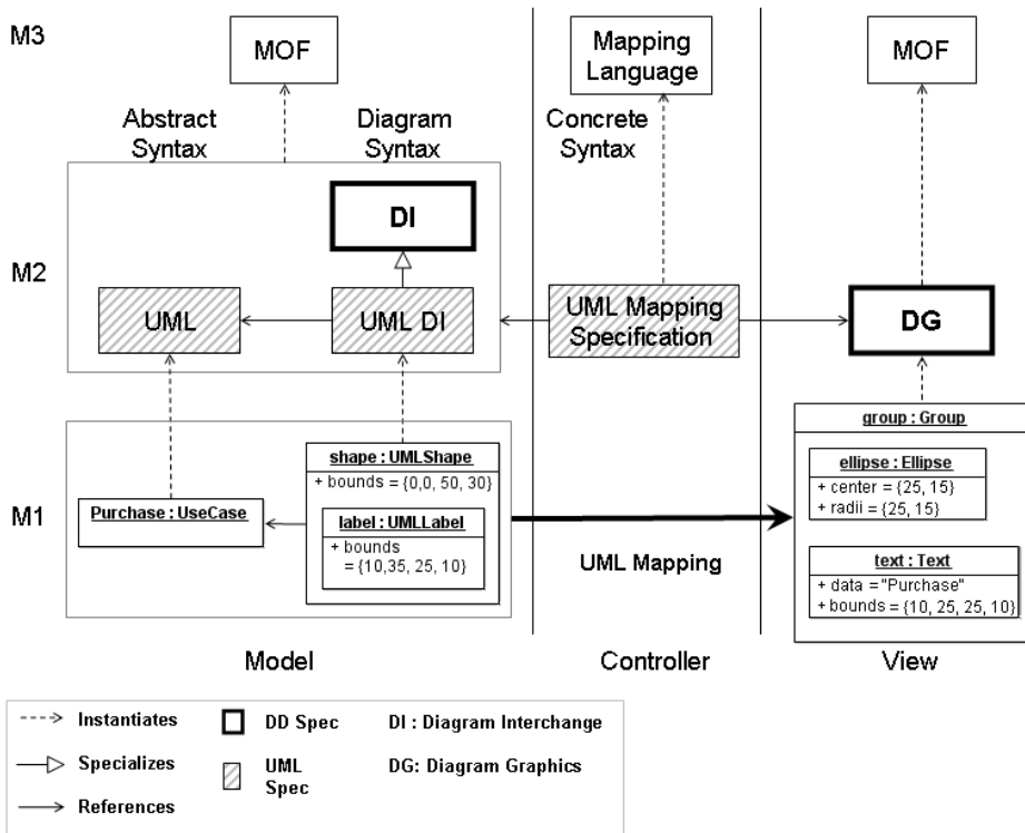
Figure 7.2 - Example of Diagram Definition Architecture For UML
