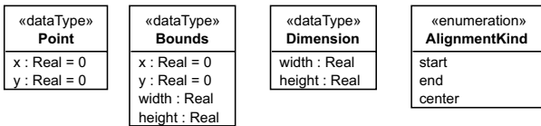
Figure 8.2 - The layout data types
