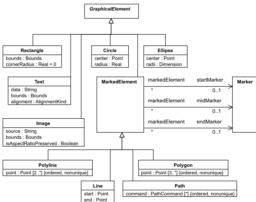
Figure 10.3 - Primitive Elements
