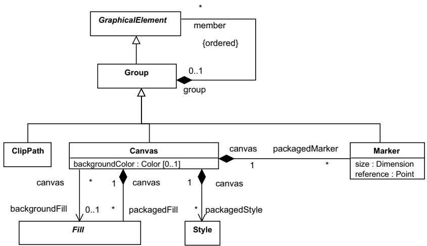
Figure 10.4 - Group Elements
