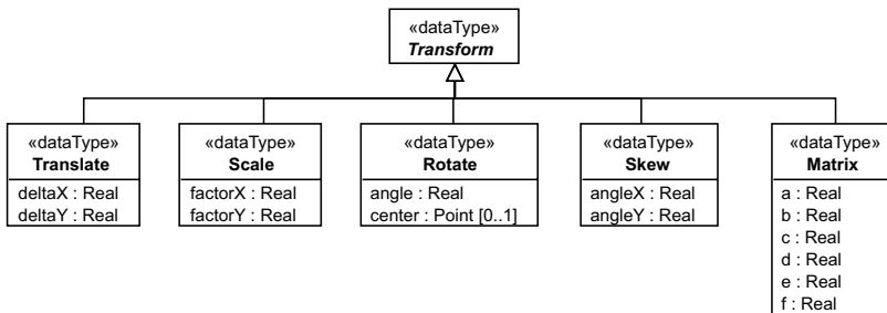
Figure 10.7 - Transforms
