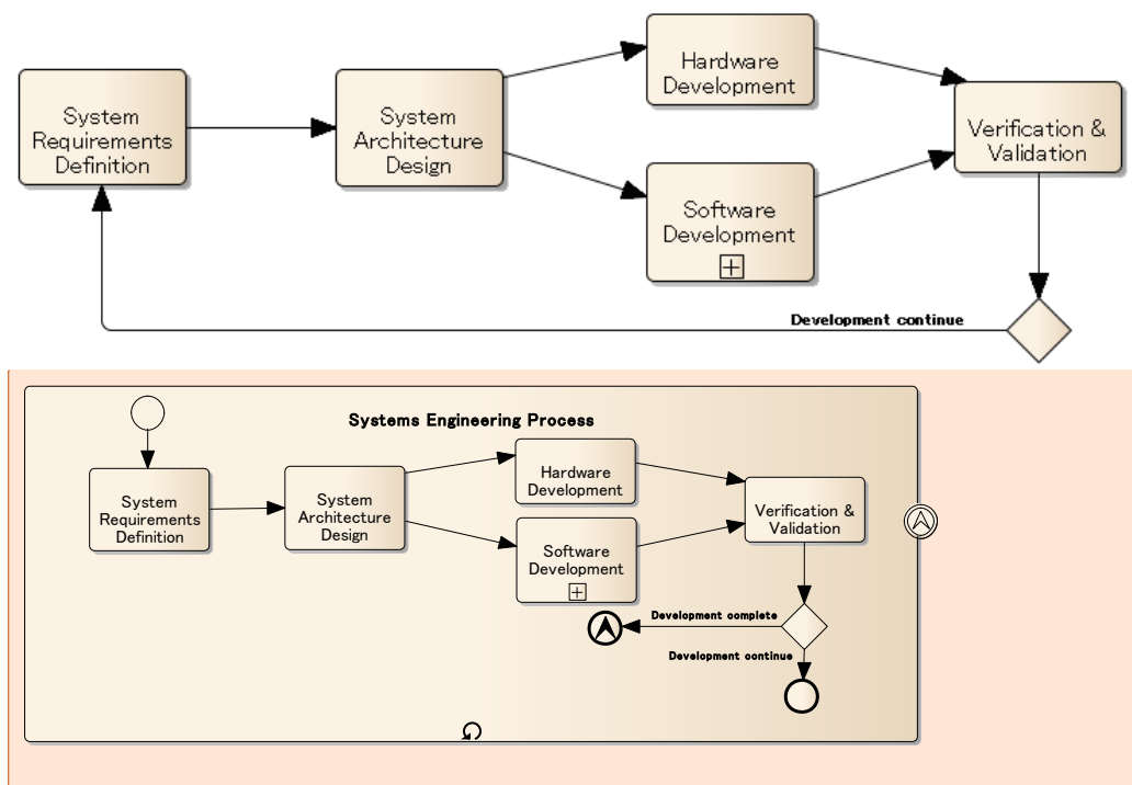
Figure 9-3 – BPMN for Systems Engineering Process
