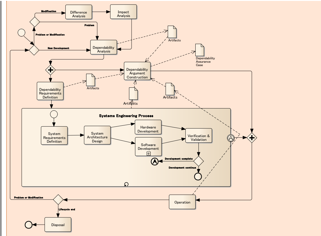
Figure 9-2 – BPMN for Dependability Process Model
