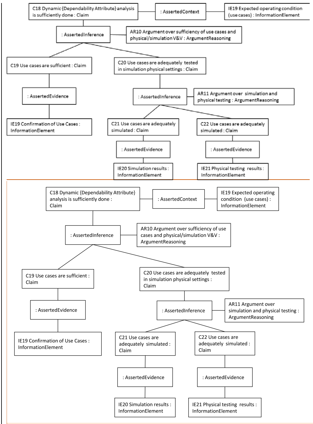
Figure 8-9 – Dynamic Dependability Analysis Argument part of the DAC template for Evolutionary Development Argument Structure
