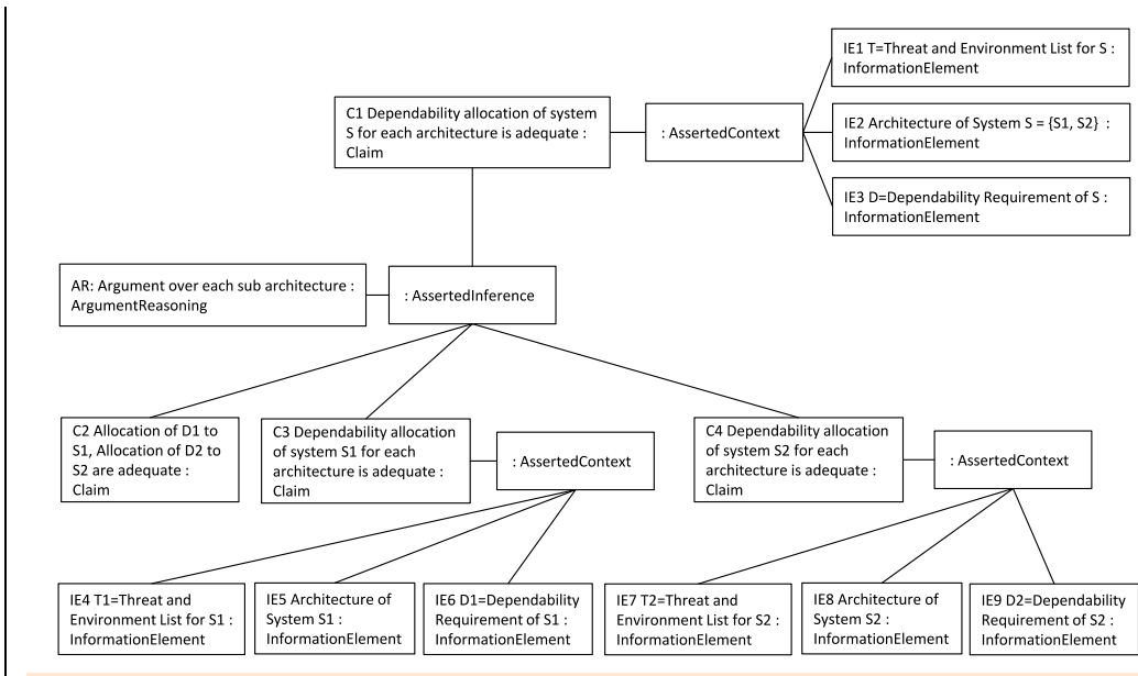
Figure 8-1 – DAC template for Dependability Allocation Argument
