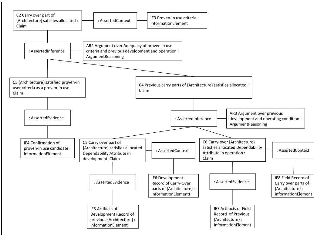
Figure 8-5 – Proven In Use Argument part of the Evolutionary Development Argument Structure
