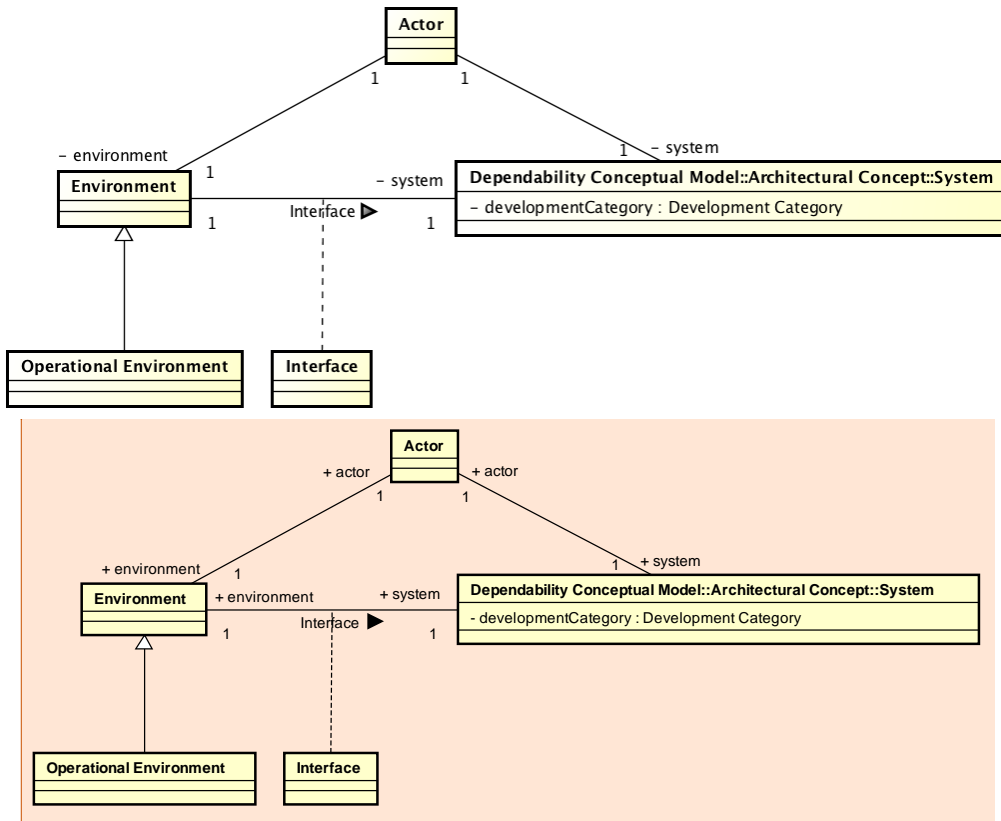
Figure 7-17 – System Environment Concept package
