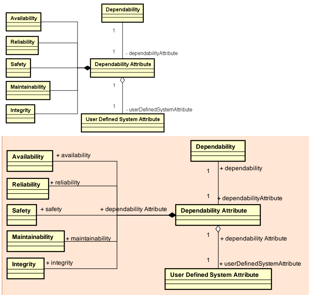
Figure 7-8 – Sample extension of Dependability Attribute (Informative)
