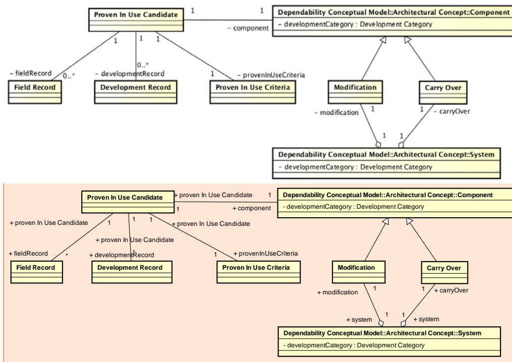
Figure 7-14 – Proven In Use package
