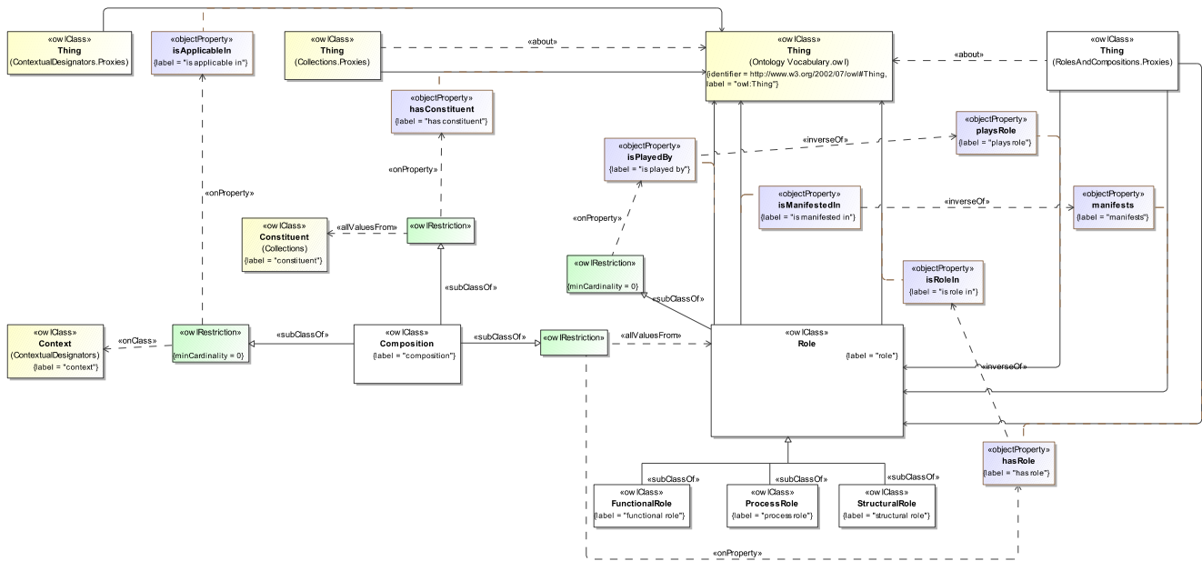
Figure 19: Roles and Compositions Ontology Overview
