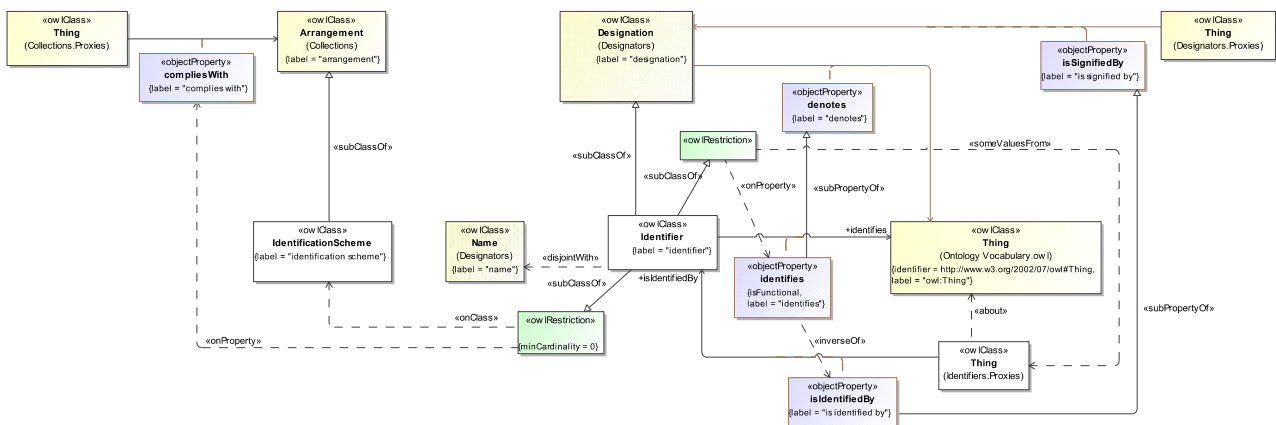
Figure 11: Overview of the Identifiers Ontology
