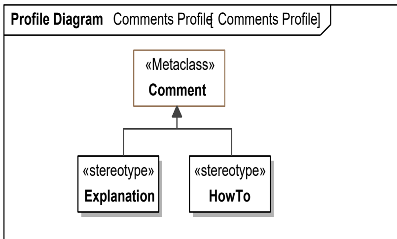
Figure 6 Comments Profile
