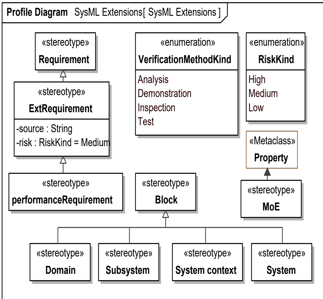
Figure 7 SysML Extensions
