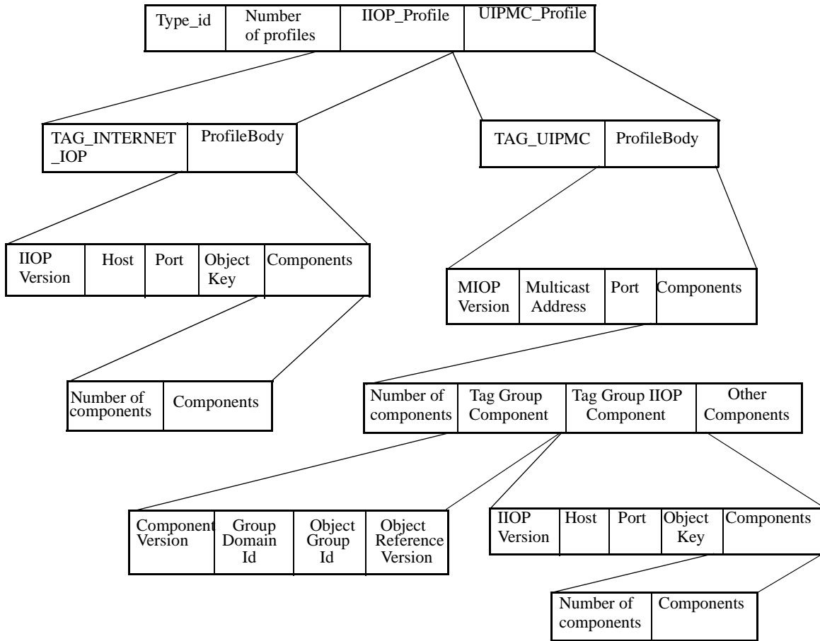
Figure 8.1 - An example of the Group Interoperable Object Reference used for Unreliable Multicast.
