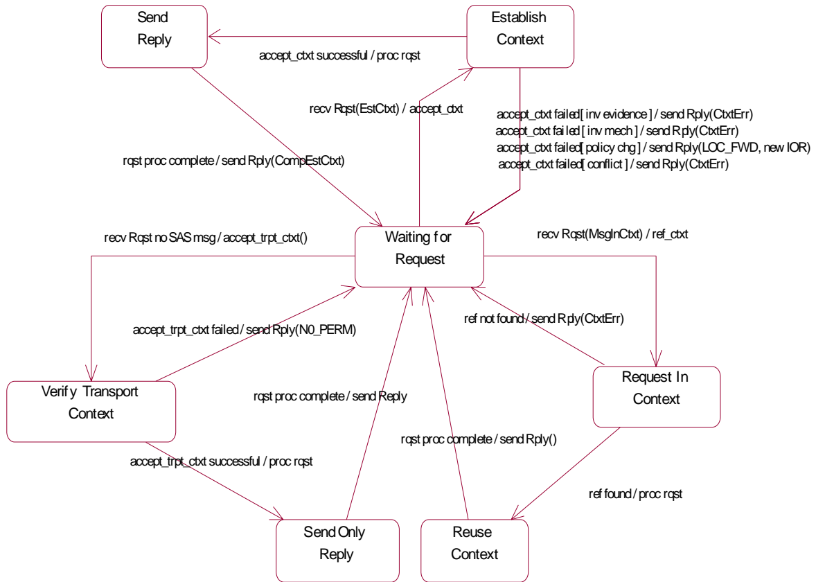
Figure 10.3 - TSS State Machine
