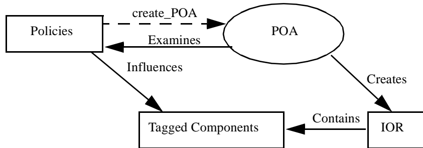
Figure 21-1 Object Creation
