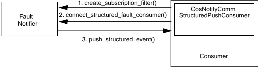
Figure 25-11 Connection Setup between the Consumer and the Fault Notifier
