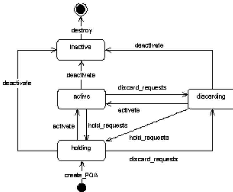
Figure 11-3 Processing States
