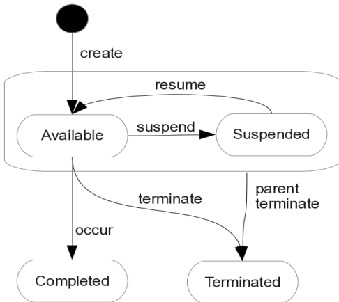
Figure 8.4 - Lifecycle of an EventListener or Milestone instance
