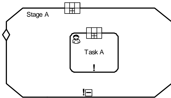
Figure 6.50 - Expanded Stage with Collapsed PlanningTable
