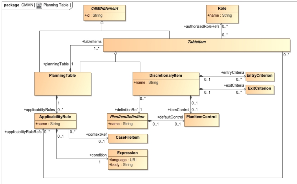
Figure 5.11 - PlanningTable class diagram
