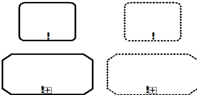
Figure 6.59 - Required Decorator example on Task and Stage
