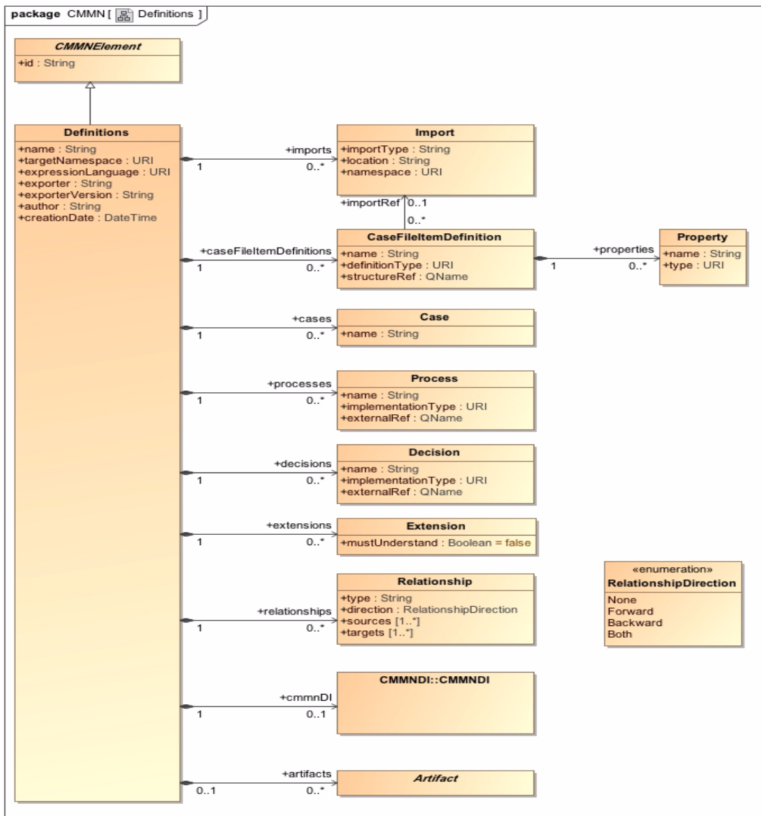
Figure 5.2 - Definitions class diagram
