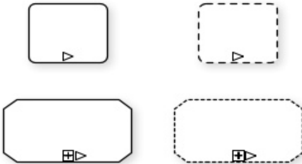
Figure 6.57 - ManualActivation Decorator example on Task and Stage
