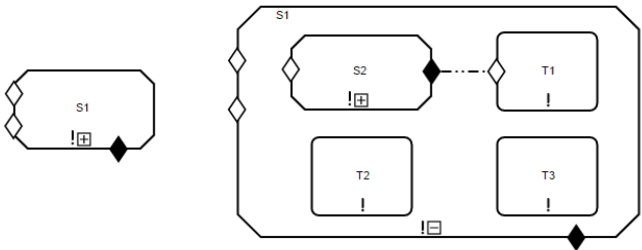
Figure 6.8 - Collapsed and Expanded versions of a Stage with two entry criterion, one sub Stage and three Tasks
