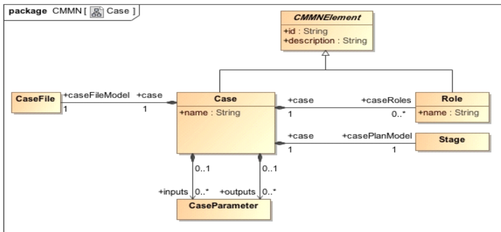
Figure 5.4 - Case class diagram
