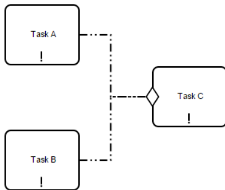
Figure 6.37 - Using Sentry-based connectors to visualize "AND"
