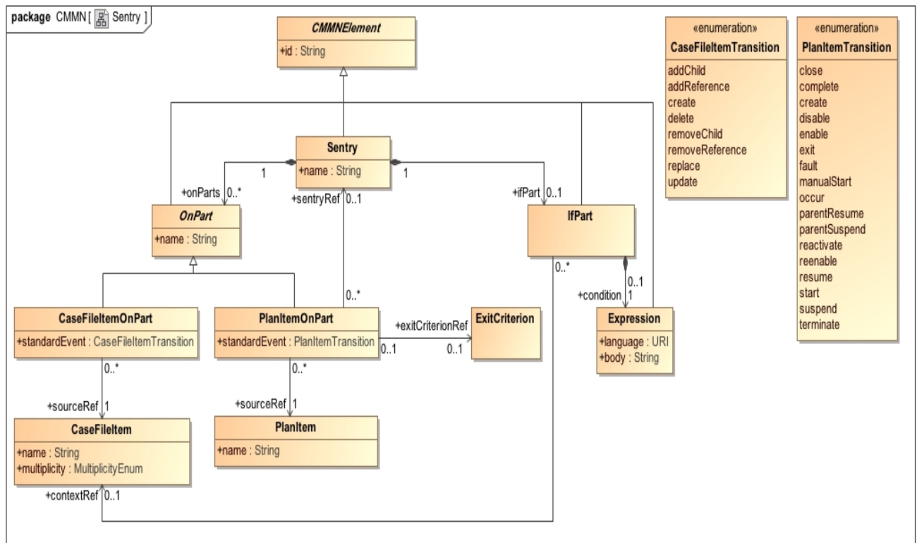
Figure 5.9 - Sentry class diagram
