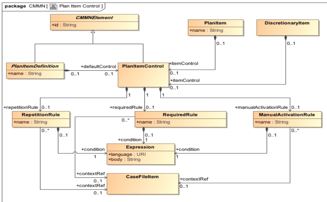
Figure 5.13 - PlanItemControl class diagram
