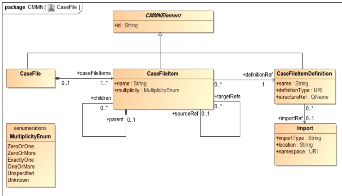
Figure 5.5 - CaseFile class diagram
