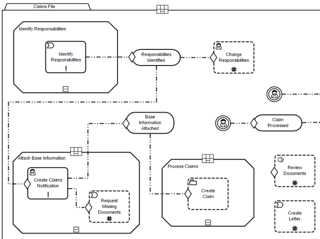
Figure 6.73 - Claims Management Example
