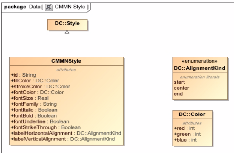
Figure 7.7 - CMMNStyle
