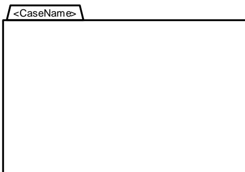
Figure 6.1 - CasePlanModel Shape
