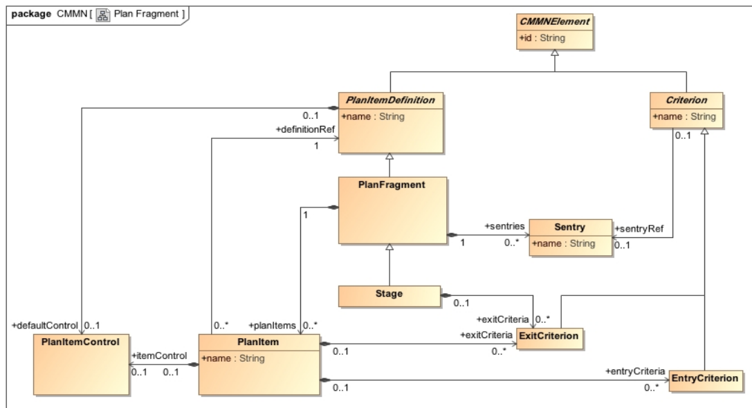
Figure 5.8 - PlanFragment class diagram
