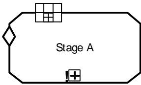
Figure 6.49 - Collapsed Stage with Collapsed PlanningTable
