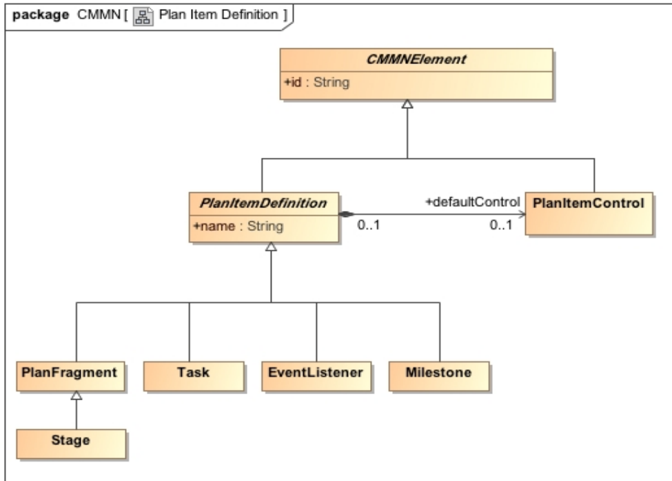
Figure 5.6 - PlanItemDefinition class diagram
