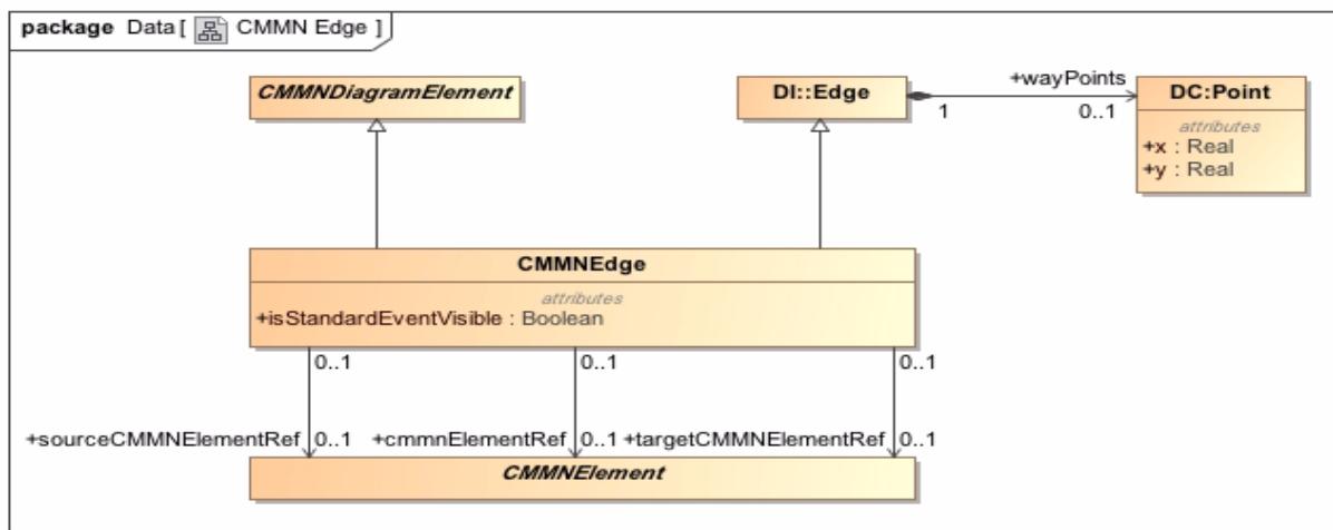
Figure 7.5 - CMMN Edge
