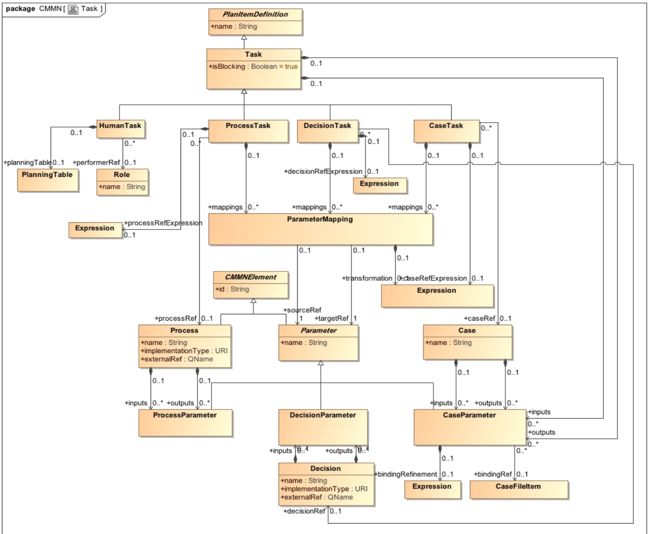
Figure 5.12 - Task class diagram
