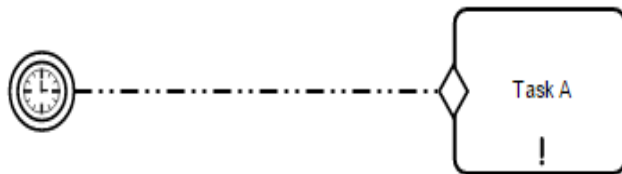
Figure 6.41 - Using the Sentry-based connector to visualize dependency between a Task and a TimerEventListener
