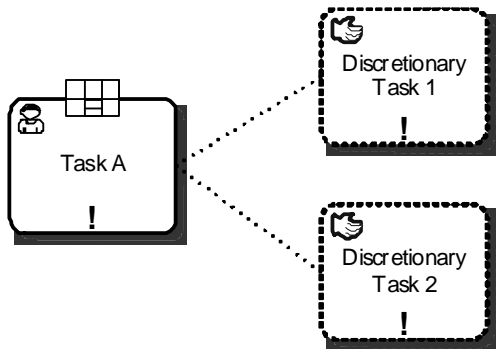
Figure 6.36 - Dependency between a blocking HumanTask and its associated Discretionary Tasks
