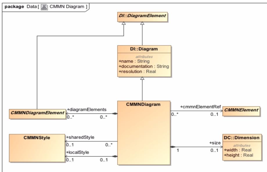
Figure 7.2 - CMMNDiagram
