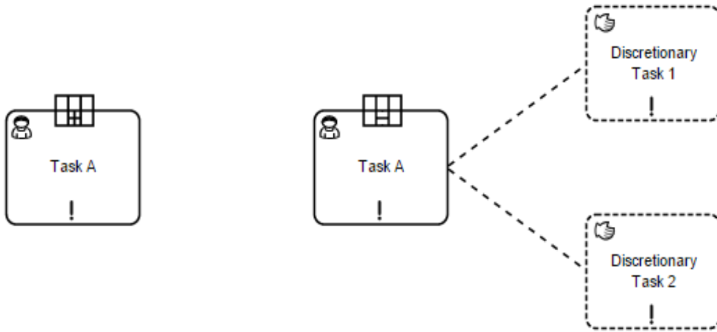
Figure 6.48 - Blocking Human Task with Discretionary Items not expanded and expanded
