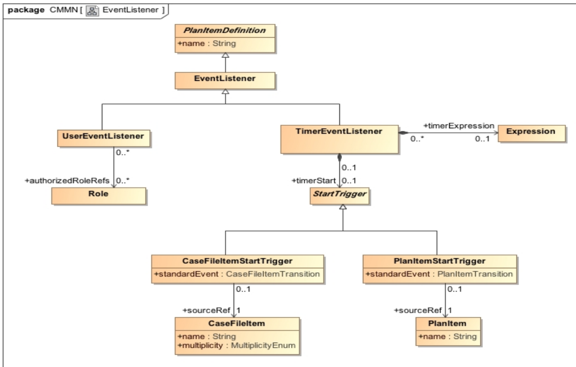
Figure 5.7 - EventListener class diagram
