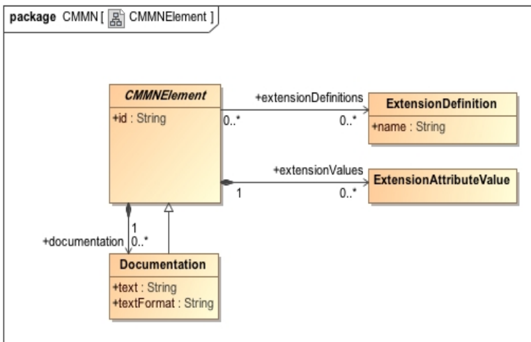
Figure 5.1 - CMMNElement class diagram
