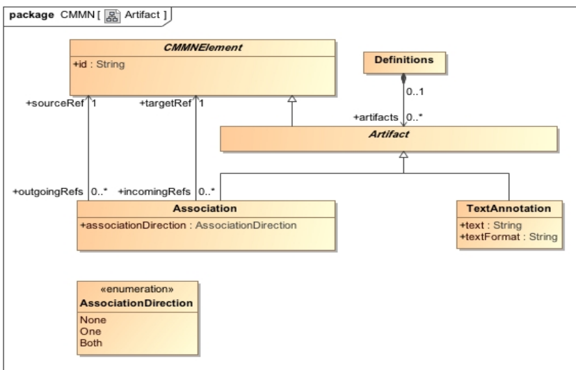
Figure 5.14 - Artifacts class diagram
