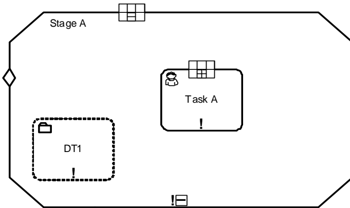
Figure 6.51 - Expanded Stage with Expanded PlanningTable
