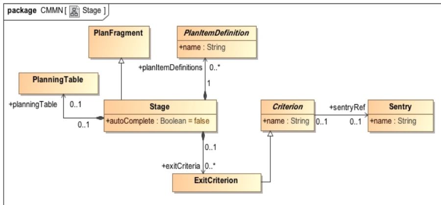
Figure 5.10 - Stage class diagram
