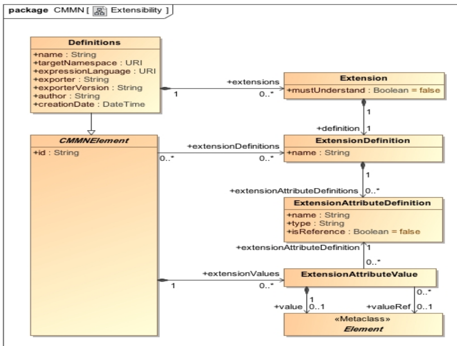
Figure 5.3 - Extensibility diagram
