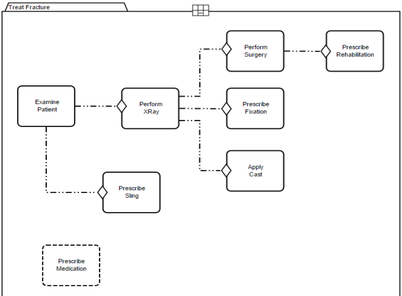
Figure 6.2 - CasePlanModel Example
