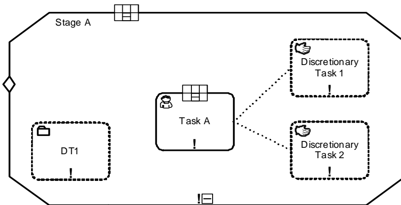
Figure 6.52 - Expanded Stage with Expanded PlanningTable and Expanded HumanTask PlanningTable
