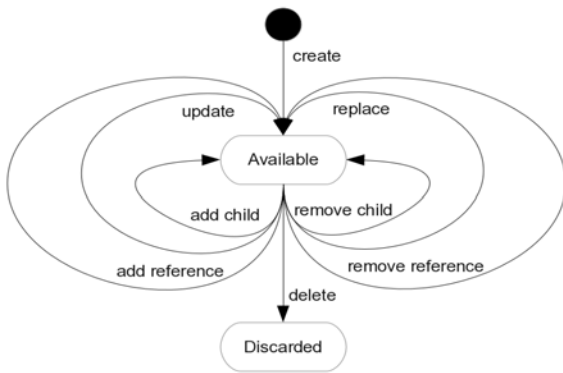
Figure 7.38.3: CaseFileItem instance lifecycle
