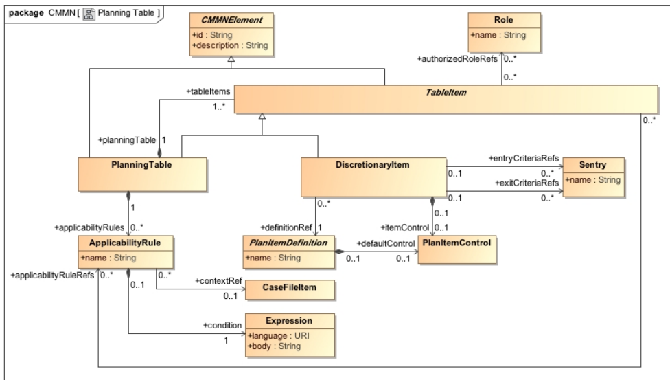
Figure 1040: PlanningTable class diagram
