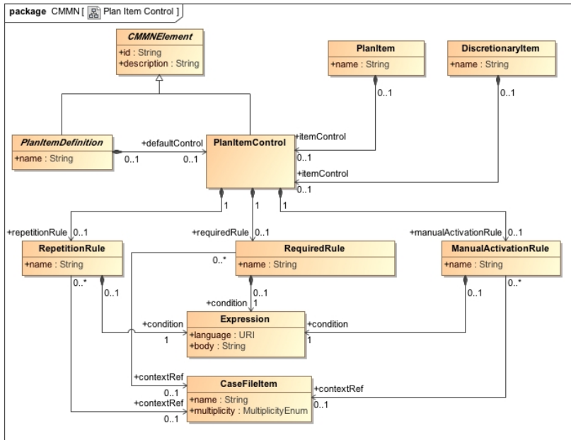
Figure 12: PlanItemControl class diagram
