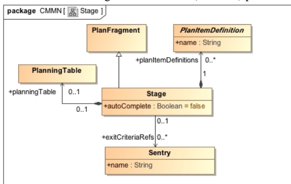
Figure 9: Stage class diagram
