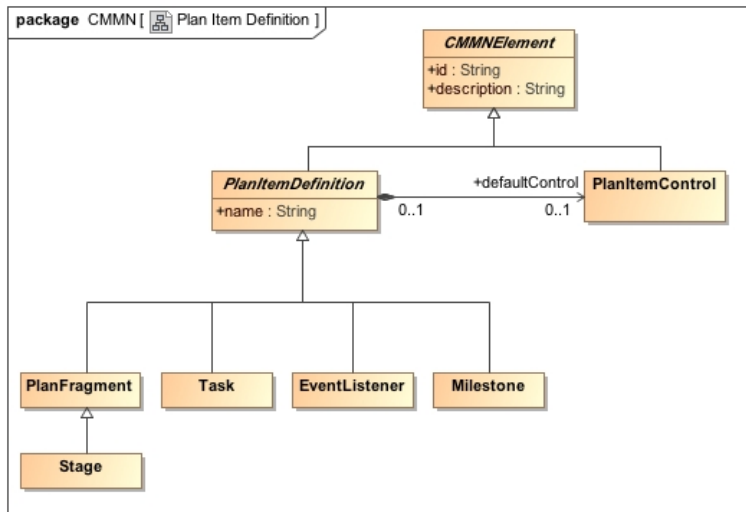
Figure 5: PlanItemDefinition class diagram
