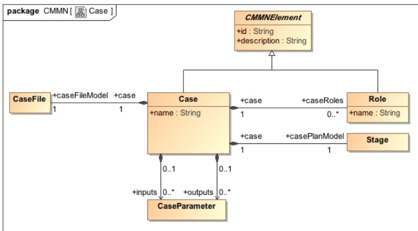
Figure 3: Case class diagram
