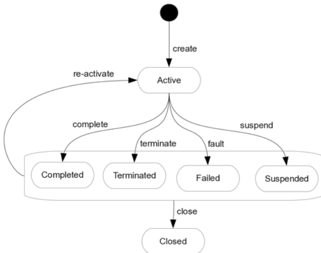
Figure 78787874: Lifecycle of a Case instance
