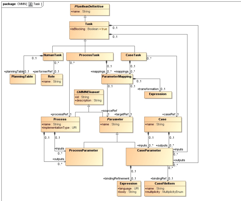
Figure 11: Task class diagram
