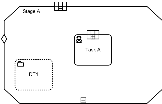
Figure 58585854: Expanded Stage with Expanded PlanningTable
