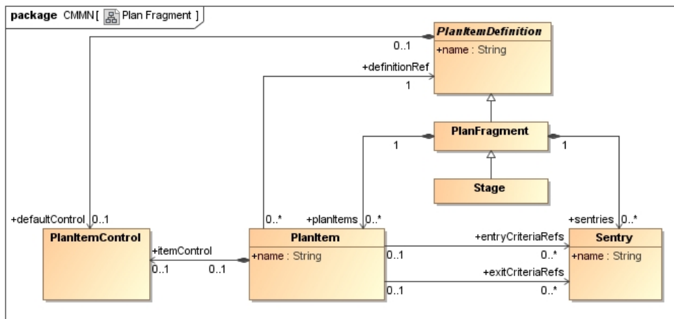
Figure 7: PlanFragment class diagram
