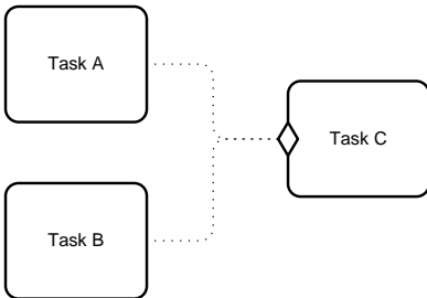
Figure 44444440: Using Sentry-based connectors to visualize "AND"
