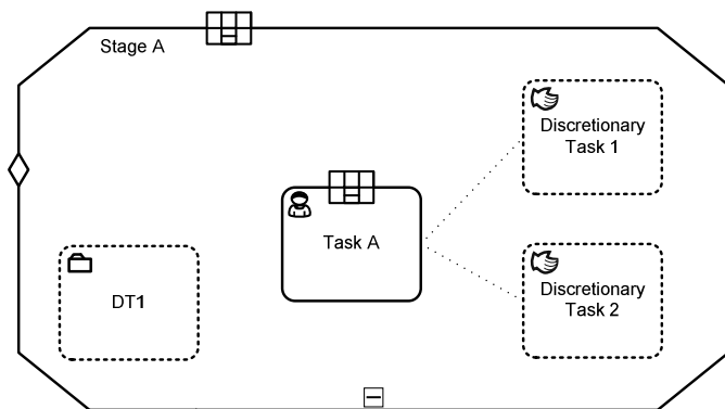
Figure 59595955: Expanded Stage with Expanded PlanningTable and Expanded HumanTask PlanningTable
