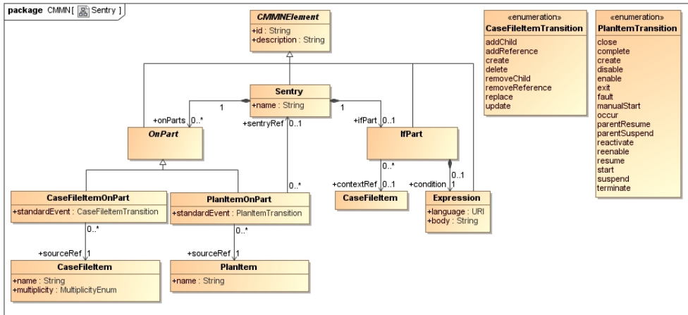
Figure 8: Sentry class diagram
