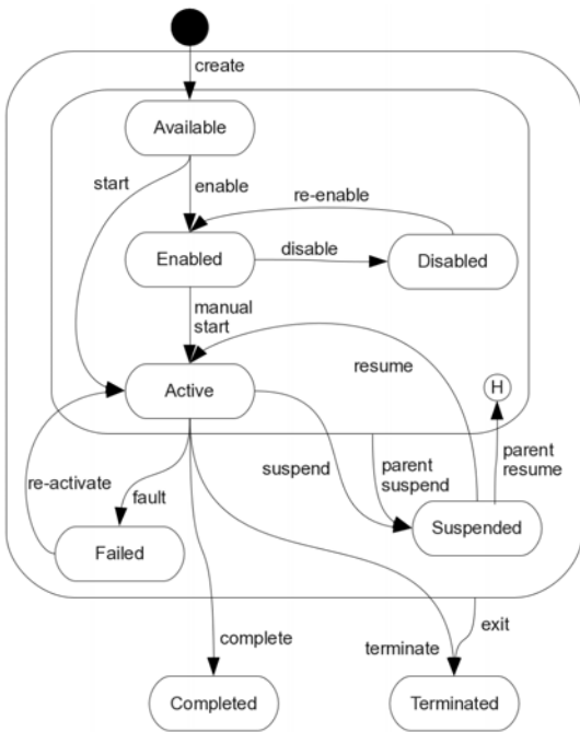
Figure 79797975: Lifecycle of a Stage or Task instance
