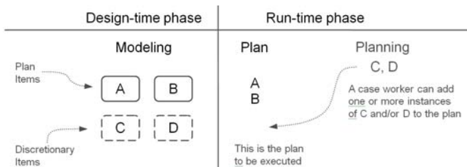
Figure 1: Design-time phase modeling and run-time phase planning
