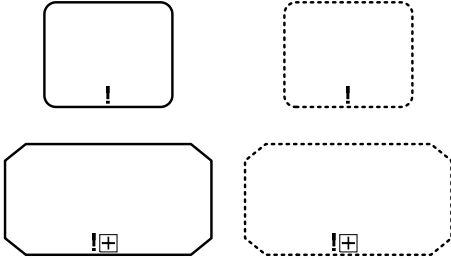
Figure 6666662: Required Decorator example on Task and Stage
