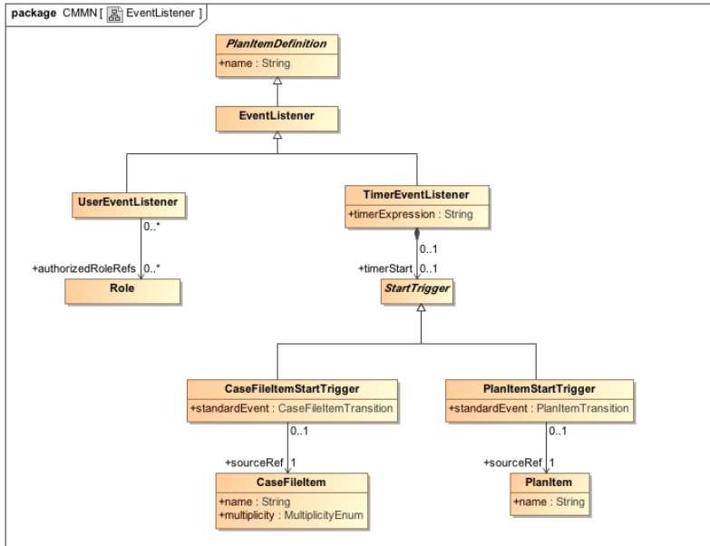
Figure 6: EventListener class diagram
