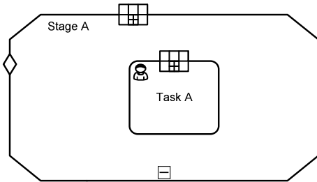
Figure 57575753: Expanded Stage with Collapsed PlanningTable
