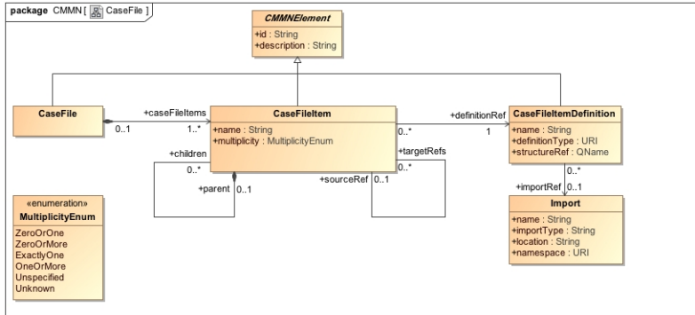
Figure 4: CaseFile class diagram
