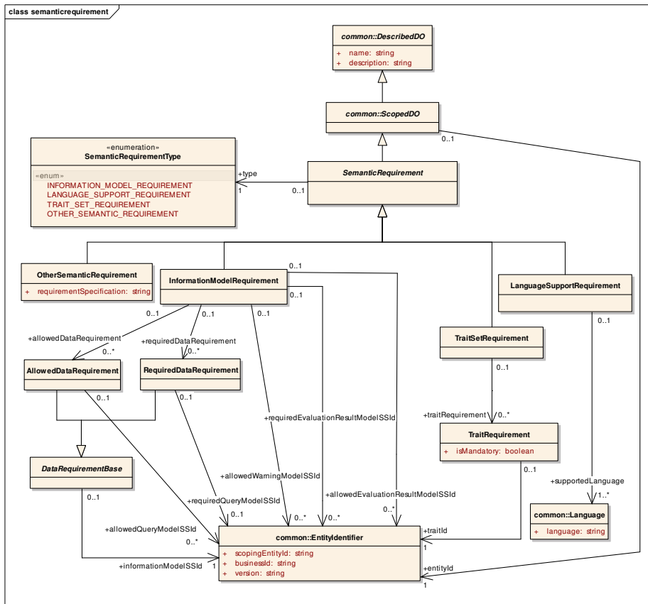
Figure 6.9 - Model for Semantic Requirement
