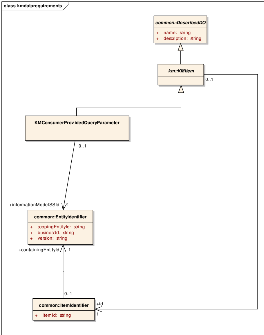
Figure 6.14 - Model for Consumer-Provided Query Parameter
