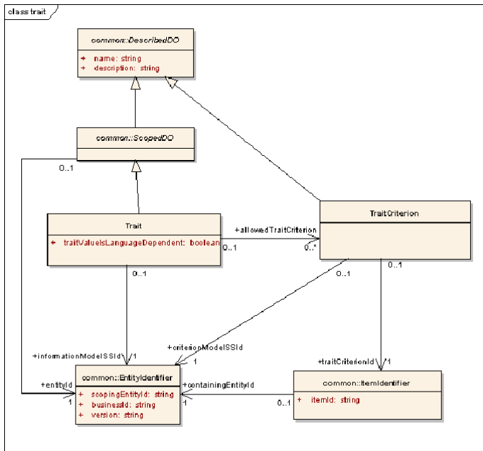
Figure 6.10 - Model for Trait
