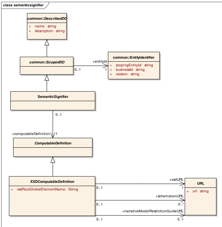
Figure 6.7 - Model for Semantic Signifier
