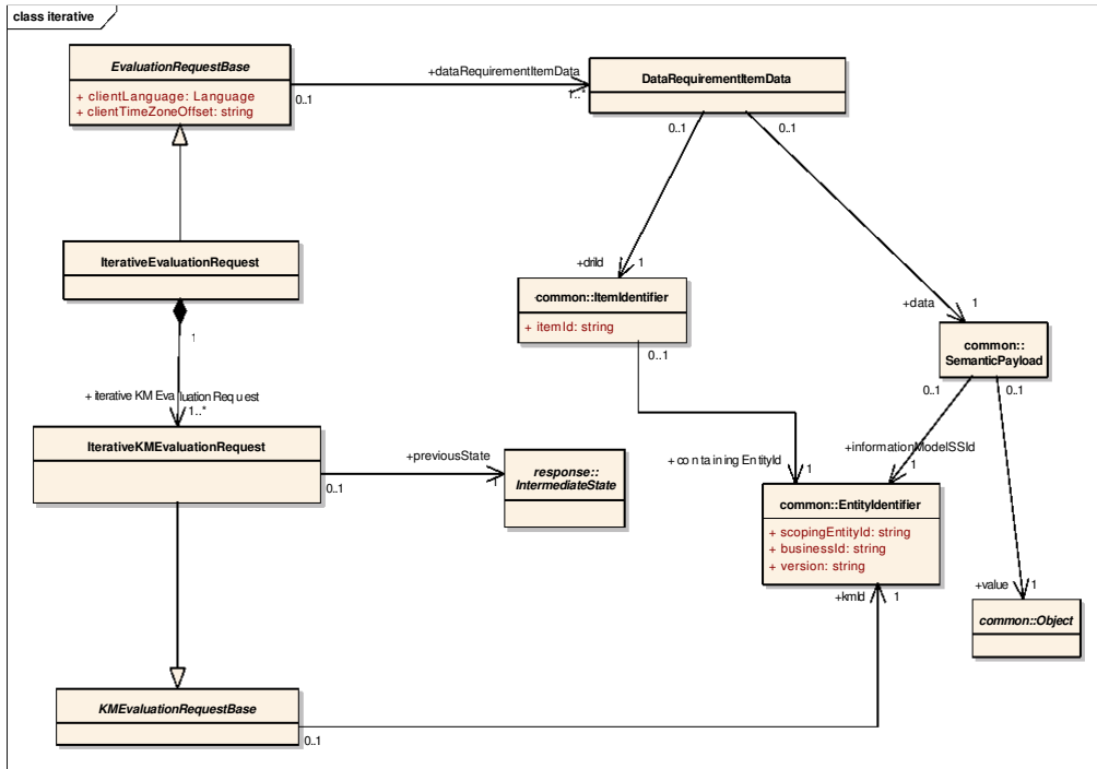
Figure 6.23 - Model for Iterative Evaluation Request
