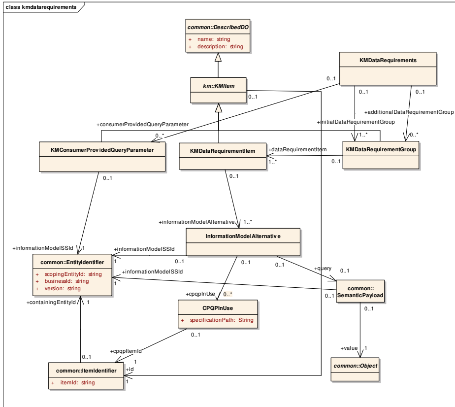
Figure 6.16 - Model for KM Data Requirements
