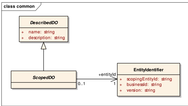
Figure 6.5 - Model for Scoped Data Object
