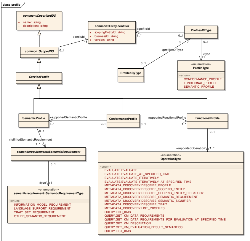
Figure 6.6 - Model for Service Profile
