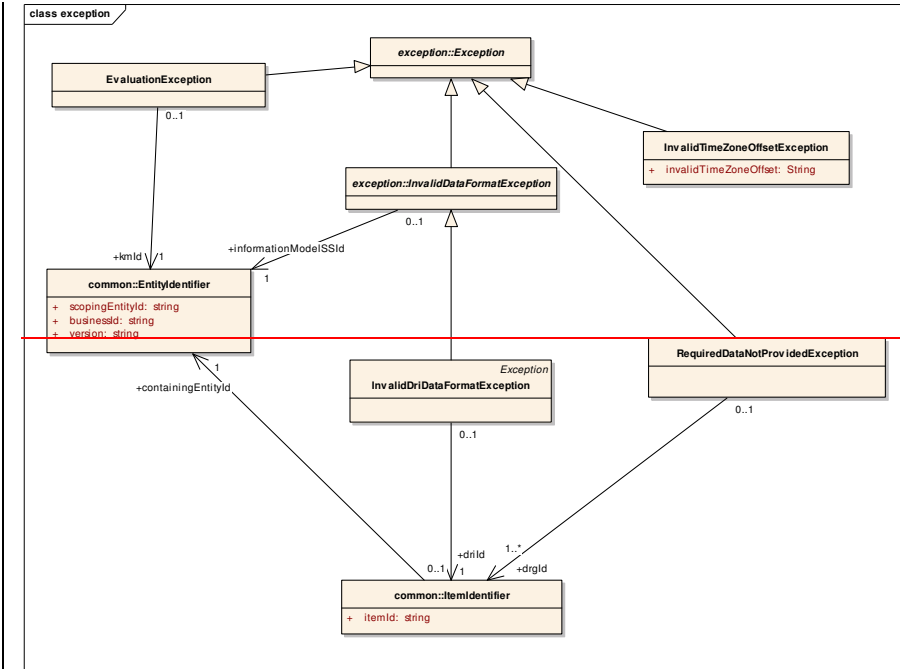
Figure 6.20 - Model for Exceptions in evaluation.exception package
