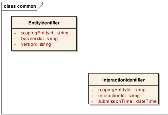
Figure 6.3 - Model for Entity Identifier and Interaction Identifier
