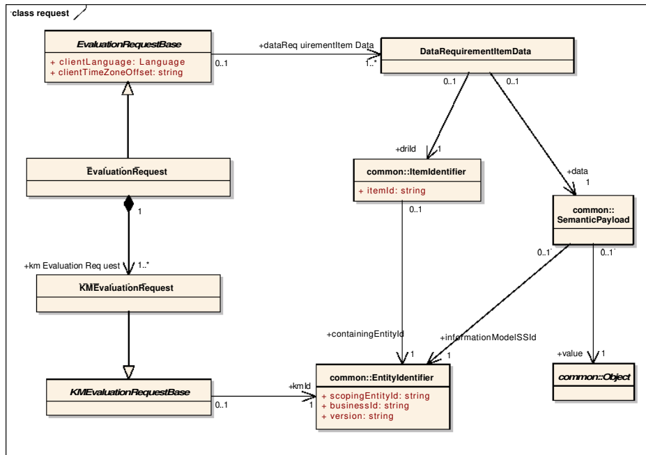
Figure 6.22 - Model for Evaluation Request
