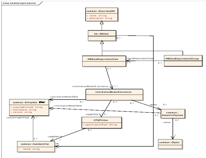
Figure 6.15 - Model for KM Data Requirement Group
