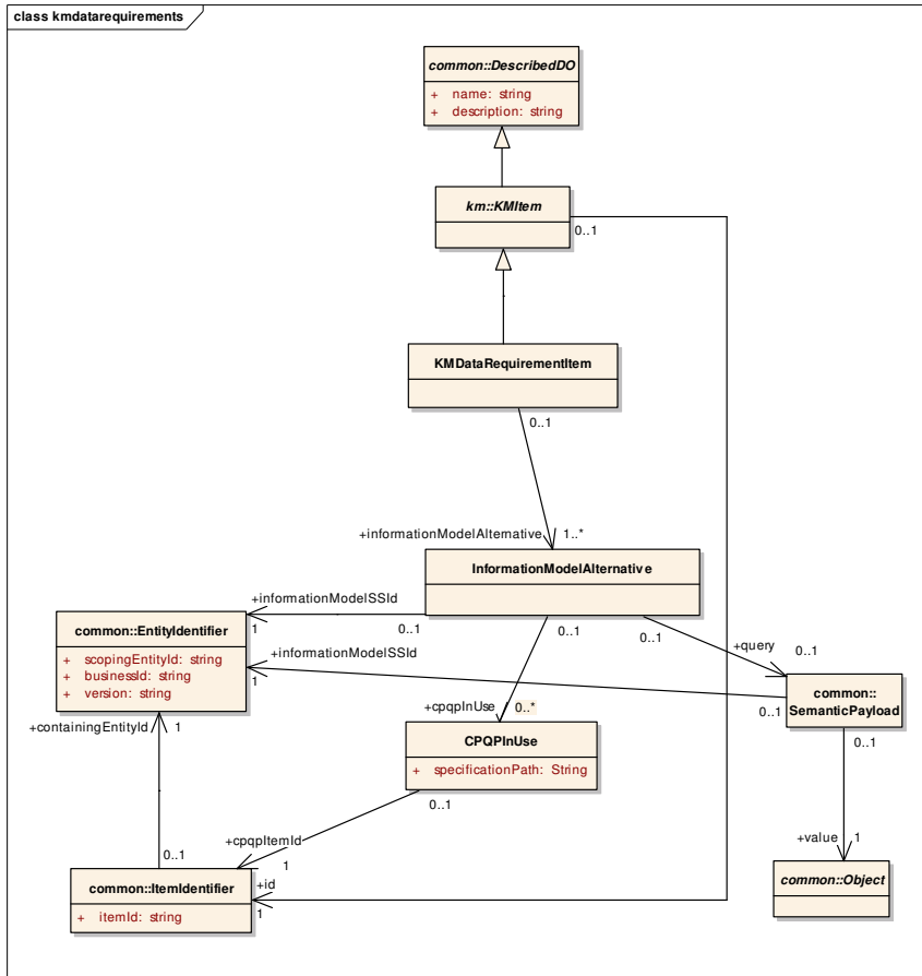
Figure 6.13 - Model for KM Data Requirement Item
