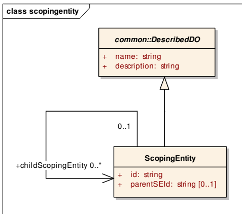
Figure 6.2 - Model for Scoping Entity
