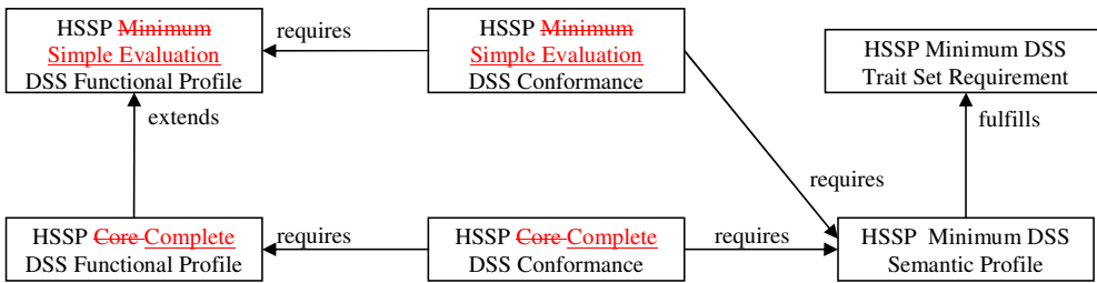
Figure 6.26 - Relationships between profiles
