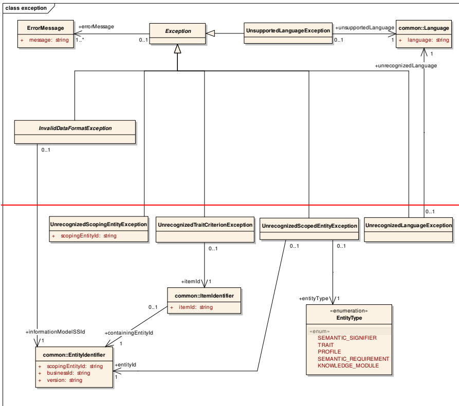
Figure 6.18 - Model for Exceptions in common.exception package
