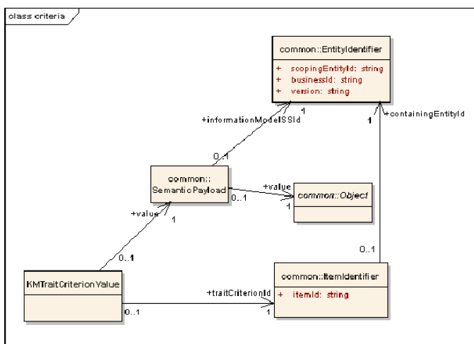
Figure 6.12 - Model for Trait Criterion
