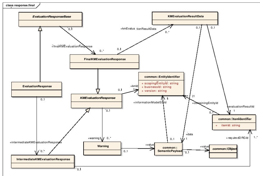
Figure 6.24 - Model for Evaluation Response
