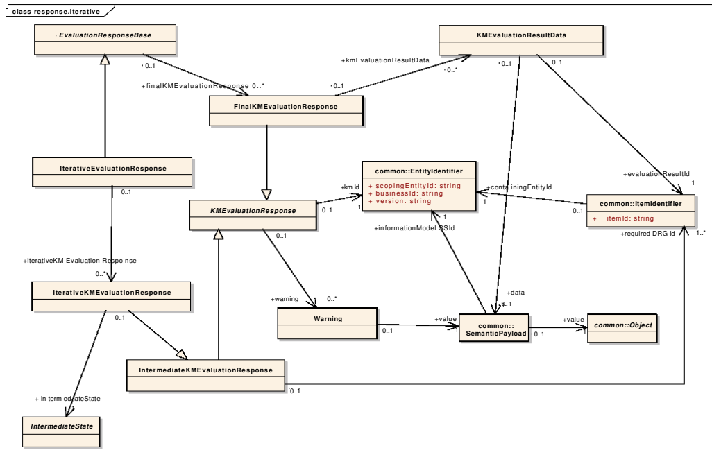
Figure 6.25 - Model for Iterative Evaluation Response
