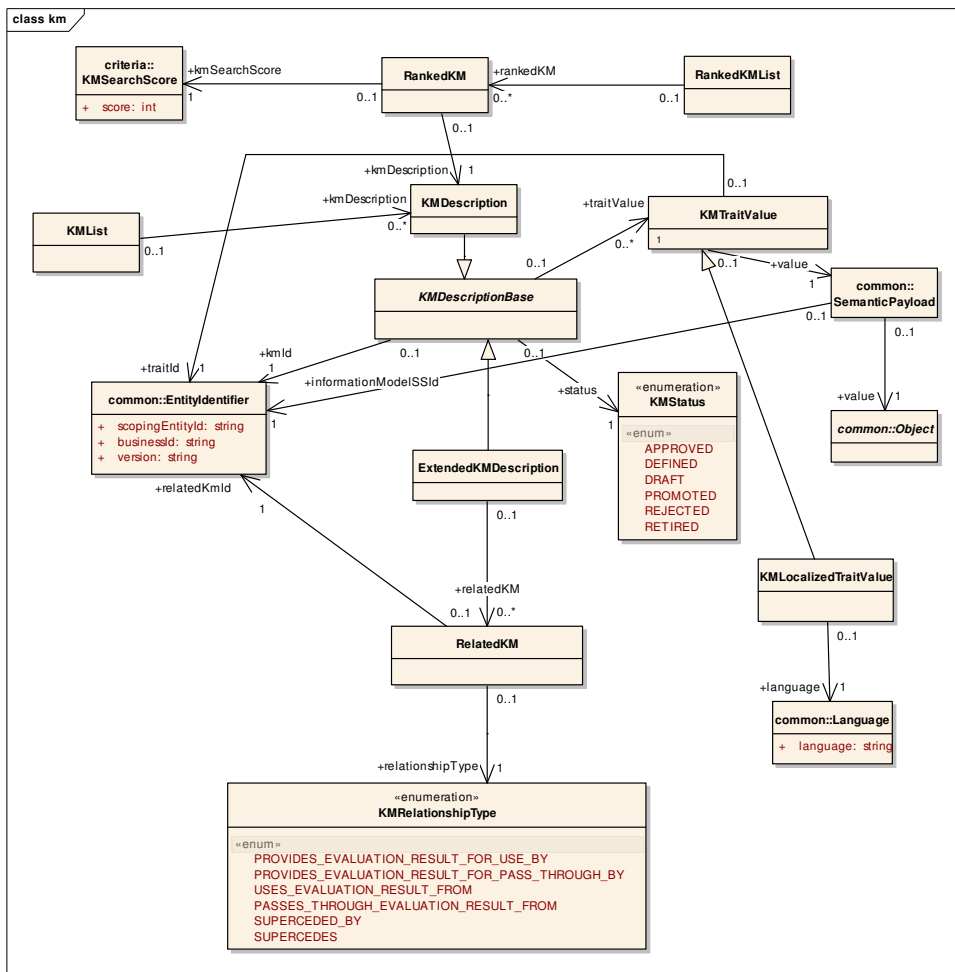
Figure 6.8 - Model for Knowledge Module Description
