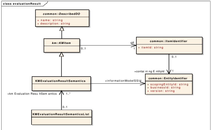
Figure 6.17 - Model for KM Evaluation Result Semantics
