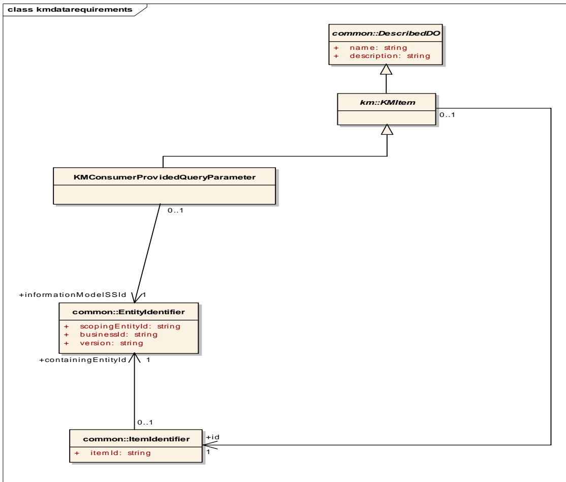
Figure 6.14 - Model for Consumer-Provided Query Parameter
