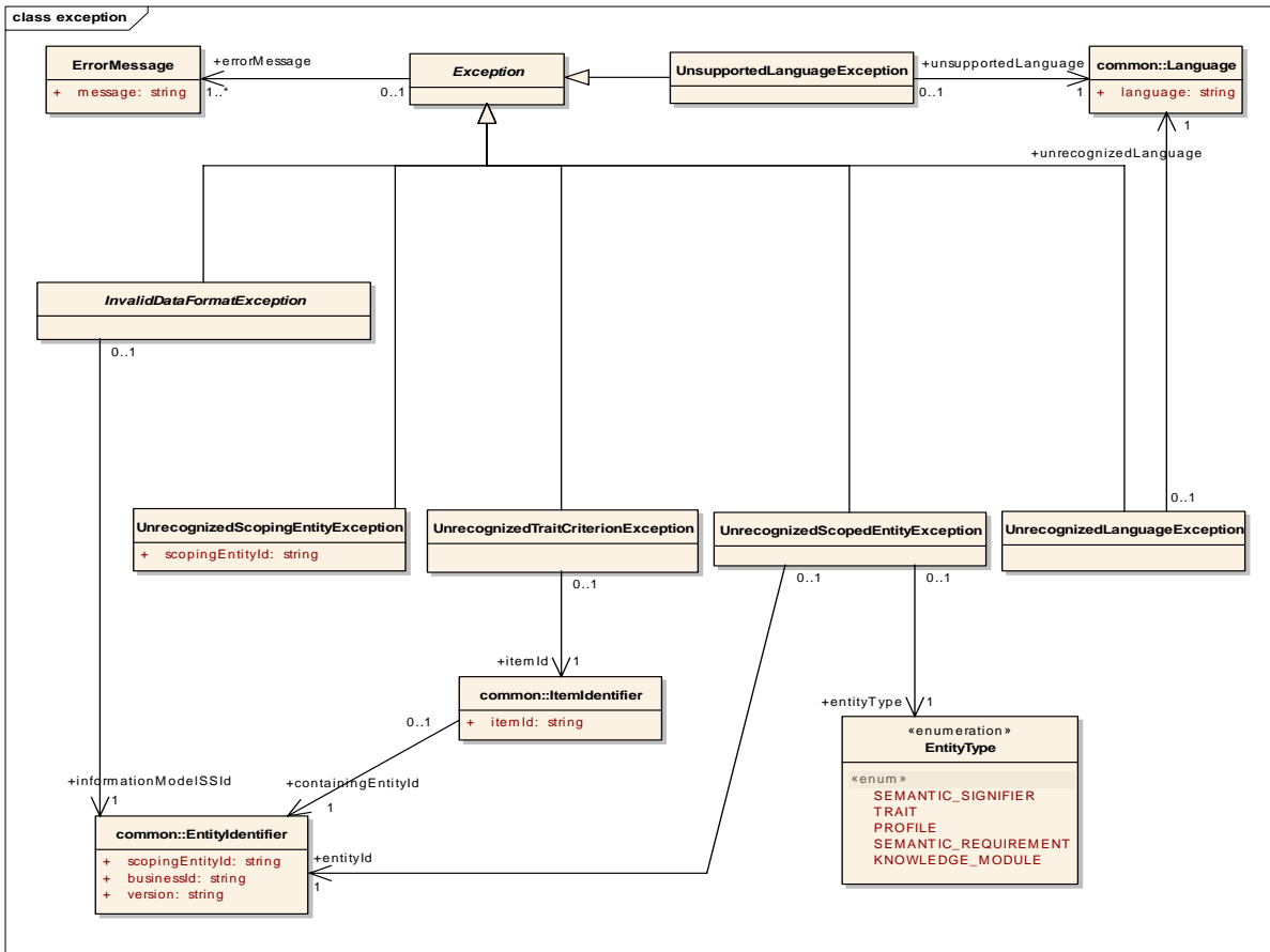
Figure 6.18 - Model for Exceptions in common.exception package
