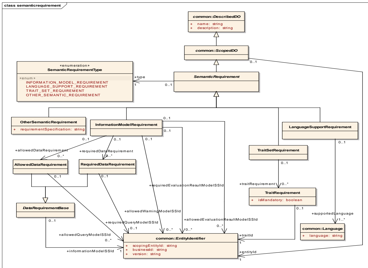
Figure 6.9 - Model for Semantic Requirement
