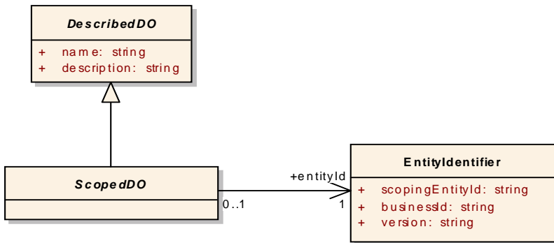
Figure 6.5 - Model for Scoped Data Object
