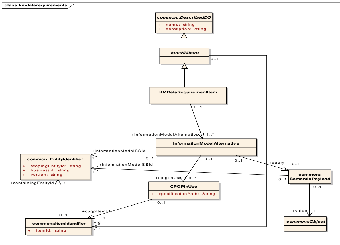
Figure 6.13 - Model for KM Data Requirement Item
