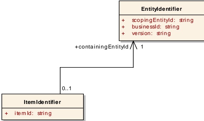
Figure 6.4 - Model for Item Identifier
