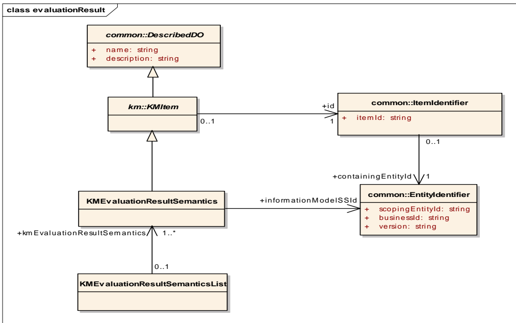
Figure 6.17 - Model for KM Evaluation Result Semantics
