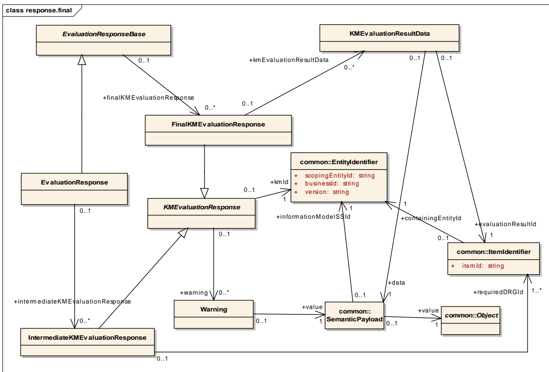
Figure 6.24 - Model for Evaluation Response
