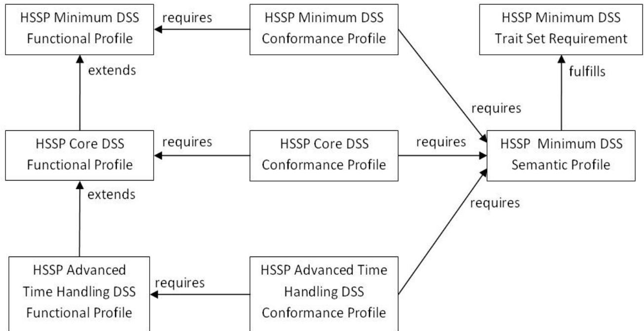
Figure 6.26 - Relationships between profiles
