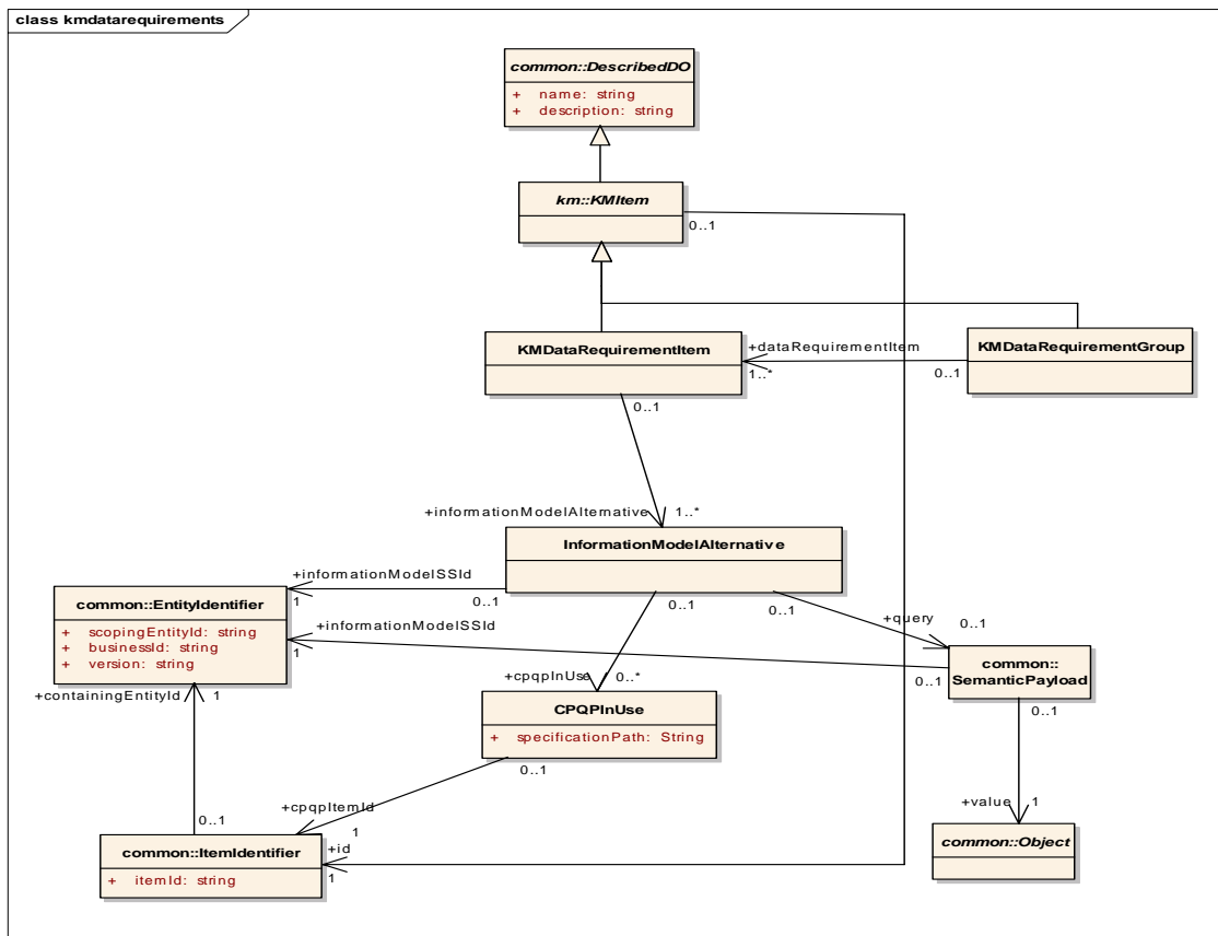
Figure 6.15 - Model for KM Data Requirement Group
