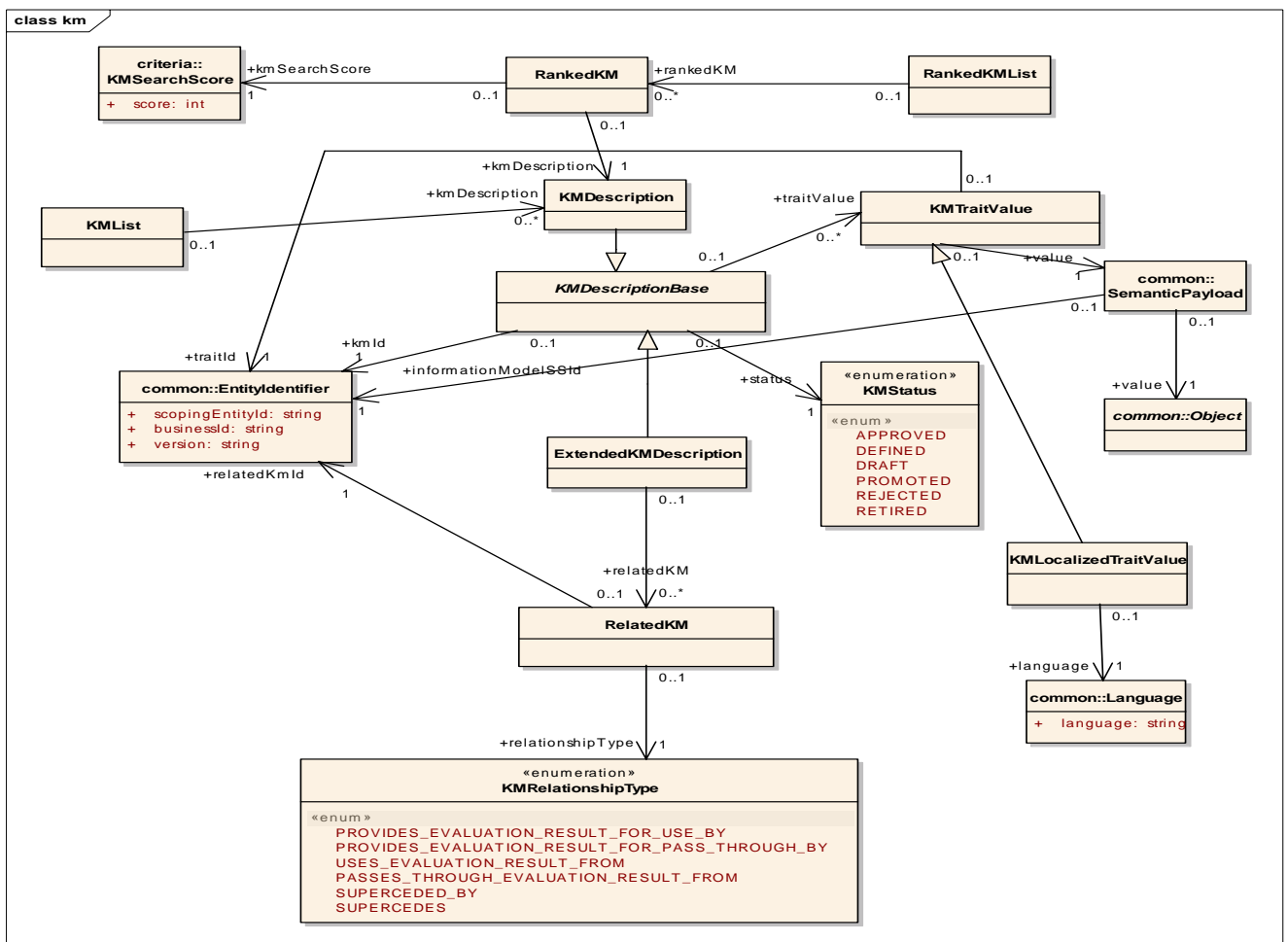
Figure 6.8 - Model for Knowledge Module Description
