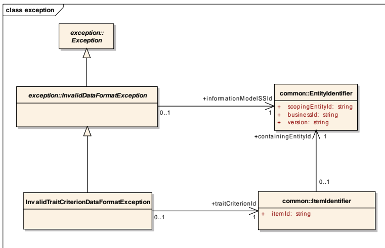
Figure 6.19 - Model for Exceptions in query.exception package
