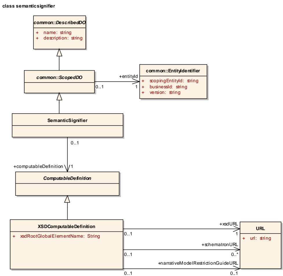
Figure 6.7 - Model for Semantic Signifier
