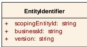
Figure 6.3 - Model for Entity Identifier
