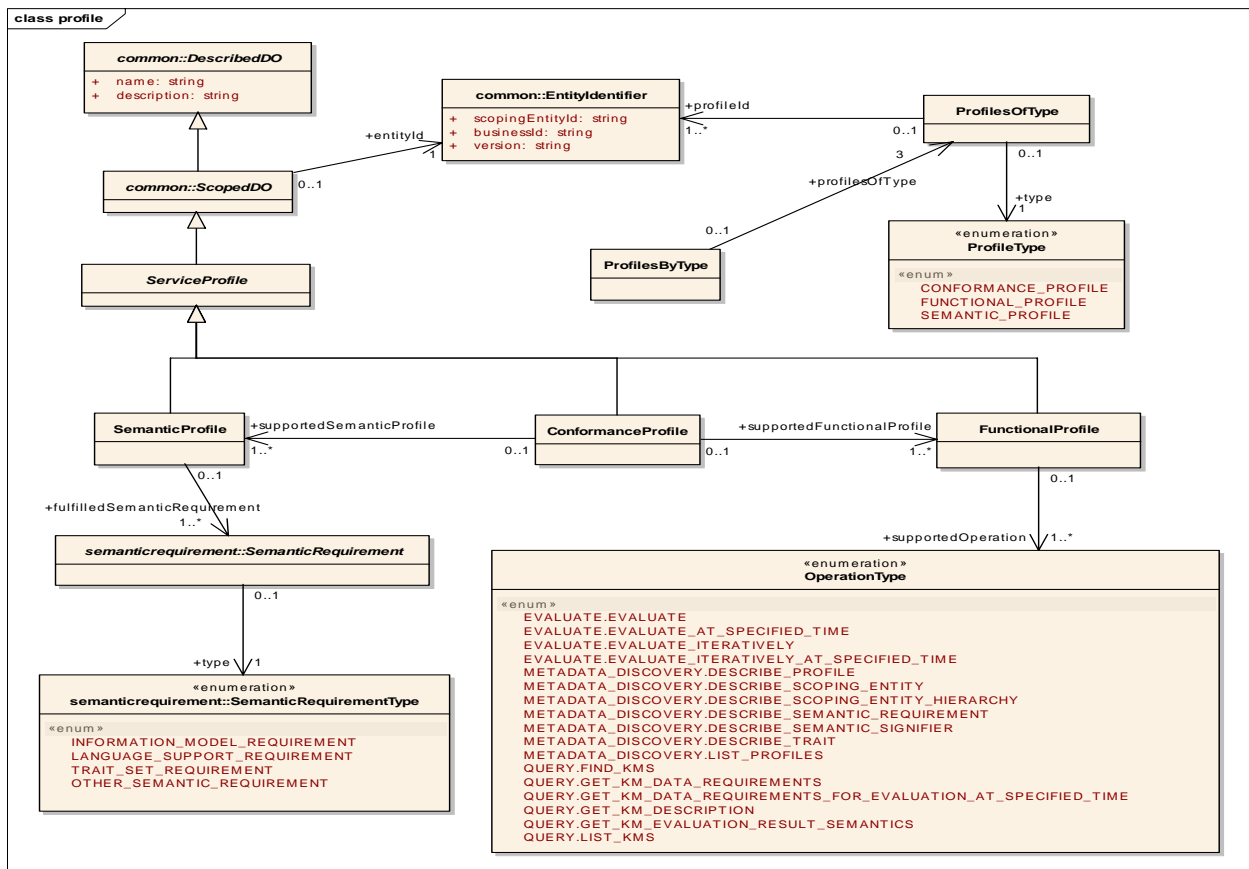
Figure 6.6 - Model for Service Profile
