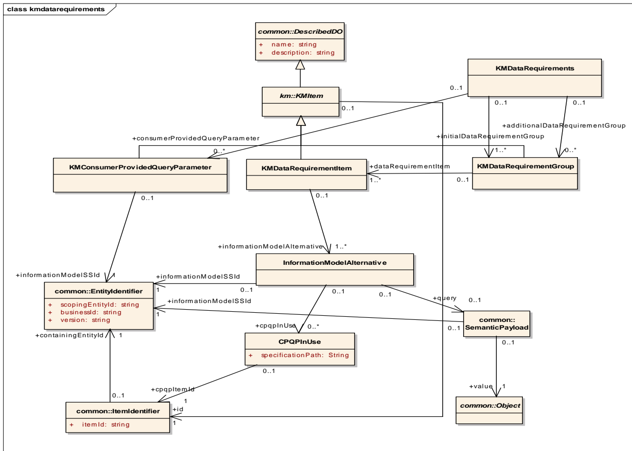
Figure 6.16 - Model for KM Data Requirements
