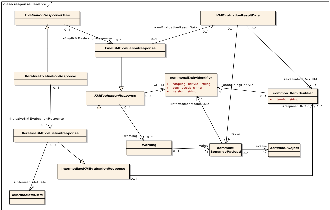
Figure 6.25 - Model for Iterative Evaluation Response
