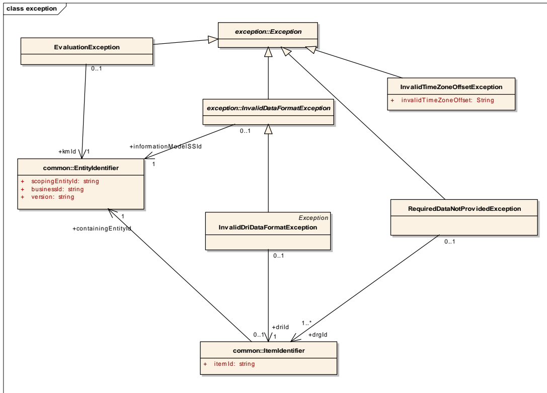
Figure 6.20 - Model for Exceptions in evaluation.exception package
