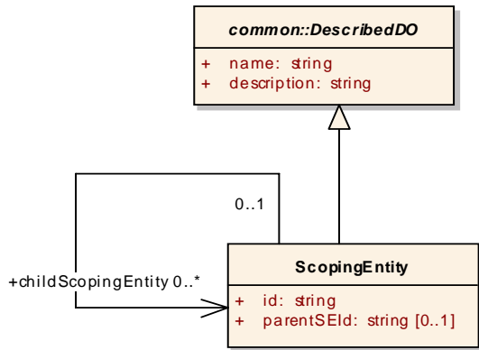
Figure 6.2 - Model for Scoping Entity
