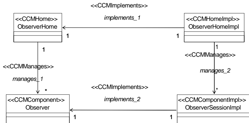
Figure 36 - The Composition model for the Observer component
