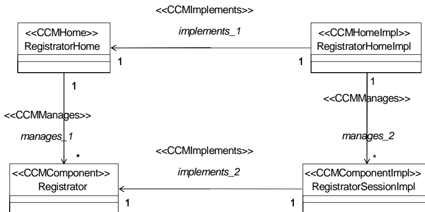
Figure 35 - The Composition model for the Registrator component
