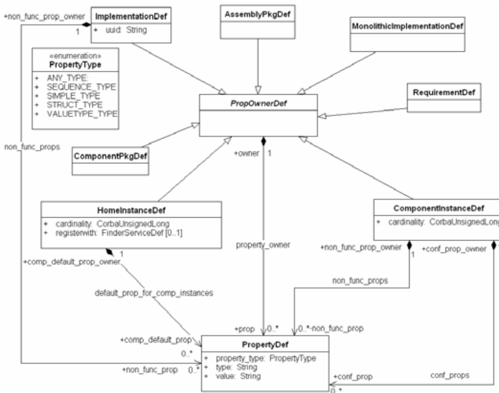
Figure 7.13 - Properties description
