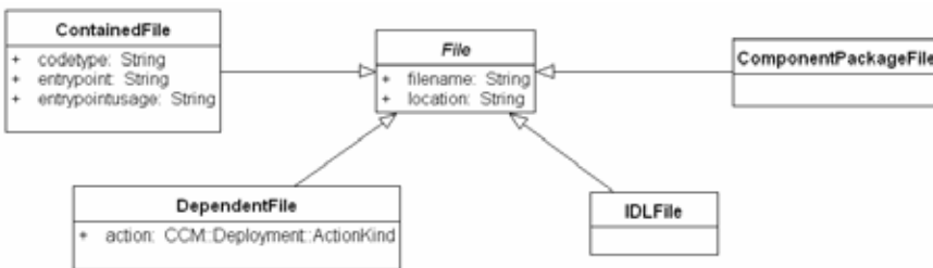
Figure 7.14 - File description
