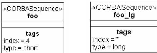
Figure 8.14 - CORBASequence example
