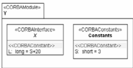
Figure 8.6 - Constant example
