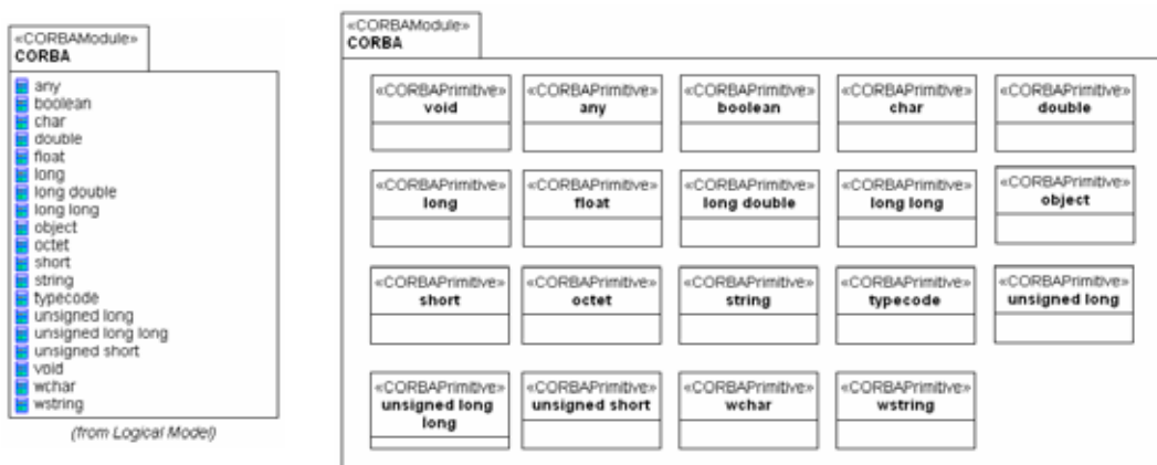
Figure 8.8 - CORBA package
