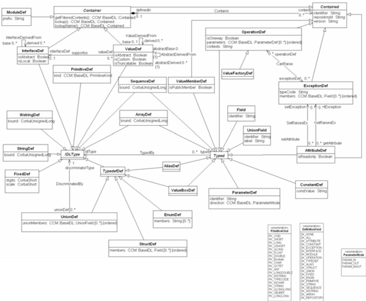
Figure 7.2 - BaseIDL Metamodel
