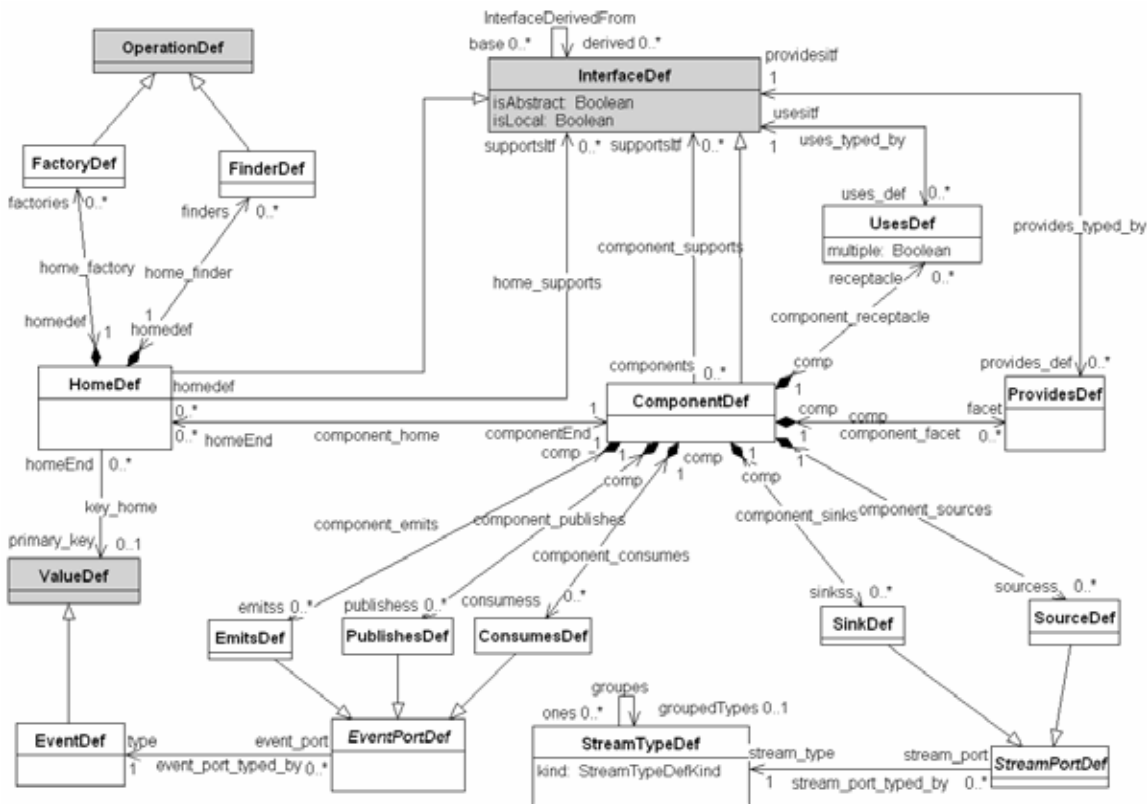
Figure 7.4 - ComponentIDL Metamodel
