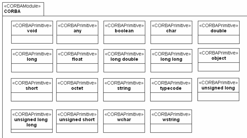
Figure 9.1 - CORBA Package
