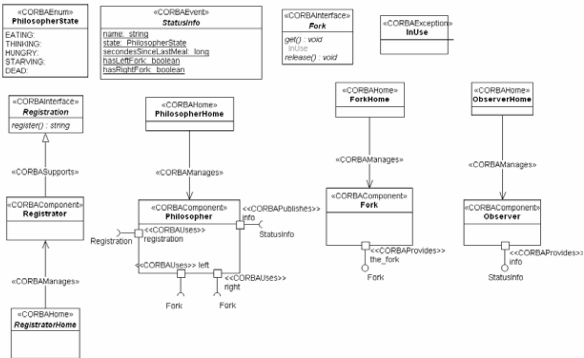
Figure 8.24 - ComponentIDL Profile example
