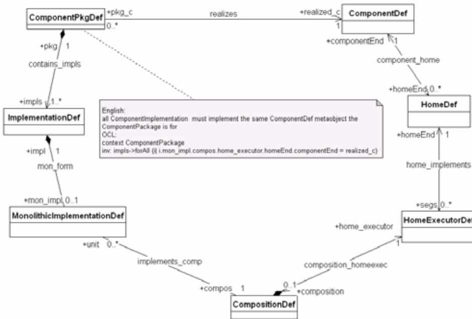
Figure 7.10 - Component package and Implementations
