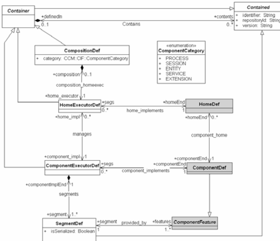
Figure 7.8 - Component Implementation Framework Metamodel
