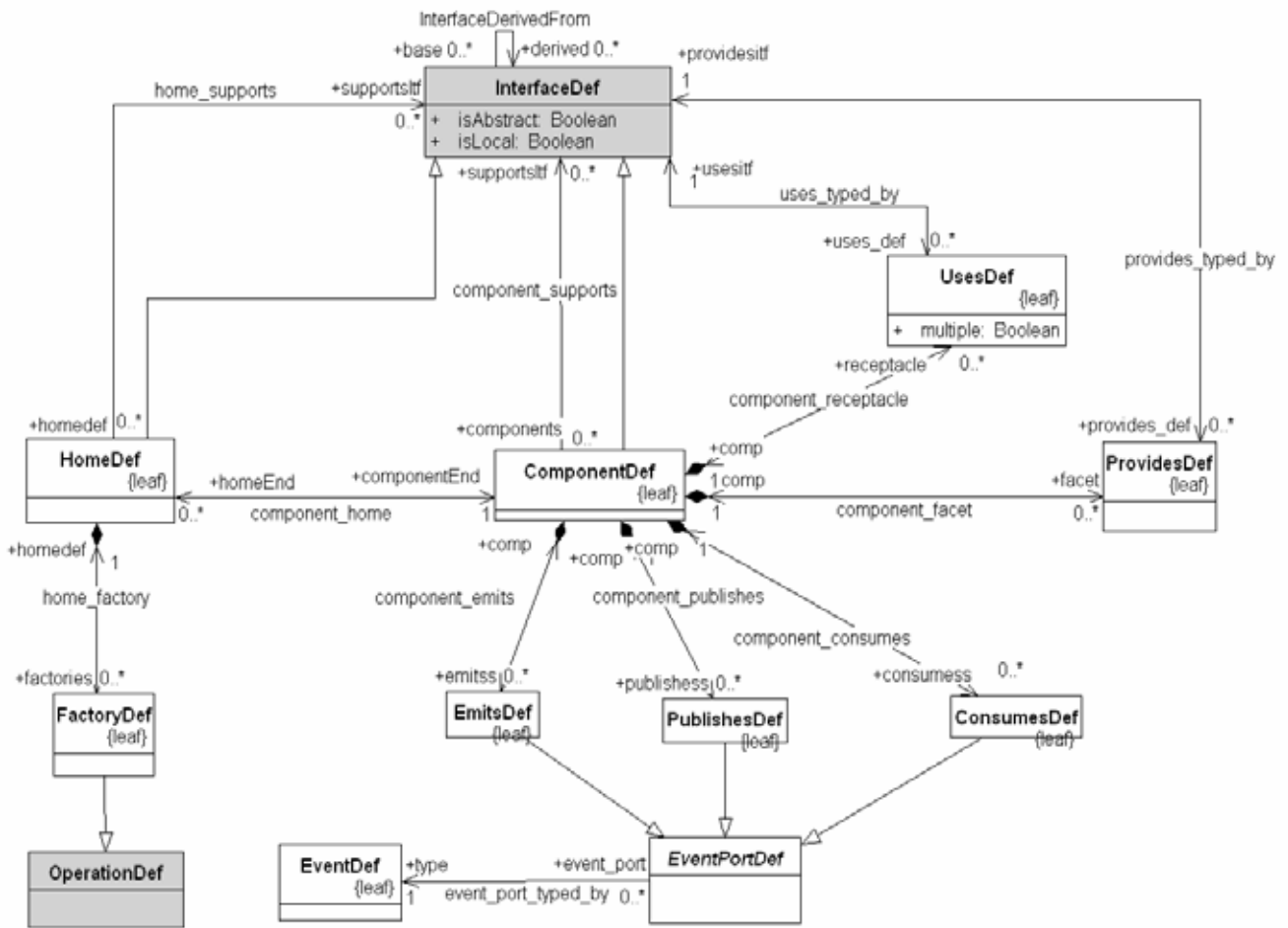
Figure 8.32 - ComponentIDL metamodel for the Lightweight CCM
