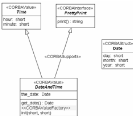
Figure 8.5 - Valuetype example
