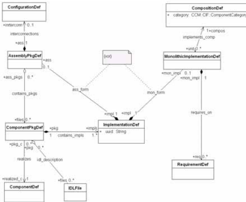
Figure 7.11 - ImplementationDef description
