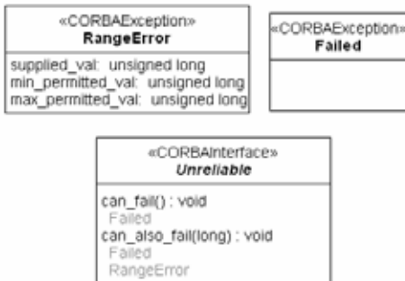
Figure 8.13 - Exception example
