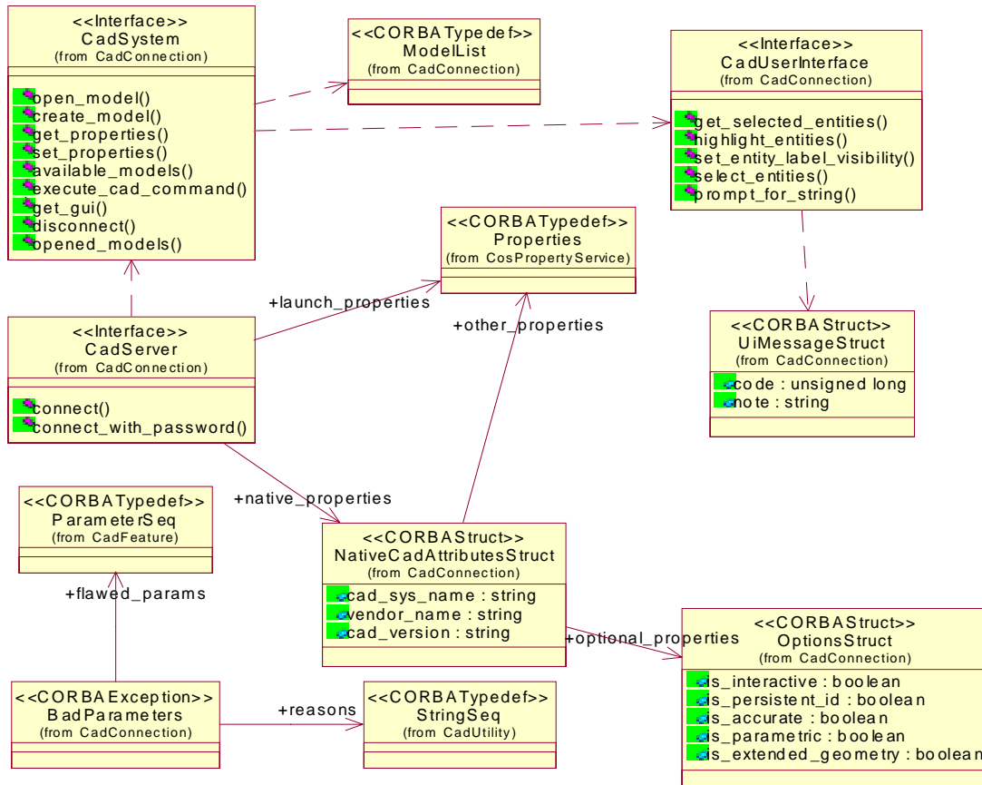
Figure 2-1 UML Diagram of the CadConnection Interfaces and Data Structures
