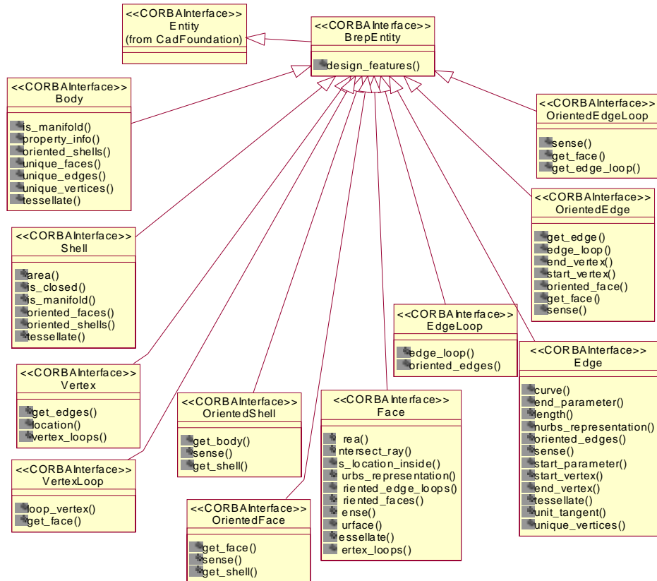
Figure 2-5 UML Diagram of CadBrep Module Interfaces
