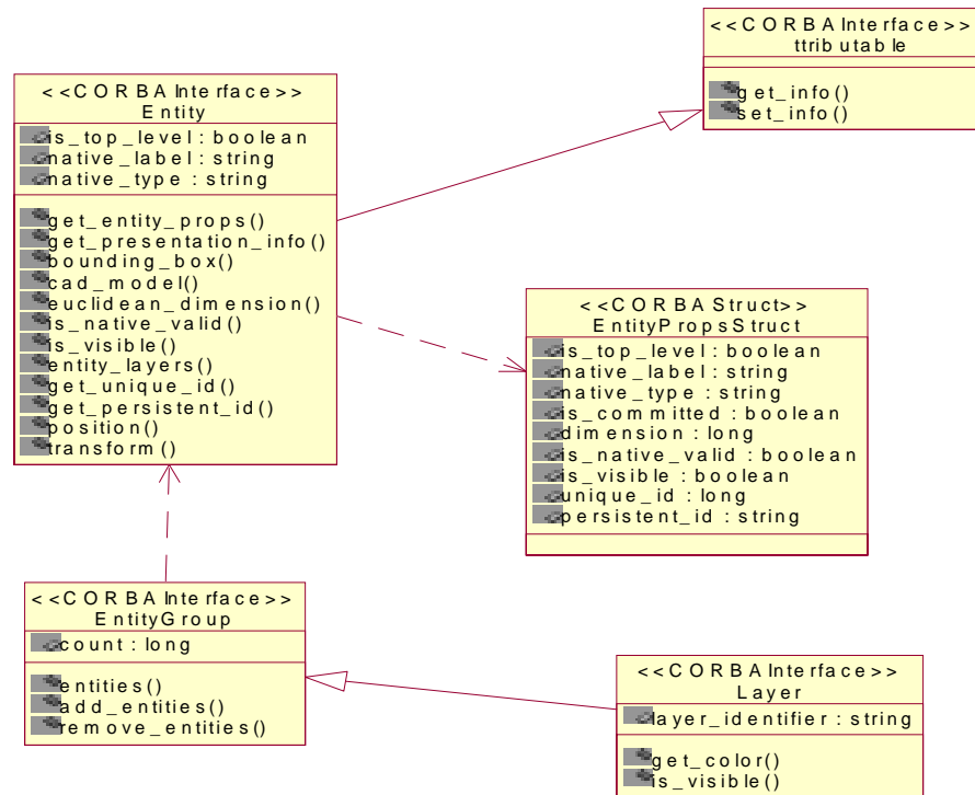
Figure 2-3 UML Diagram of CadFoundation Module
