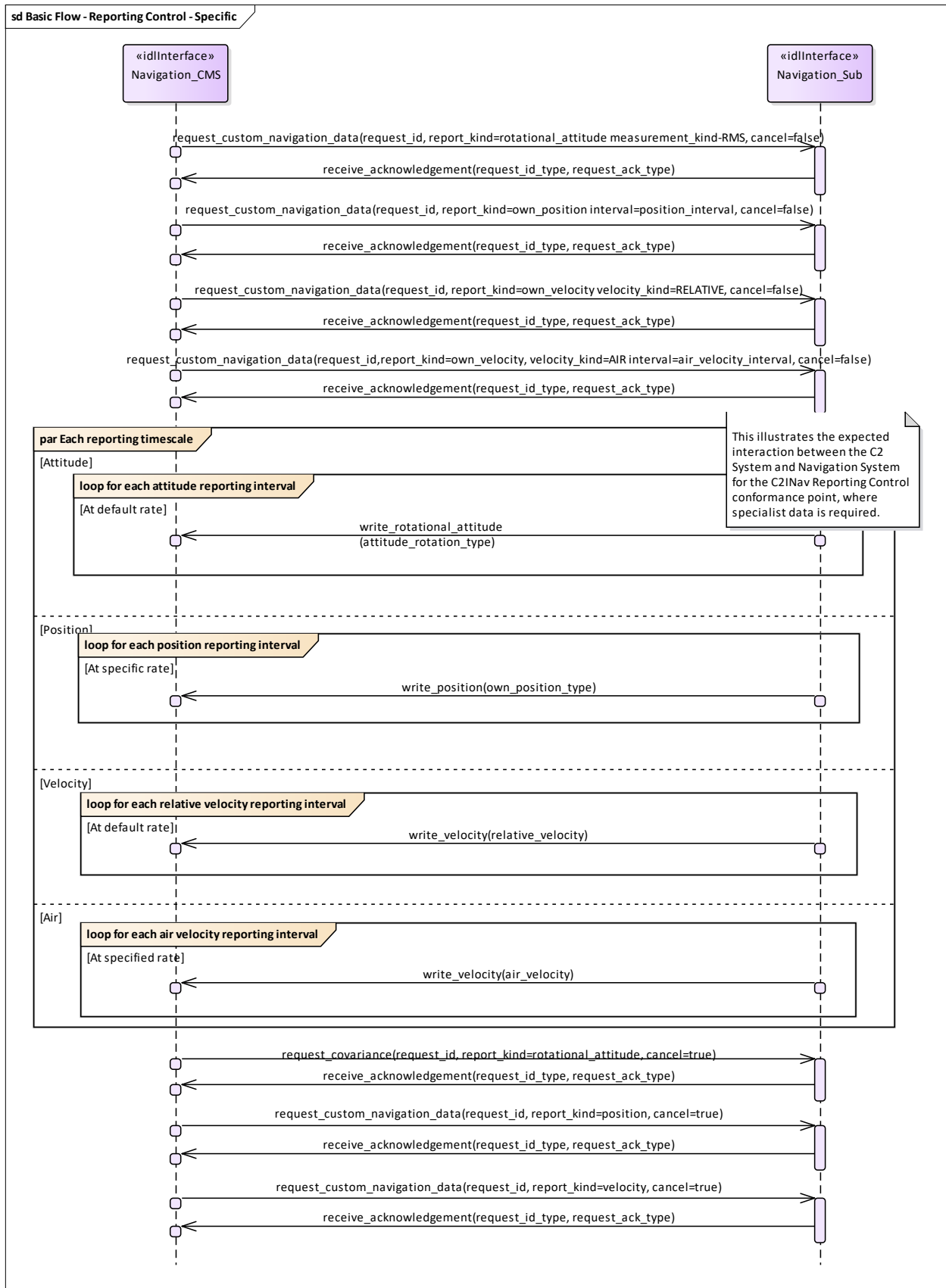
Figure 7-13: Basic Flow - Reporting Control - Specific (Sequence diagram)
