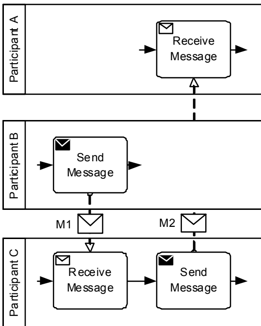
Figure 11.20 - A Collaboration view of an expanded Sub-Choreography
