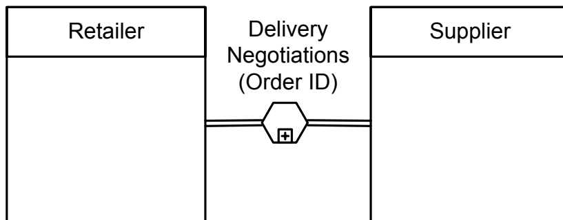
Figure 9.19 - An example of a Sub-Conversation
