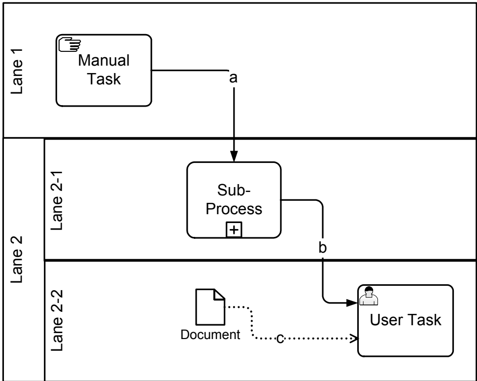
Figure 12.12 - Nested Lanes Example
