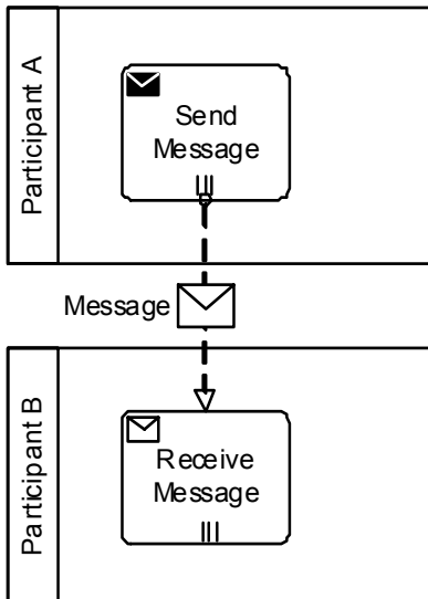
Figure 11.14 - The Collaboration view of a Parallel Multi-Instance Choreography Task
