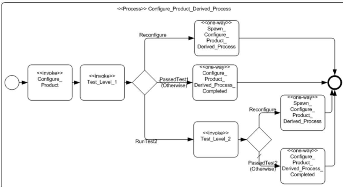
Figure 14.6 - An example of a WSBPEL pattern for the derived Process
