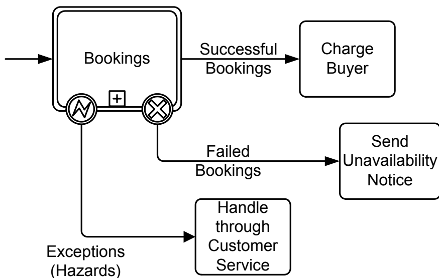
Figure 10.34 - A Collapsed Transaction Sub-Process
