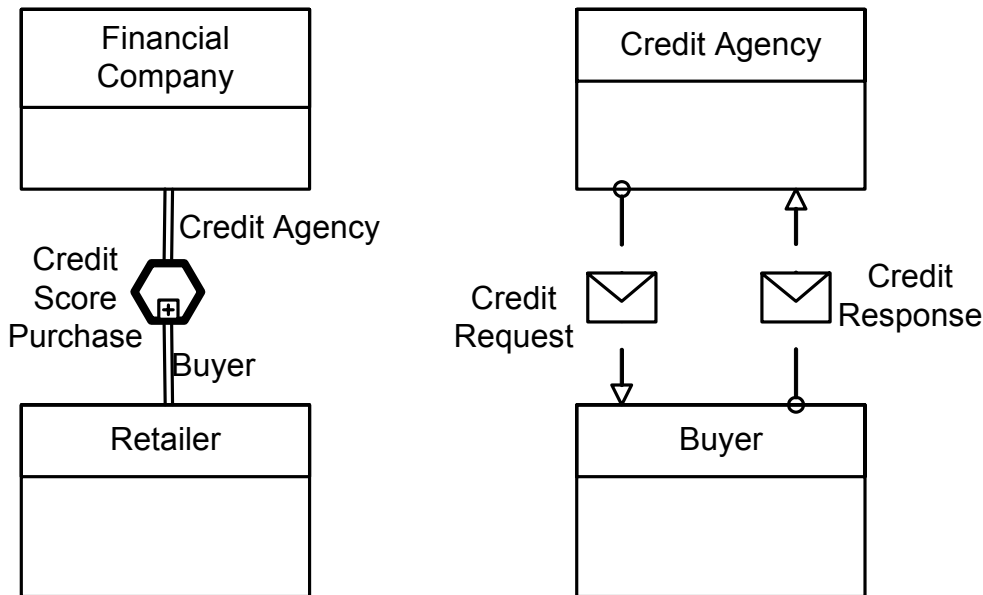
Figure 9.30 – Call Conversation Links
