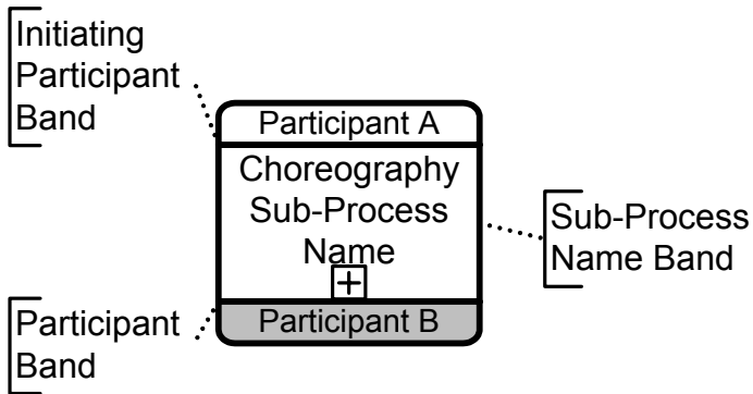
Figure 11.17- A Sub-Choreography
