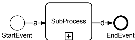
Figure 12.10 - Collapsed Sub-Process
