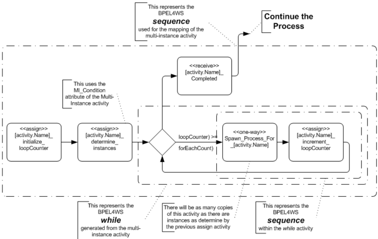
Figure A.5 - BPEL4WS Pattern of Parallel Multi-instance, ML_FlowCondition = One
