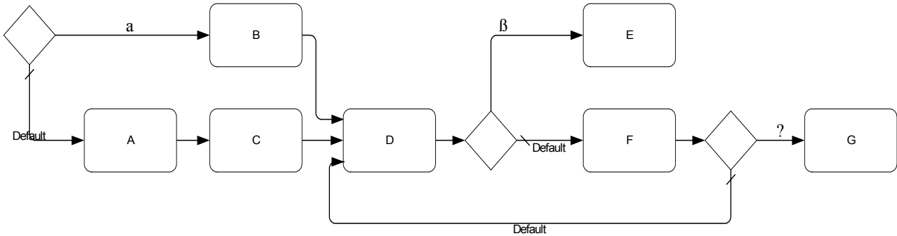
Figure 10.39 - Workflow Pattern #16 -- Arbitrary Cycle
