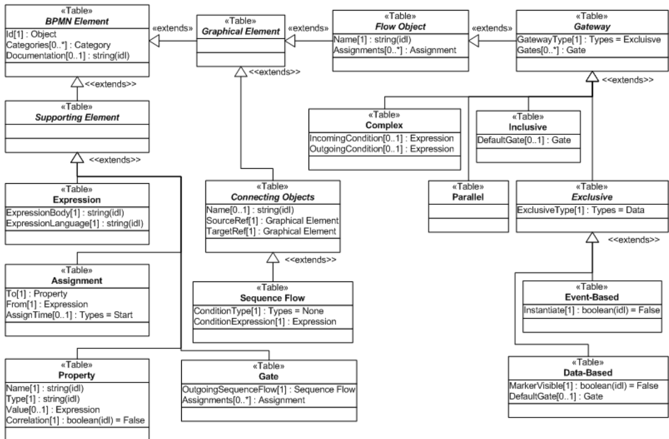
Figure B.4 - BPMN Gateway Elements and Attributes
