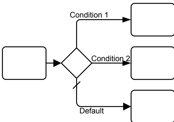
Figure 10.24 - A Data-Based Decision Example -- Workflow Pattern #4 -- Exclusive Choice ["Default Condition" changed to "Default" in figure: Issue 11241, item b]
