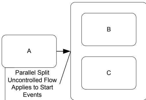
Figure 10.20 - Workflow Pattern #2: Parallel Split -- Version 3
