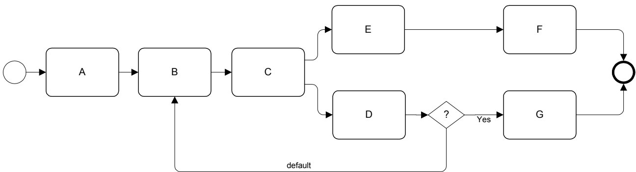
Figure 10.50 - Improper Looping
