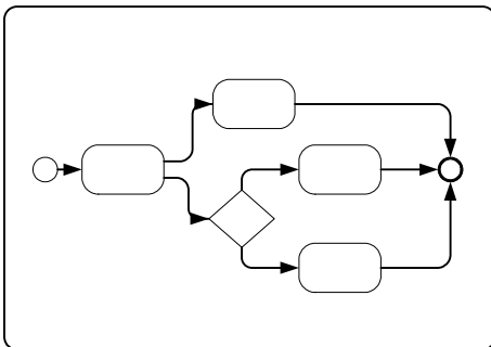
Figure 9.7 - Expanded Sub-Process
