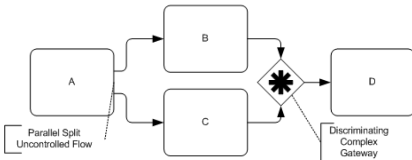
Figure 10.32 - Workflow Pattern #8 -- Discriminator
