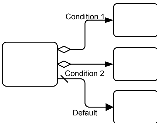
Figure 9.25 - An Inclusive Decision using Conditional Sequence Flow ["Default Condition" changed to "Default" in figure; Issue 11241, item a]
