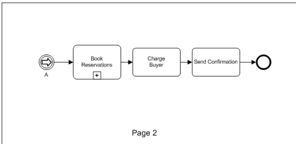
Figure 10.42 - Link Intermediate Event Used as Off-Page Connector
