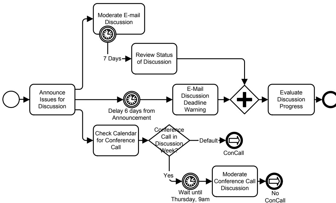
Figure A.32 - “Discussion Cycle” Sub-Process Details
