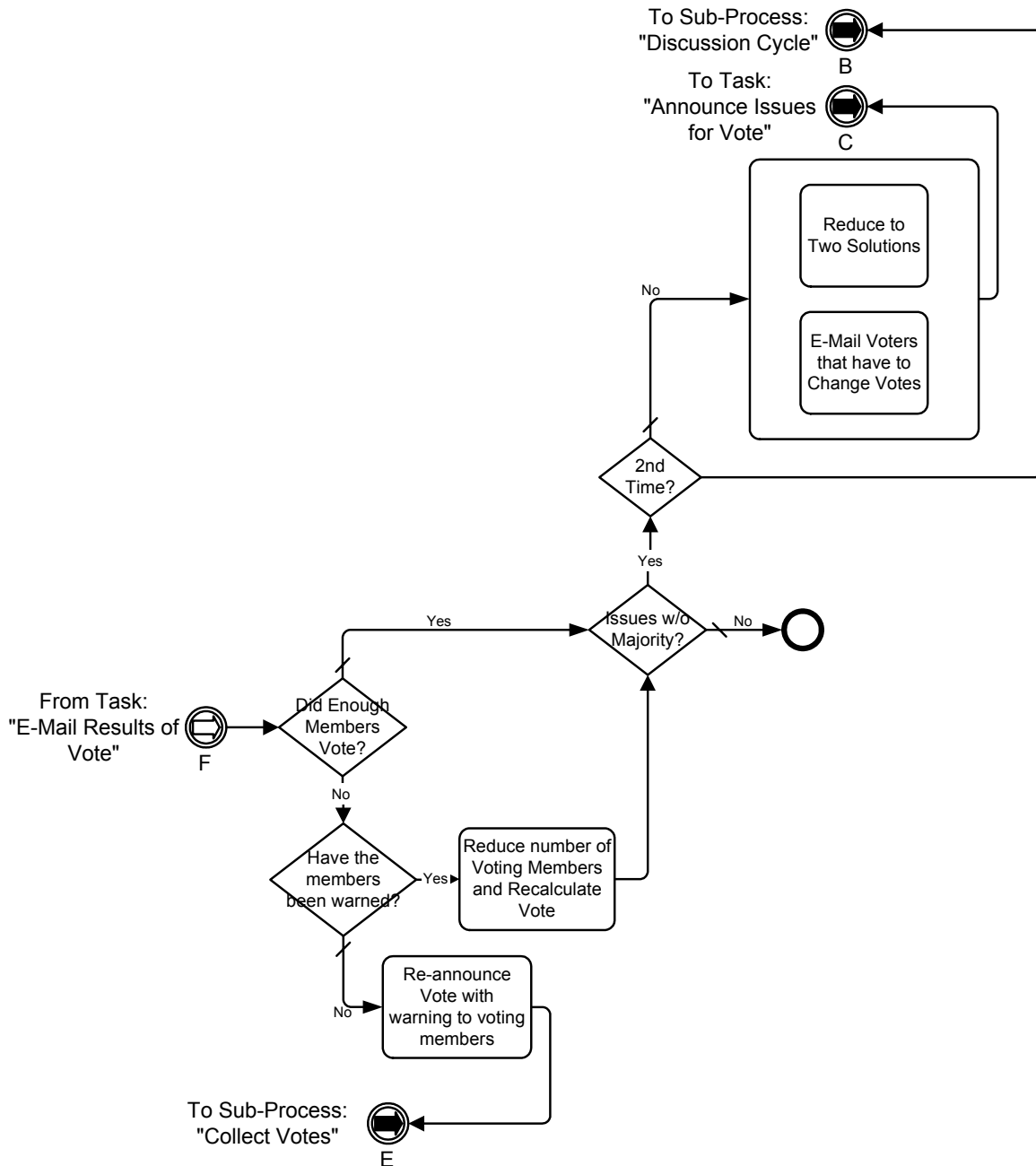
Figure A.33 - The last segment of the E-Mail Voting Process
