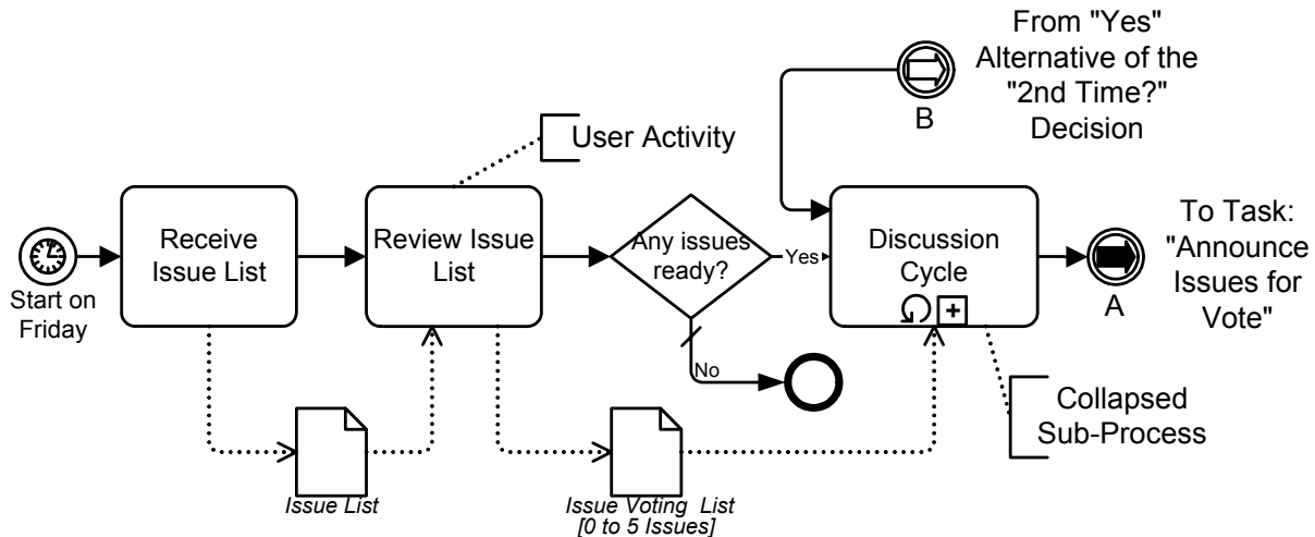
Figure A.30 - The Start of the Process
