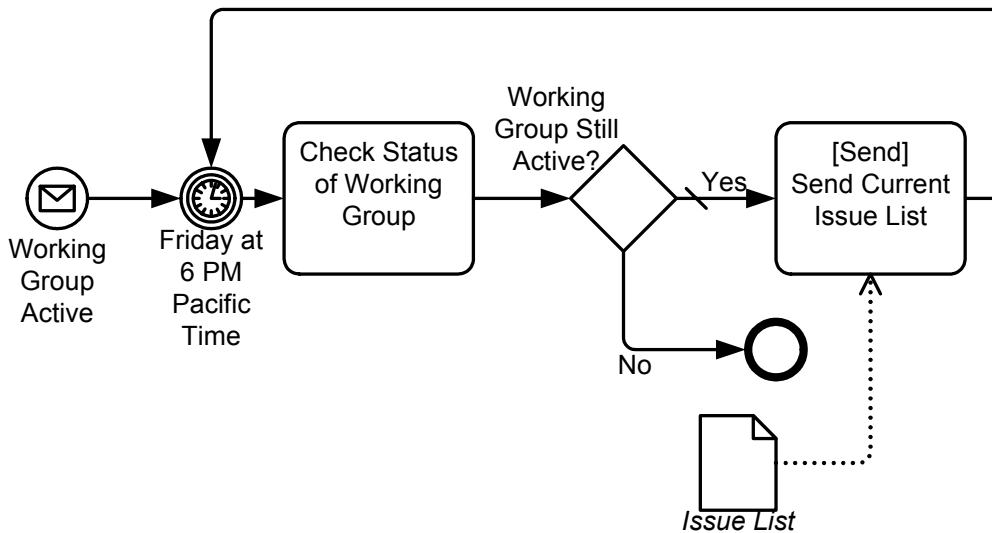
Figure A.31 - The Ongoing Starter Process
