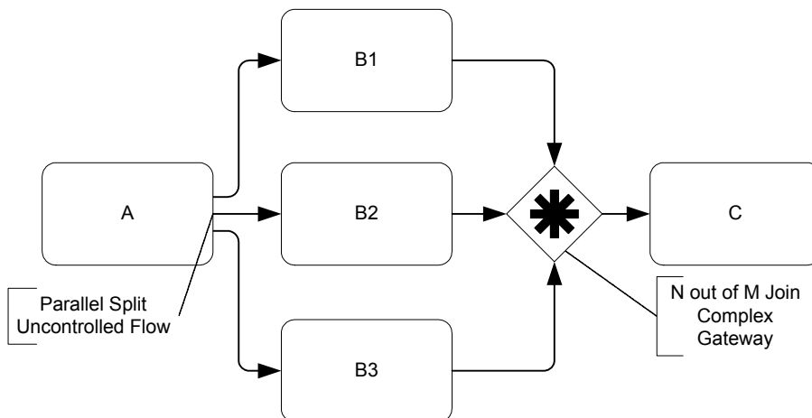
Figure 10.34 - Workflow Pattern #8 -- N out of M Join
