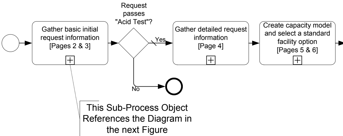
Figure 9.10 - A Sub-Process Object with its Details Shown in the diagram of the next Figure
