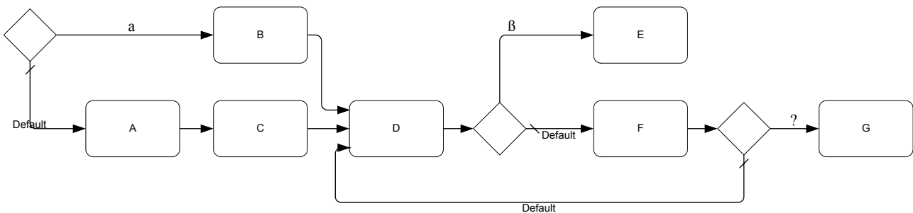
Figure 10.39 - Workflow Pattern #16 -- Arbitrary Cycle
