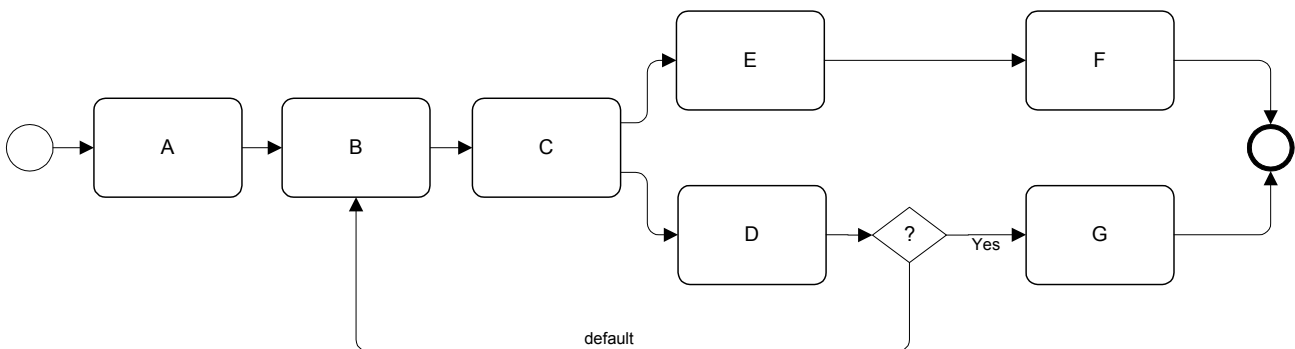
Figure 10.51 - Improper Looping
