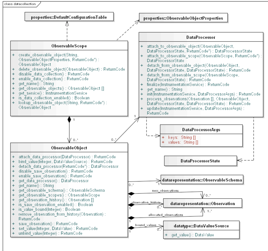
Figure 9 Data Collection Module
