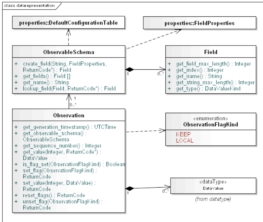
Figure 8 Data Representation Module
