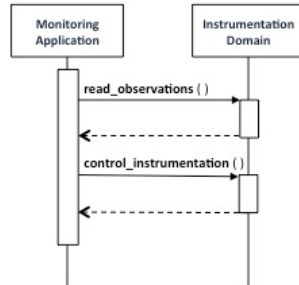
Figure 6 Example interaction with Instrumentation Domain
