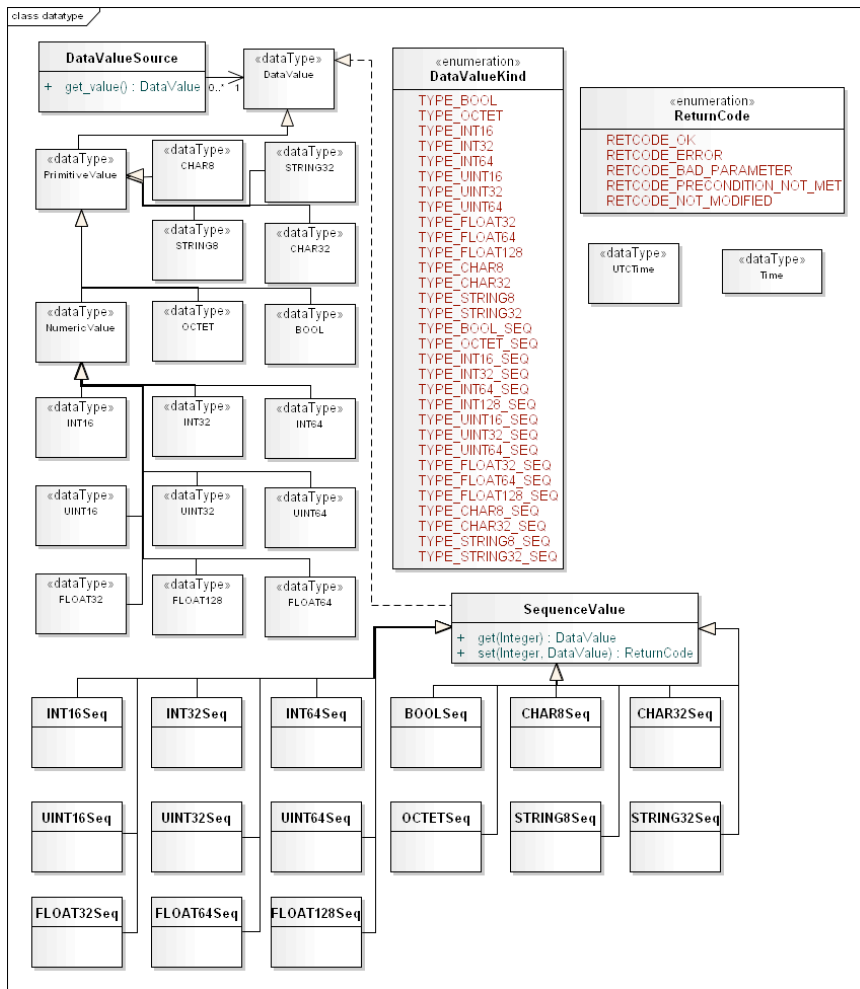
Figure 10 Data Type Module
