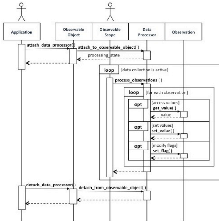
Figure 5 Data Processing Example
