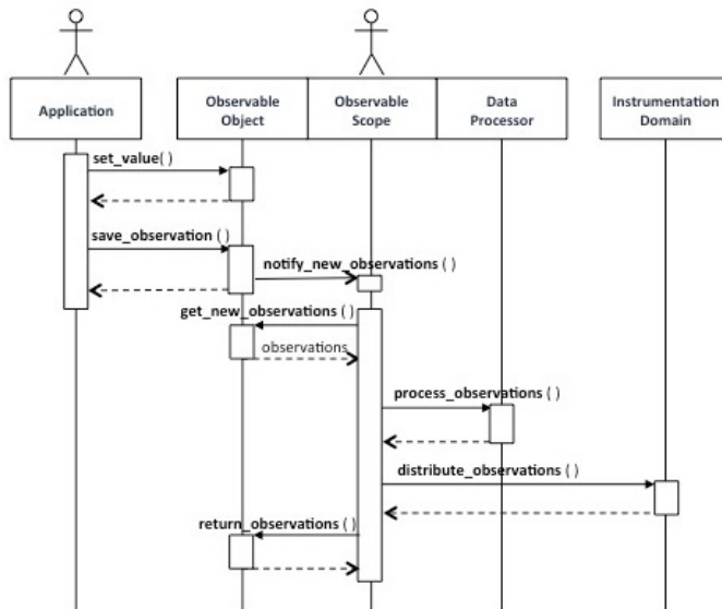
Figure 4 Example of data collection
