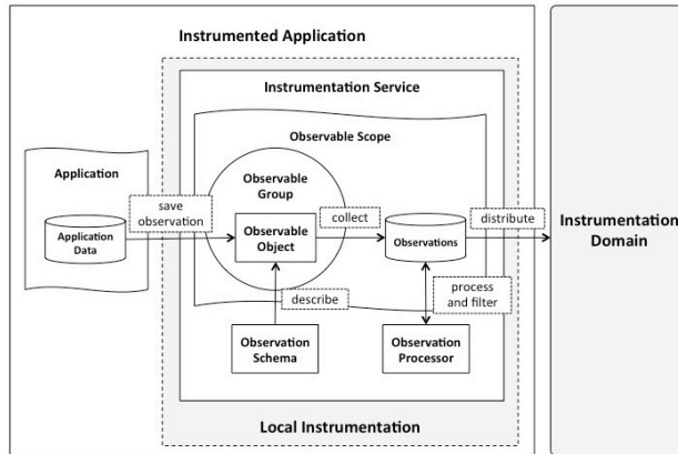
Figure 3 Components of the local instrumentation
