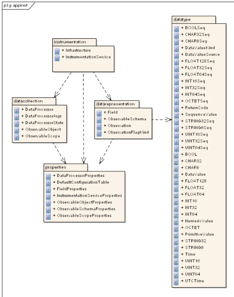
Figure 1 Application Instrumentation PIM
