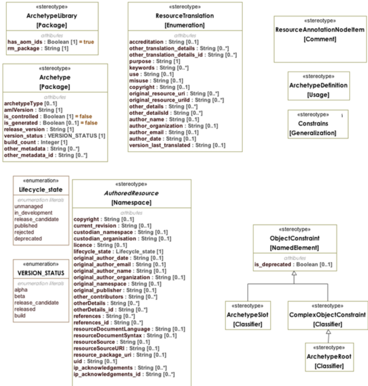
Figure 4. Constraint Profile
