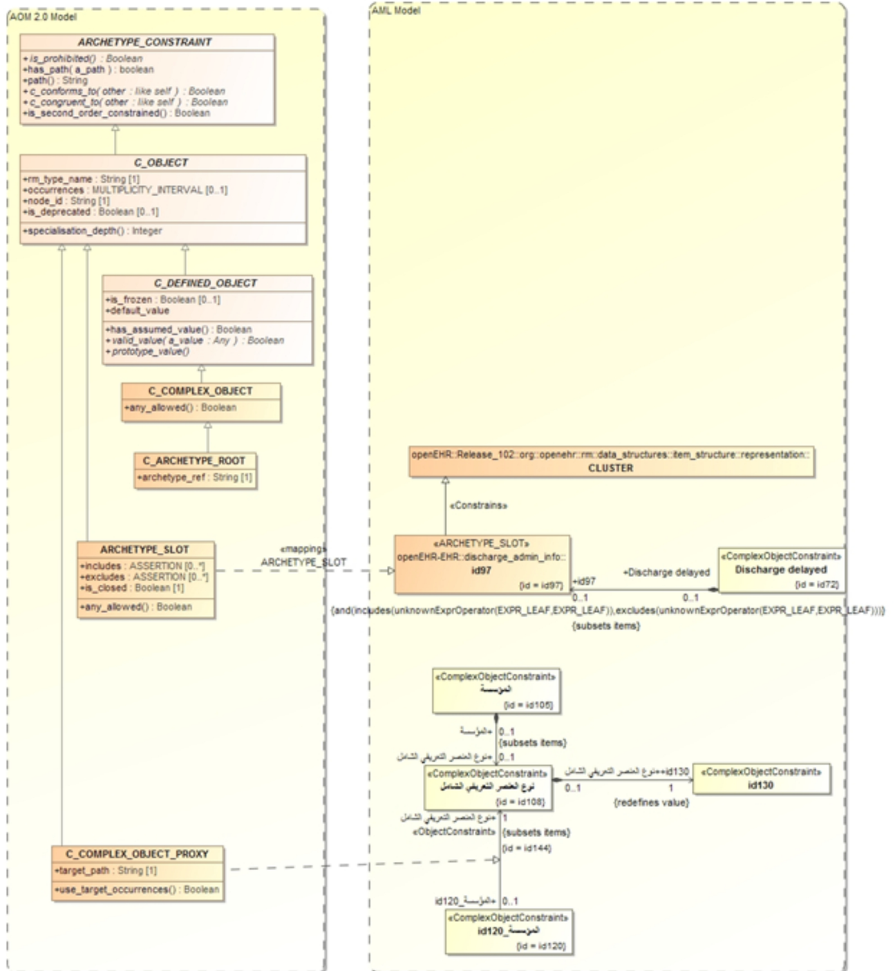
Figure 15. Object Reference Mapping
