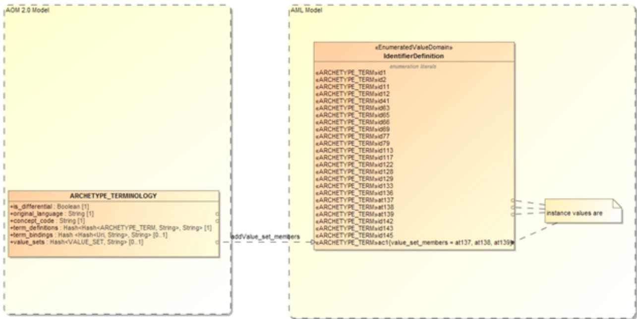
Figure 13. Local Value-sets
