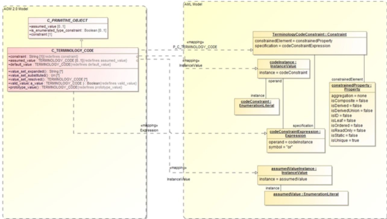
Figure 18. Code Constraint Mapping Overview
