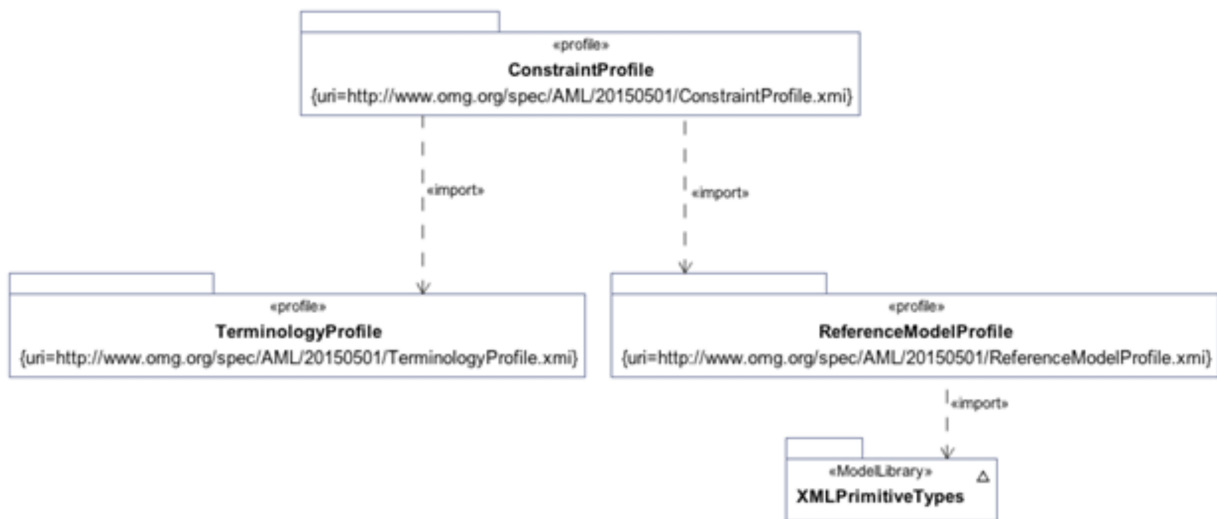
Figure 1. AML Dependencies
