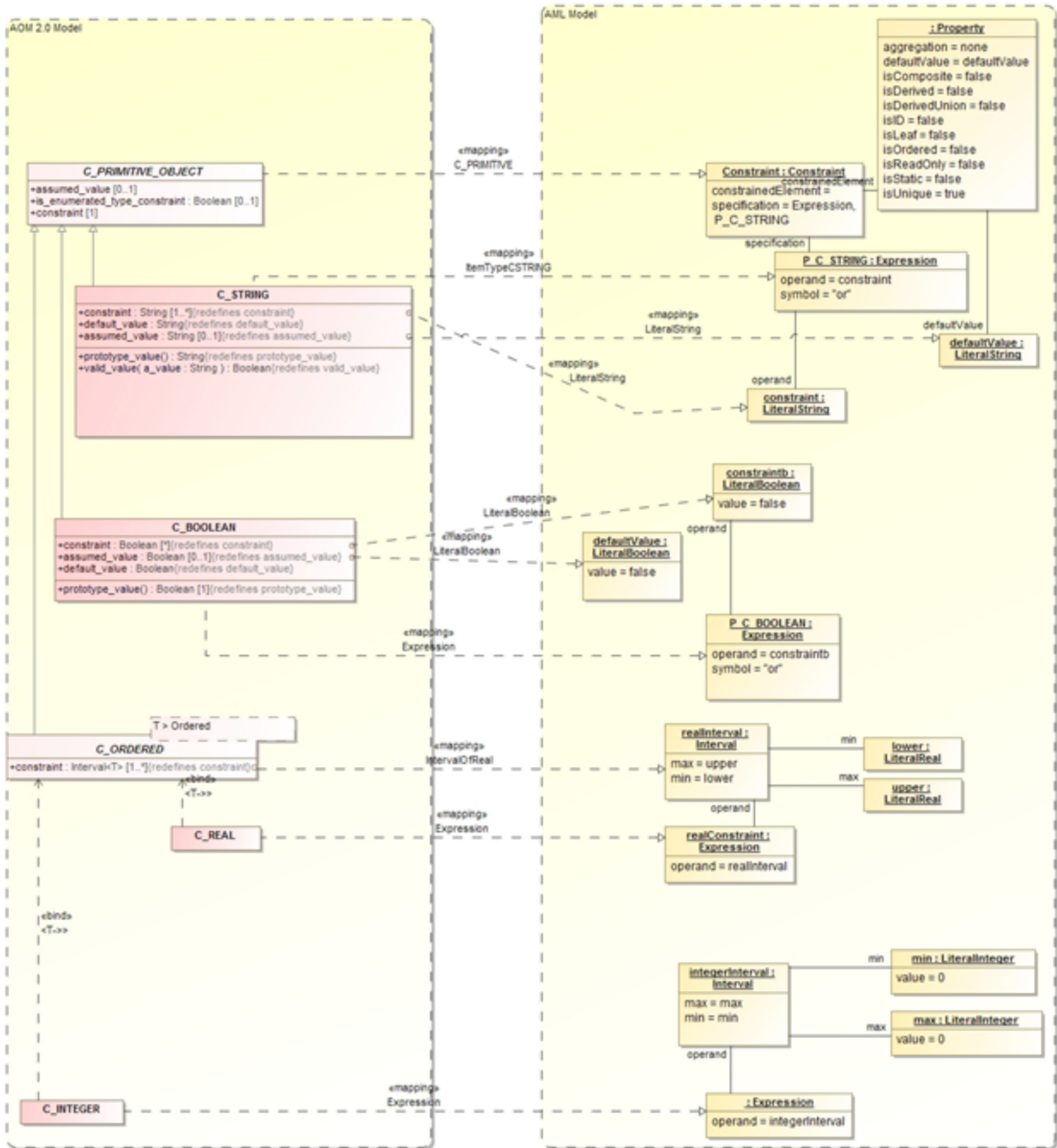
Figure 16. Primitive Constraints
