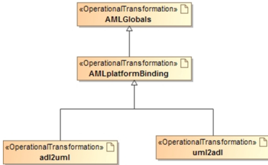
Figure 6. AML Transformations
