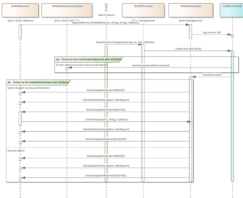
Figure 6-7-7: Alert Registration and Creation Sequence Diagram
