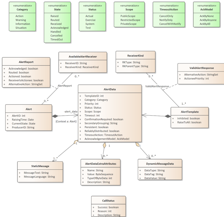
Figure 6-2-2: PIM class diagram for ALMAS Data Model
