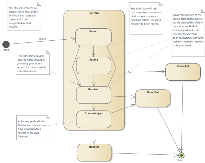
Figure 6.5-5: Action/Situation Alert Lifecycle
