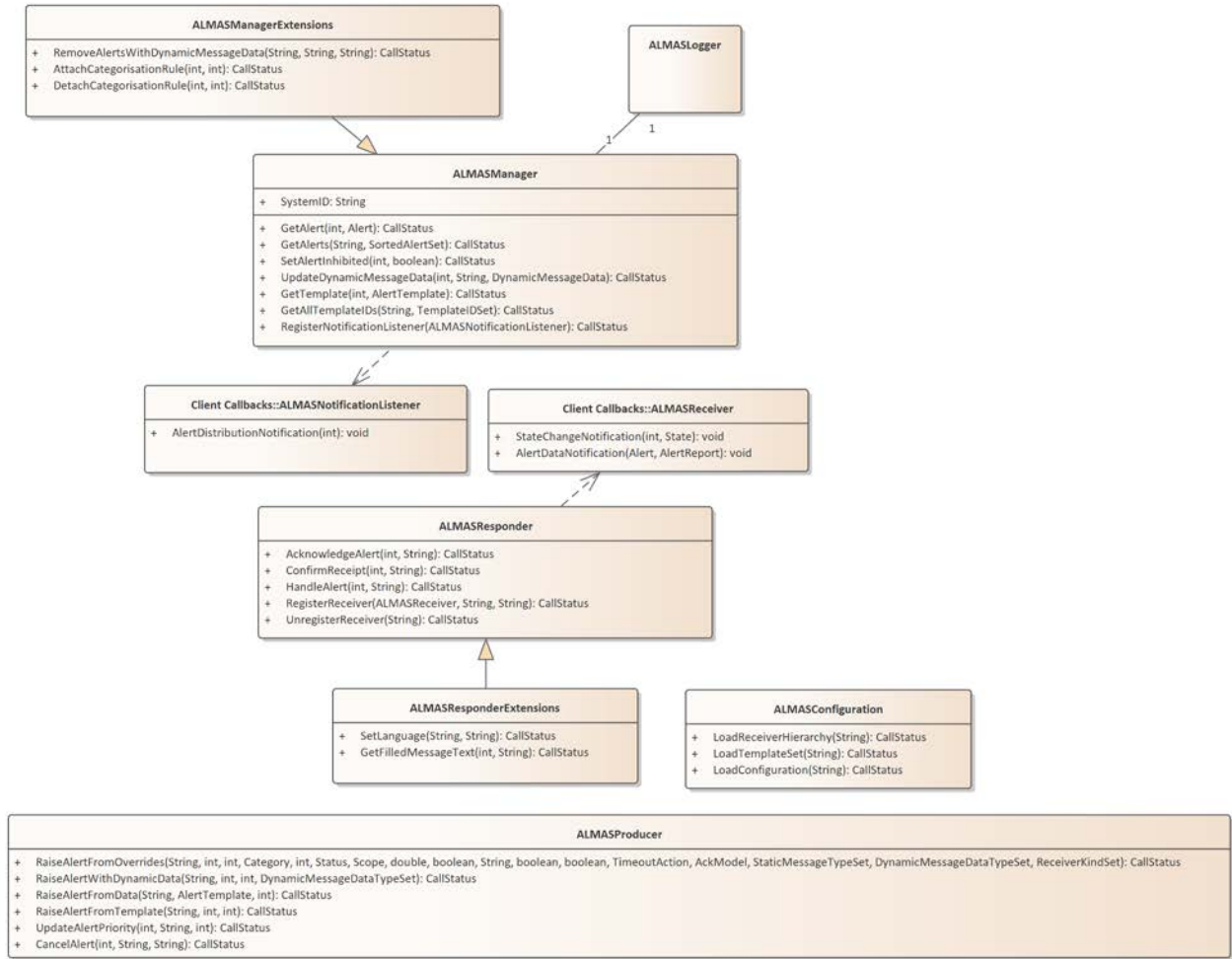
Figure 6.3 : PIM class diagram for ALMAS Management
