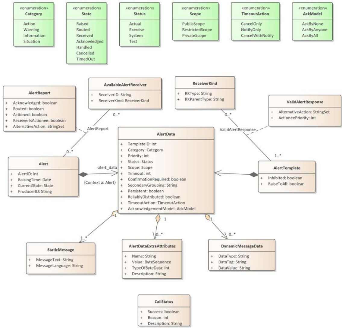
Figure 6.2 : PIM class diagram for ALMAS Data Model
