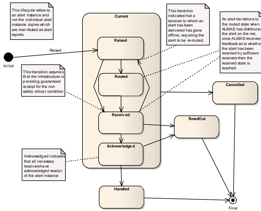
Figure 6.5 : Action/Situation Alert Lifecycle
