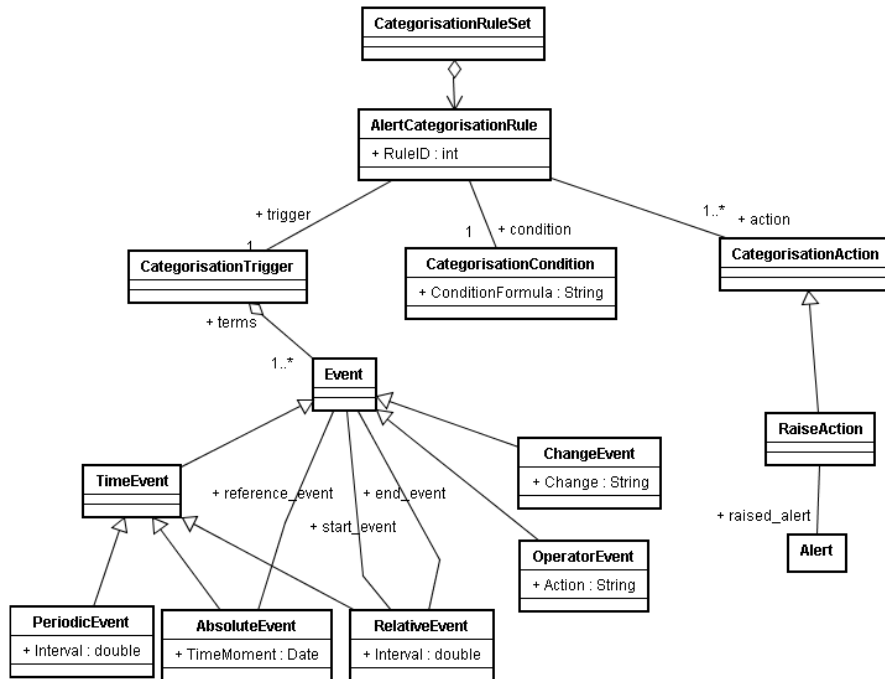
Figure 6.4 : Alert Categorisation Platform Independent Model
