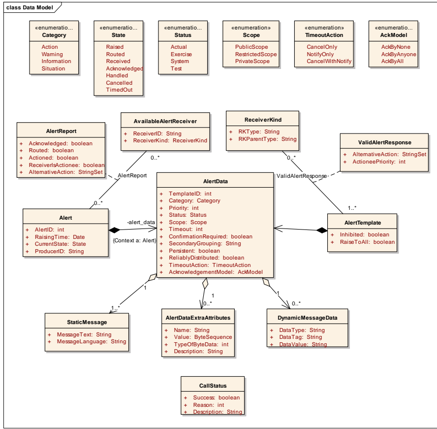
Figure 6.2 : PIM class diagram for ALMAS Data Model
