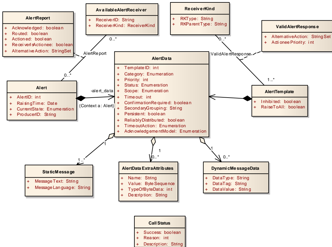
Figure 6.2 : PIM class diagram for ALMAS Data Model
