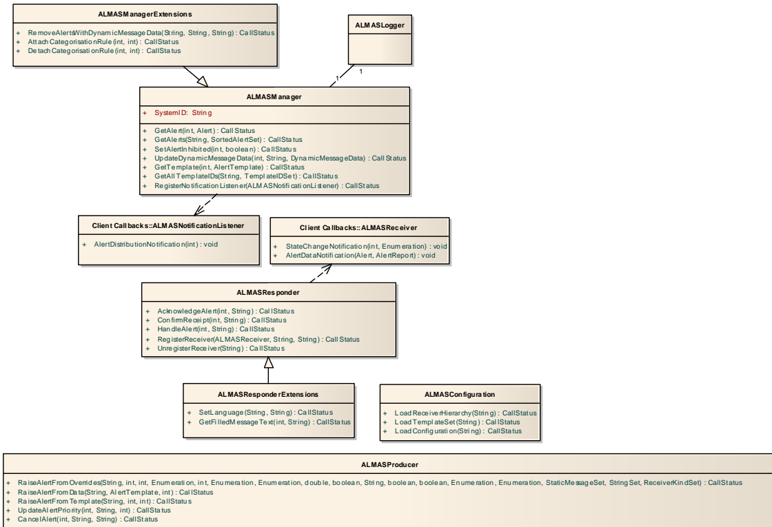
Figure 6.3 : PIM class diagram for ALMAS Management
