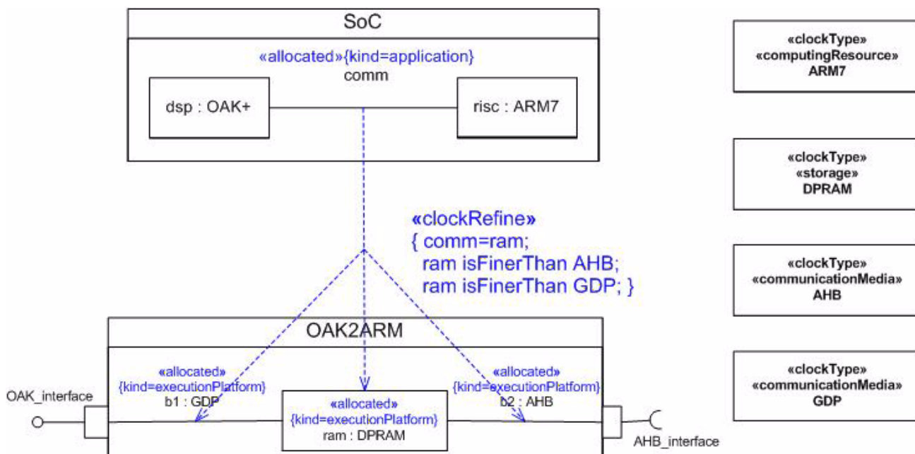
Figure 11.8 - Communication refinement
