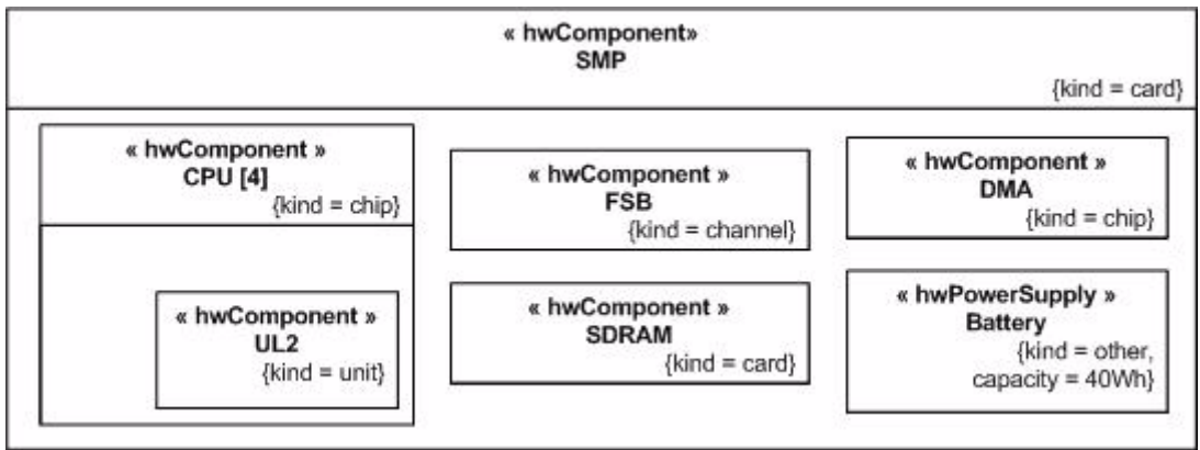
Figure 14.81 - SMP physical view
