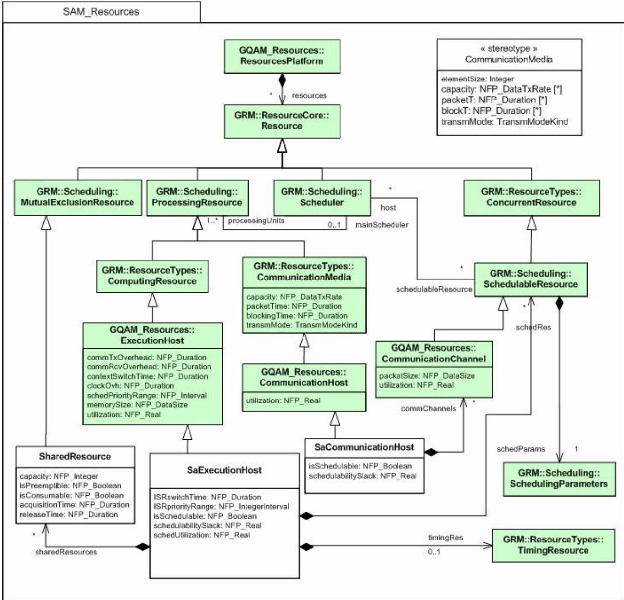
Figure 16.6 - The SAM Resources domain model
