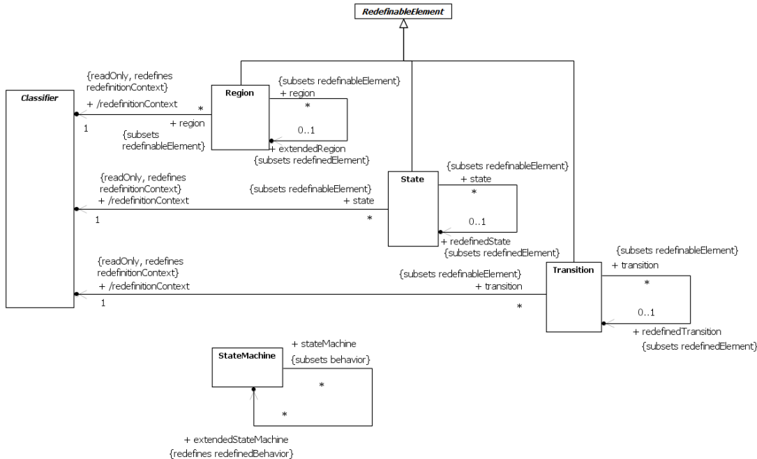
Figure 14.37 StateMachine redefinition
