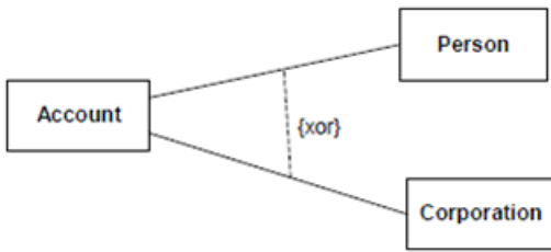
Figure 7.16 {xor} constraint
