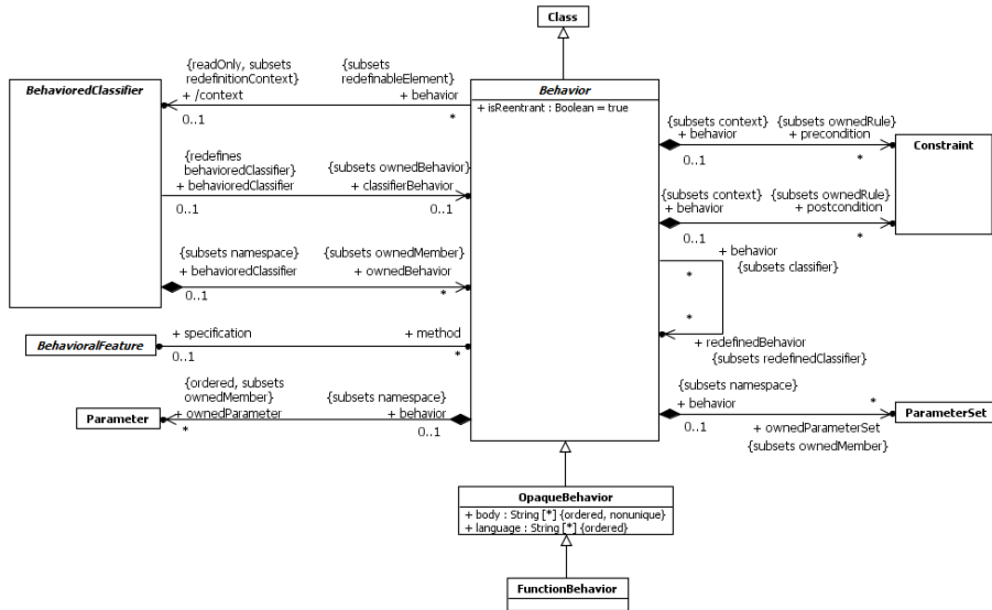
Figure 13.1 Behaviors
