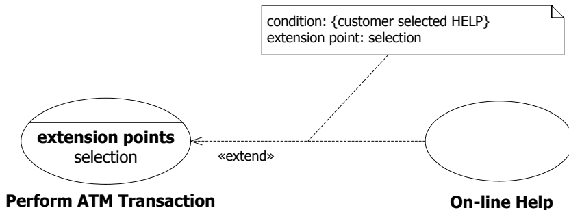
Figure 18.3 Example Extend
