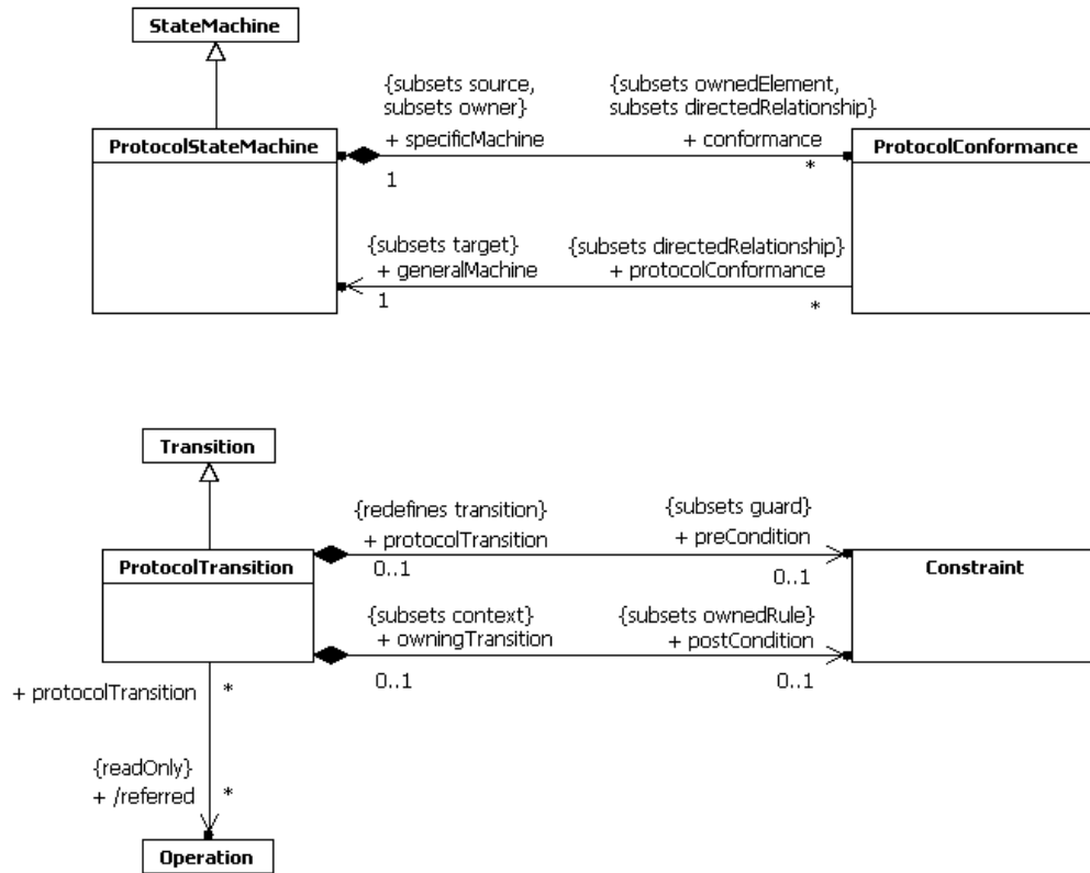
Figure 14.41 ProtocolStateMachines
