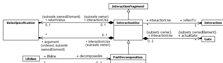
Figure 17.18 InteractionUses
