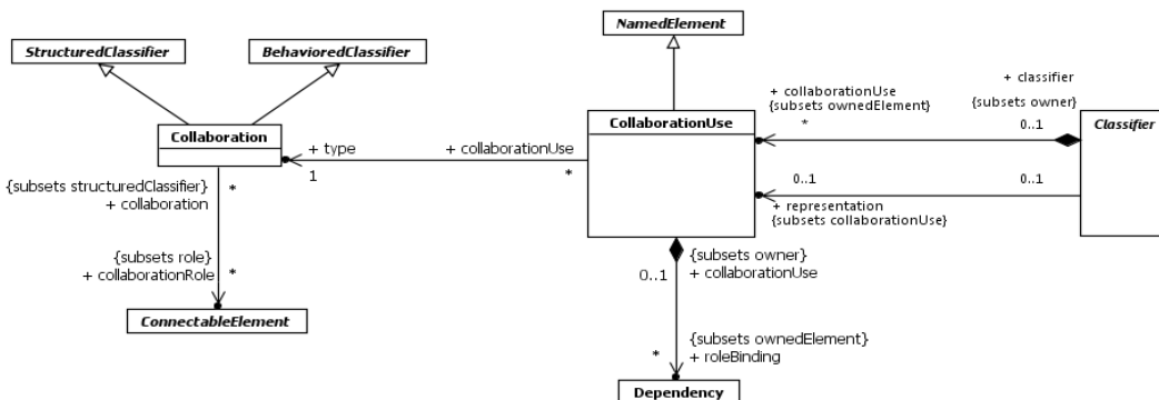
Figure 11.49 Collaborations
