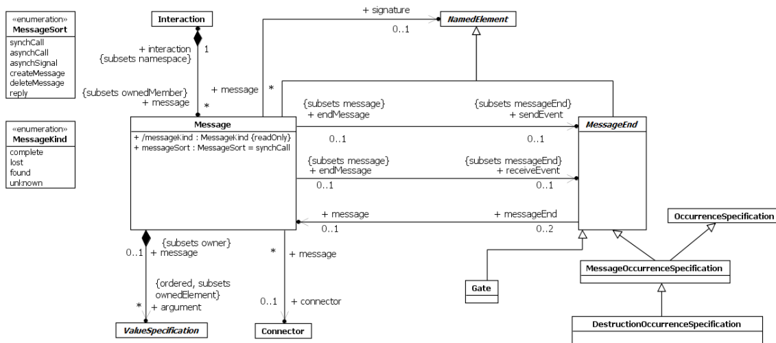
Figure 17.7 Messages
