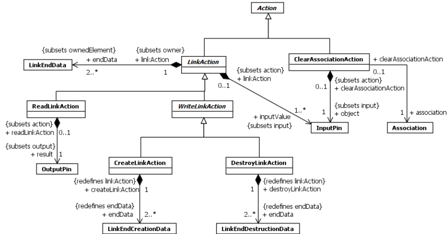
Figure 16.34 Link Actions
