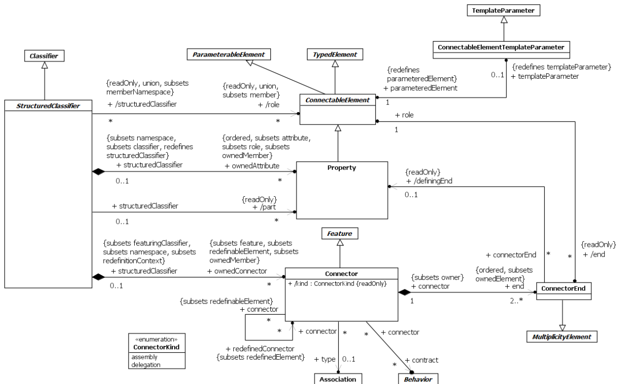
Figure 11.1 Structured Classifiers
