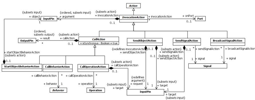
Figure 16.13 Invocation Actions
