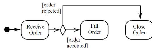
Figure 15.40 DecisionNode example
