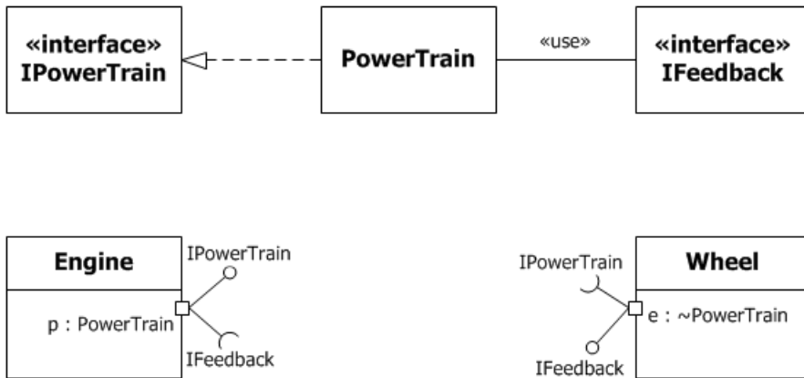
Figure 11.11 Port notation
