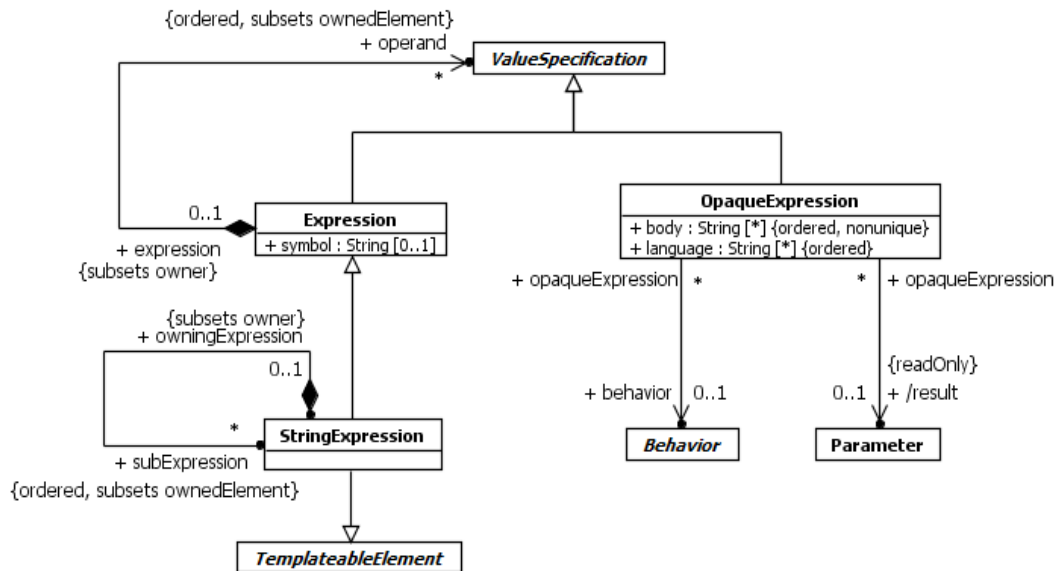
Figure 8.2 Expressions
