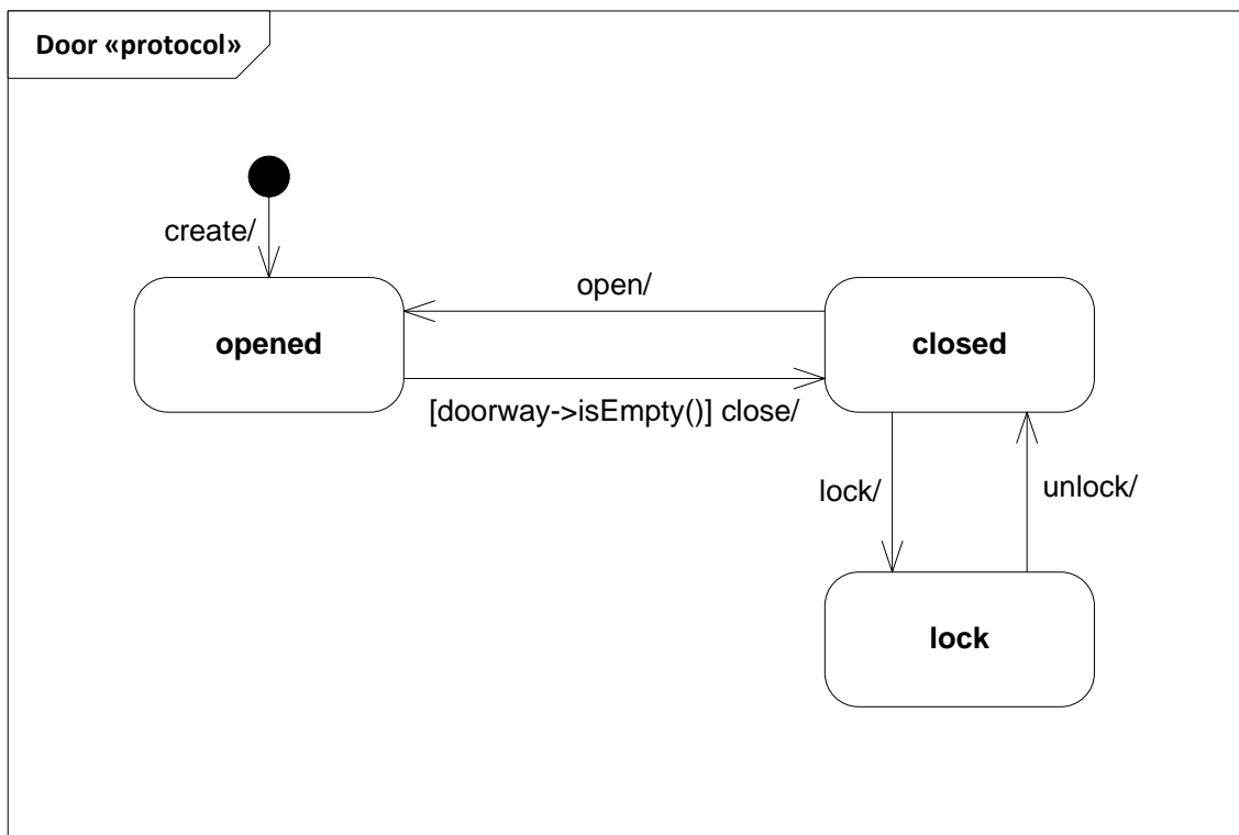
Figure 14.44 ProtocolStateMachine example
