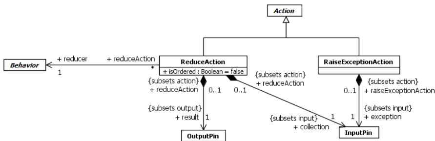
Figure 16.56 Other Actions
