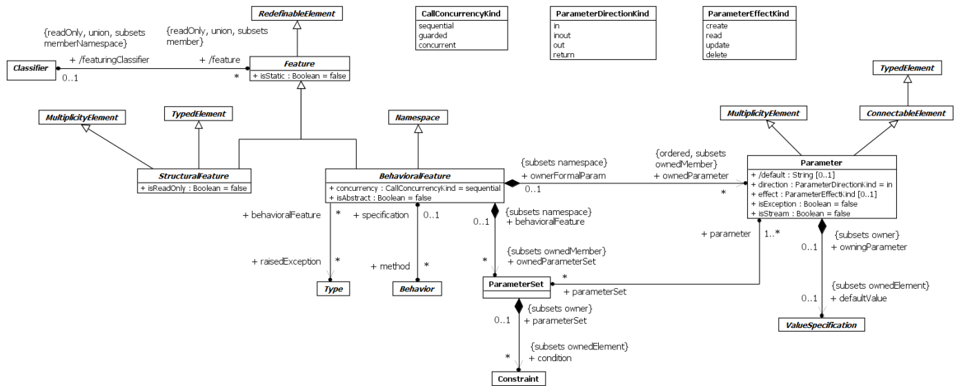
Figure 9.9 Features
