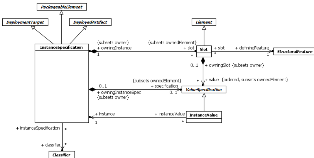
Figure 9.27 Instances
