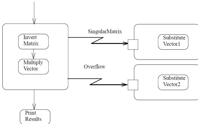
Figure 15.64 ExceptionHandler example
