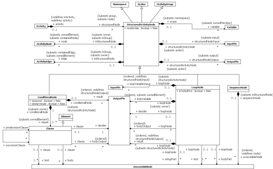
Figure 16.45 Structured Actions
