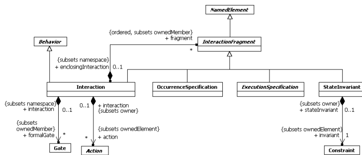
Figure 17.1 Interactions
