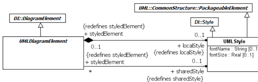
Figure B.8 UML Styles
