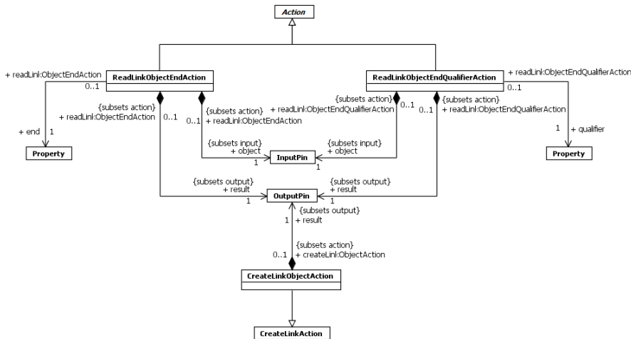
Figure 16.35 Link Object Actions
