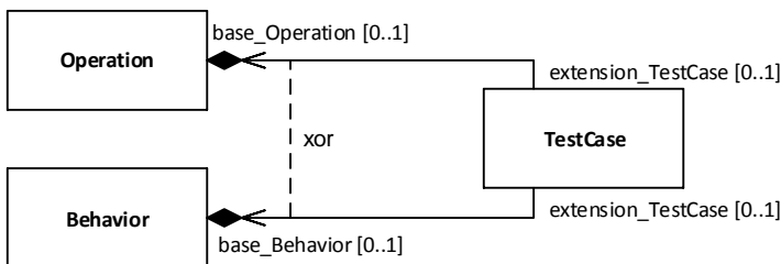
Figure 12.17 MOF Model Equivalent to Multiple Metaclass Extension
