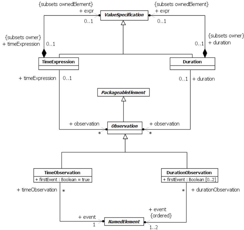
Figure 8.3 Time and Duration
