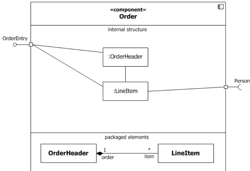
Figure 11.48 Delegation Connectors connect externally provided Interfaces to the parts that realize or require them.
