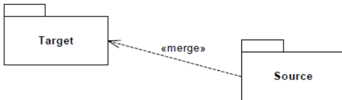
Figure 12.4 Notation for Package Merge
