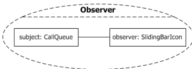
Figure 11.50 The internal structure of the Observer Collaboration
