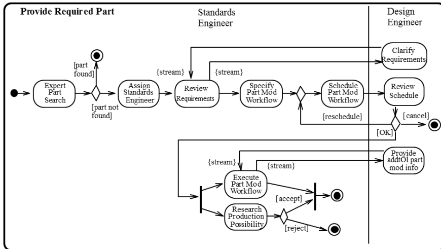
Figure 15.23 Part selection workflow example
