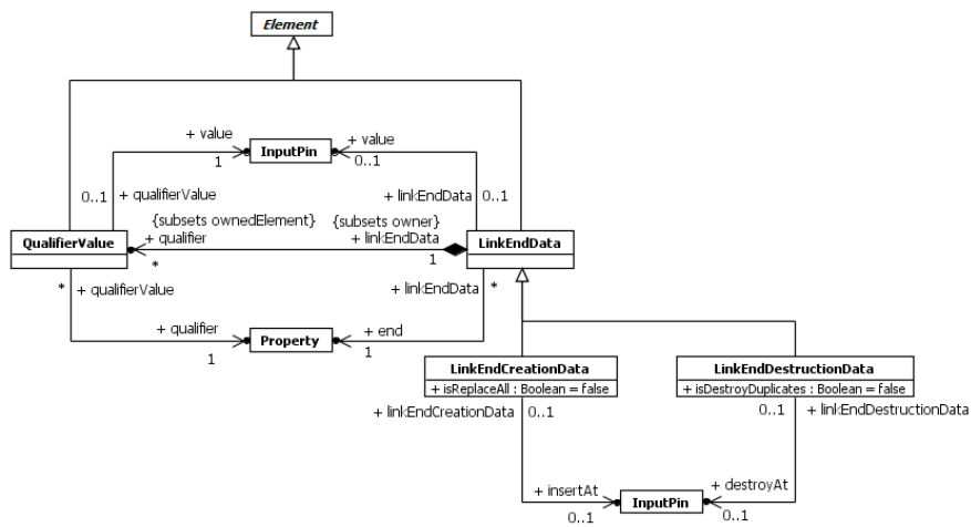
Figure 16.33 Link End Data
