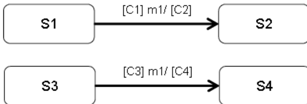
Figure 14.43 Example of several ProtocolTransitions associated with the same operation (m1)
