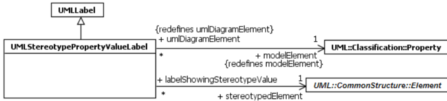
Figure B.7 Stereotype Application Labels
