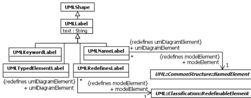
Figure B.5 Labels
