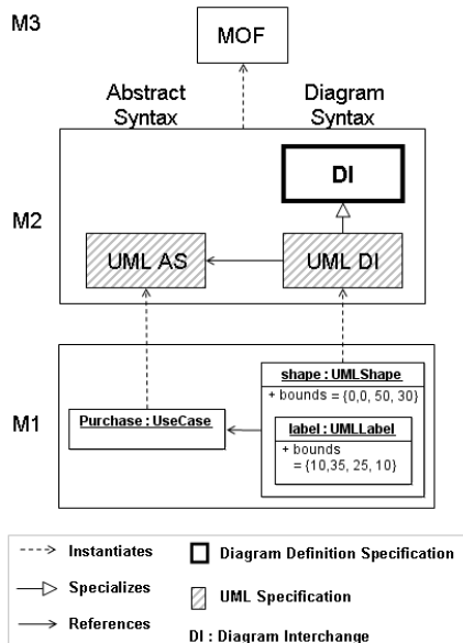
Figure B.2 UML Diagram Interchange Architecture
