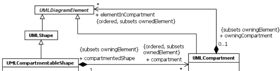
Figure B.6 UML Compartmentable Shapes
