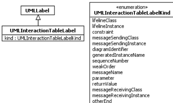
Figure B.15 Interaction Shapes
