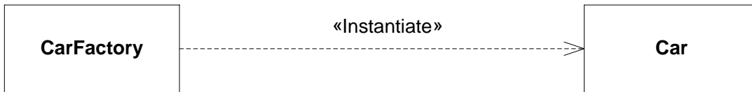
Figure 7.19 An example of an «Instantiate» Dependency
