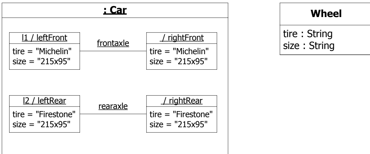
Figure 11.21 An Instance of the Car Class
