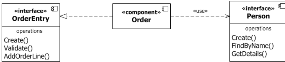
Figure 11.43 Explicit representation of provided and required Interfaces using Dependency notation.
