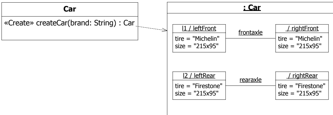
Figure 11.23 A constructor for the Car Class
