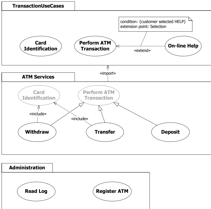
Figure 18.11 Example UseCases owned by Packages
