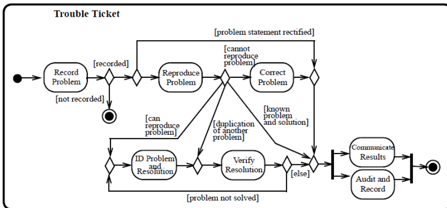
Figure 15.24 Trouble ticket workflow example
