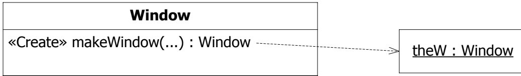
Figure 11.22 InstanceSpecification indicating a constructor
