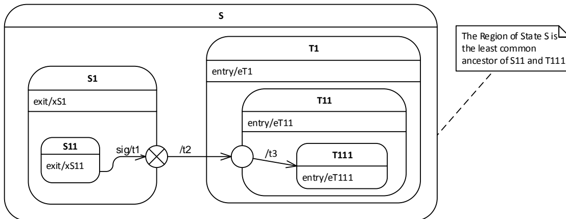
Figure 14.2 Compound transition example
