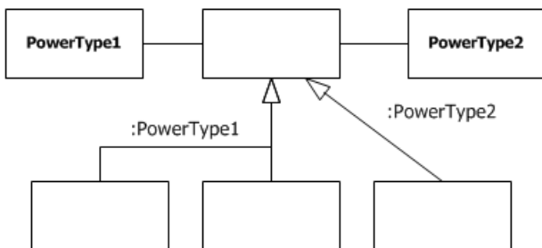
Figure 9.20 Power type notation with shared target style
