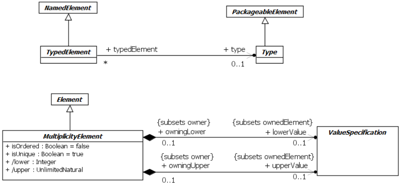
Figure 7.10 Abstract syntax of types and multiplicity elements
