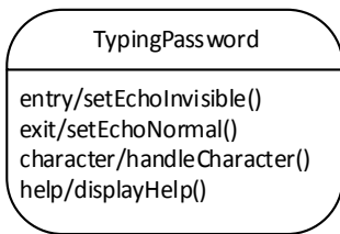
Figure 14.6 State with compartments
