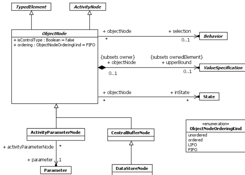
Figure 15.48 Object Nodes
