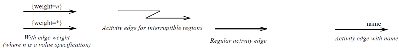
Figure 15.5 ActivityEdge notation
