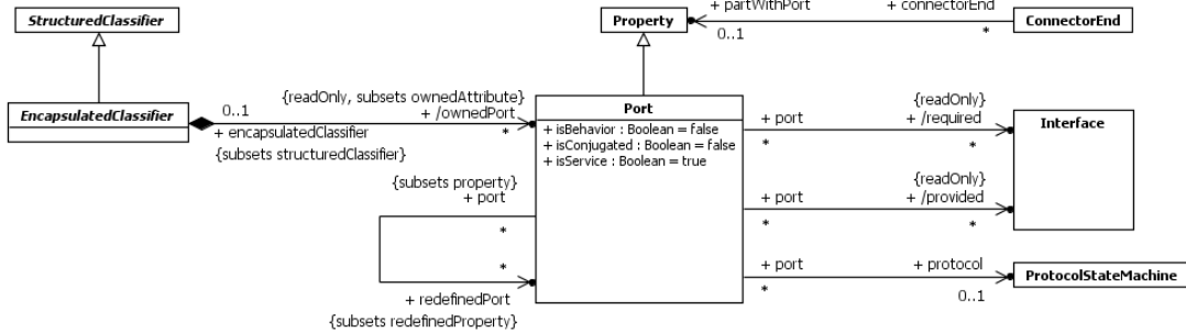
Figure 11.10 Encapsulated Classifiers
