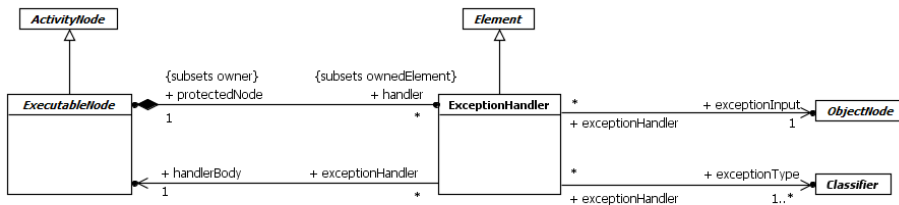
Figure 15.60 Executable Nodes
