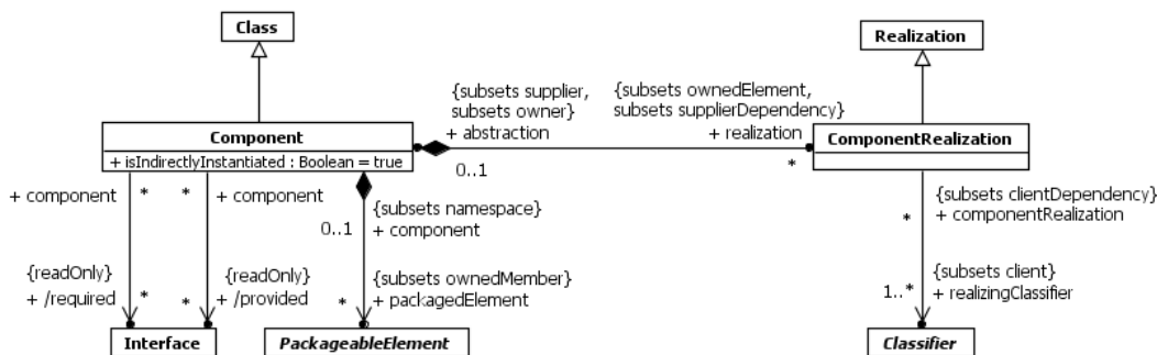
Figure 11.38 Components
