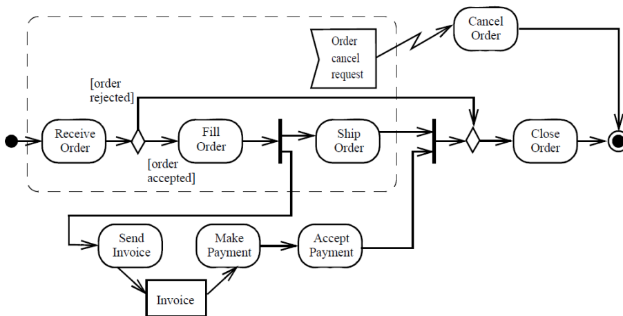
Figure 15.73 InterruptibleActivityRegion example
