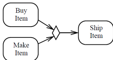
Figure 15.39 MergeNode example
