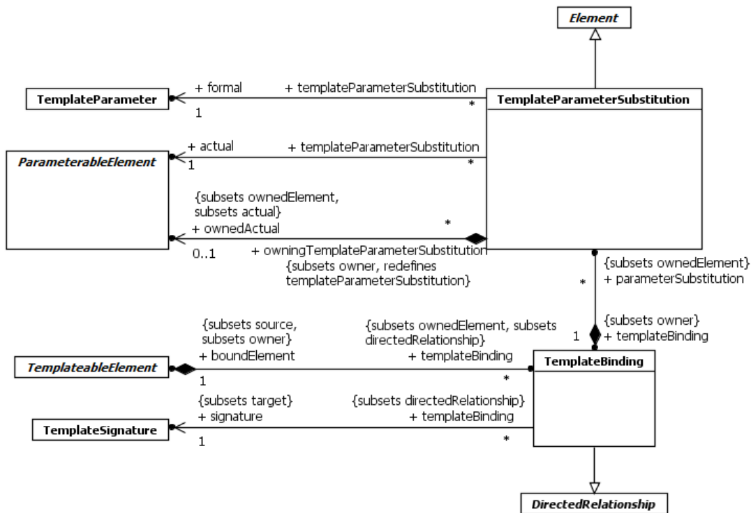
Figure 7.4 Template bindings
