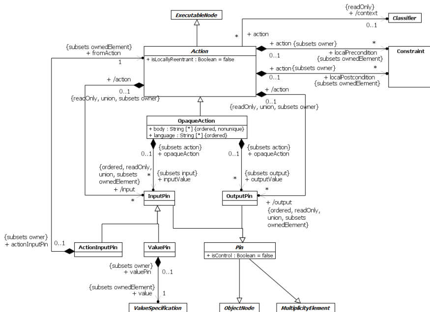
Figure 16.1 Actions
