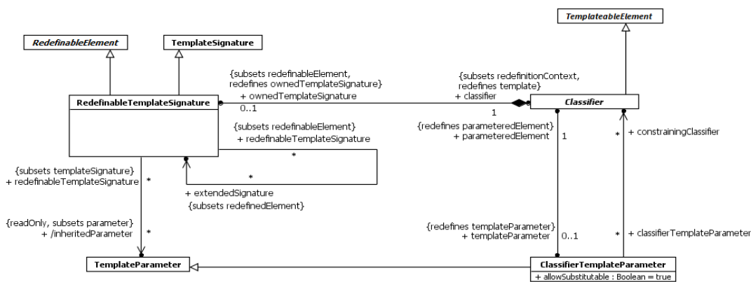
Figure 9.4 Classifier Templates
