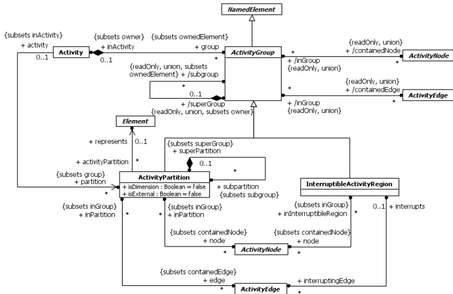
Figure 15.65 ActivityGroups
