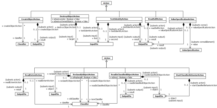
Figure 16.30 Object Actions
