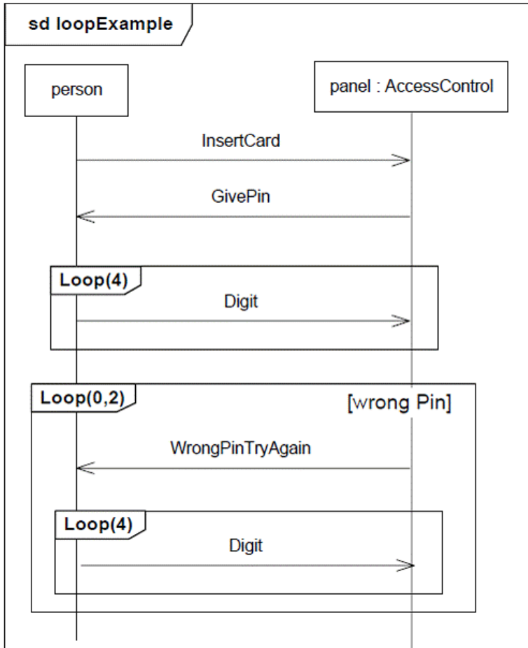
Figure 17.13 - Loop CombinedFragment
