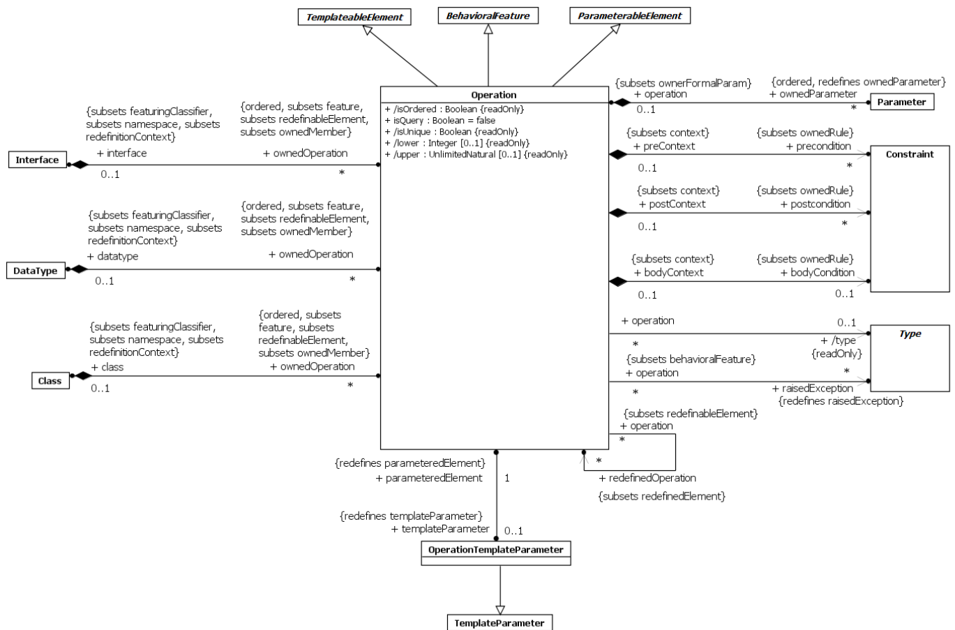
Figure 9.13 Operations
