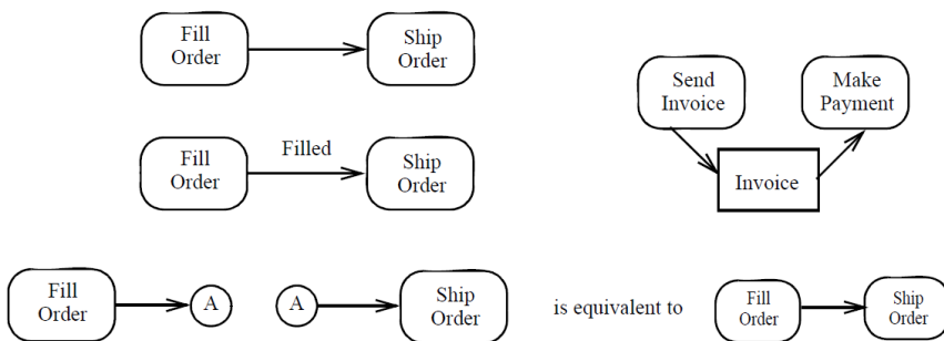
Figure 15.13 ActivityEdge examples
