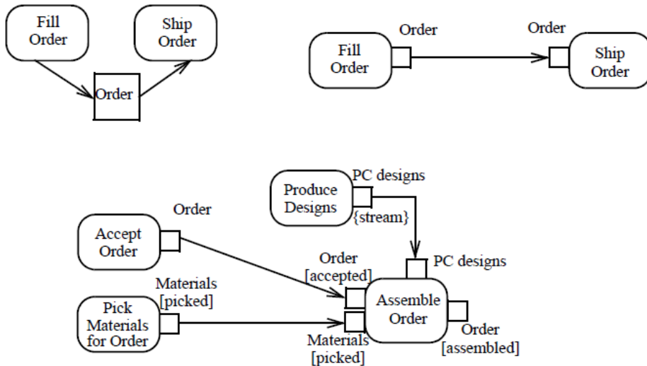
Figure 16.10 Pin examples
