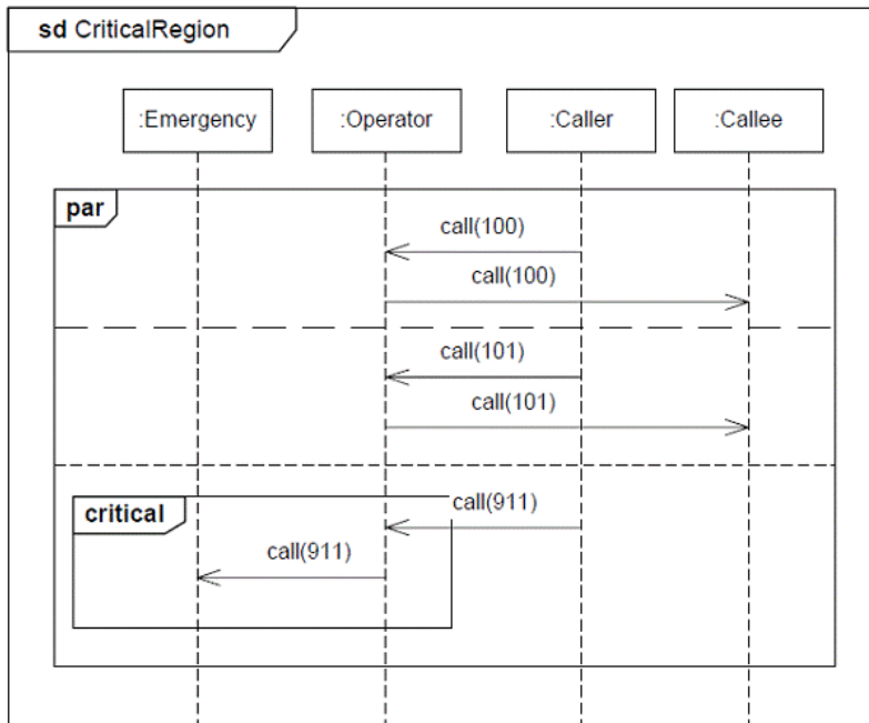
Figure 17.12 Critical Region
