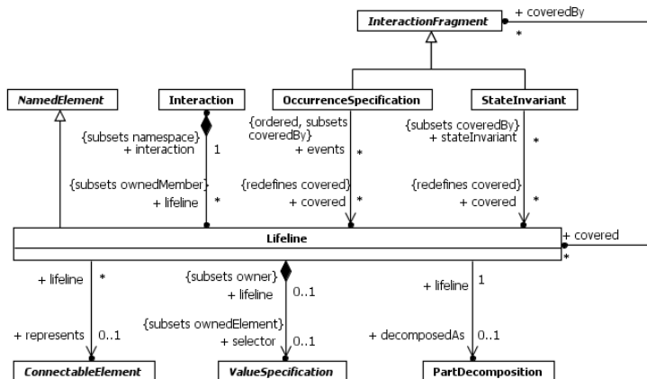
Figure 17.6 Lifelines
