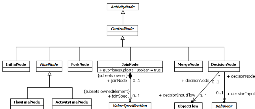
Figure 15.26 Control Nodes
