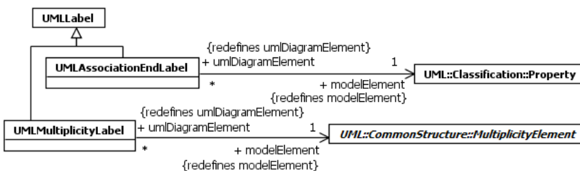
Figure B.11 Multiplicity and Association End Labels
