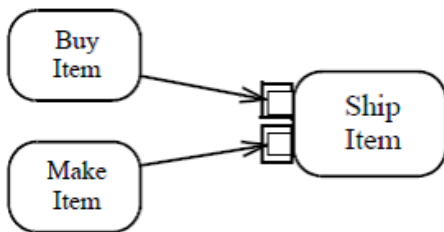
Figure 16.29 Alternative input/outputs using ParameterSets
