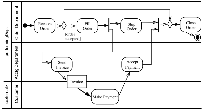
Figure 15.70 ActivityPartitions using swimlane notation
