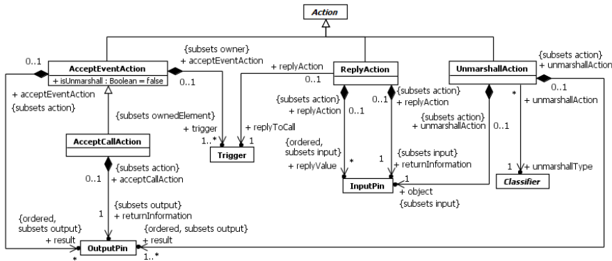
Figure 16.39 Accept Event Actions
