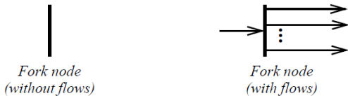
Figure 15.29 ForkNode and JoinNode notation
