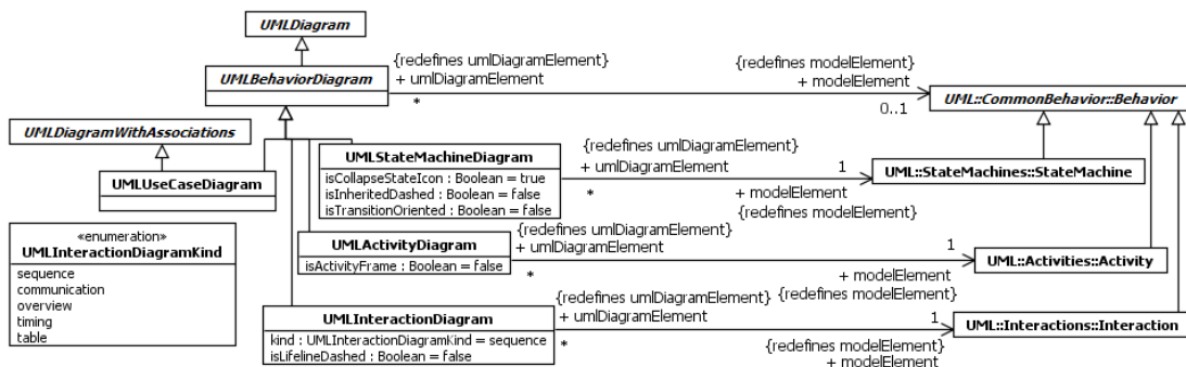
Figure B.13 Behavior Diagrams
