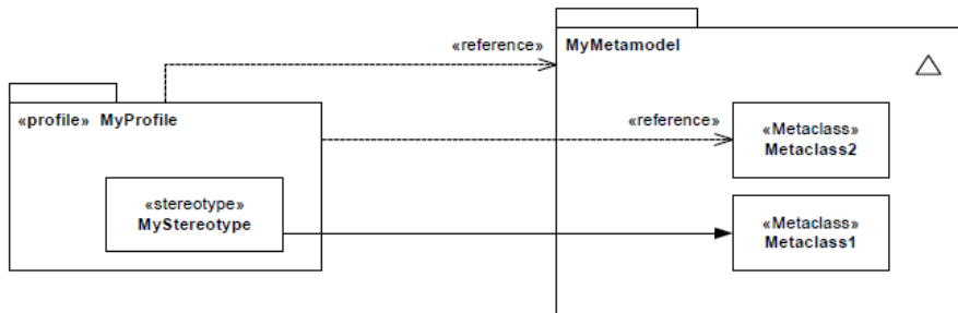
Figure 12.14 Specification of an Available Metaclass
