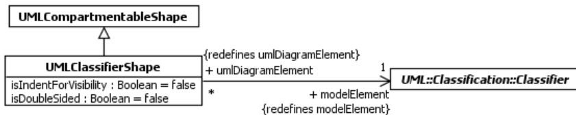
Figure B.10 Classifier Shapes
