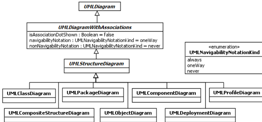
Figure B.9 Structure Diagrams
