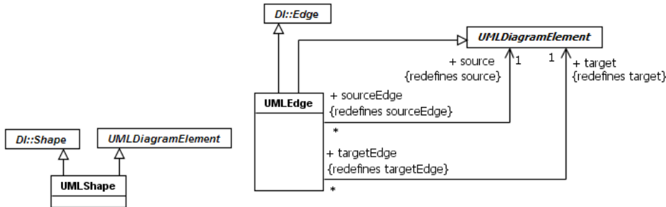
Figure B.4 UML Shapes and Edges
