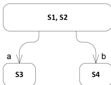
Figure 14.15 State list notation option
