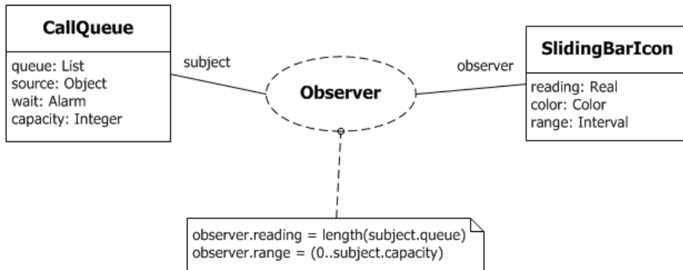
Figure 11.51 Alternative notation for the parts of the Observer Collaboration.
