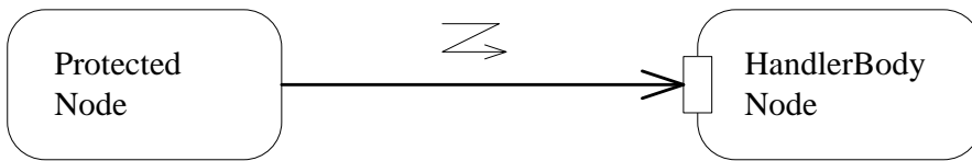
Figure 15.63 Alternative ExceptionHandler notation
