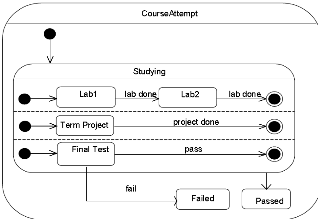
Figure 14.9 Composite State with Regions
