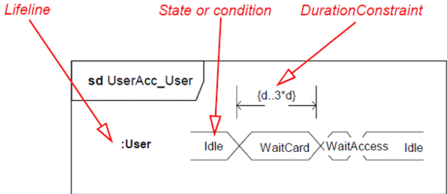
Figure 17.29 Compact Lifeline with States
