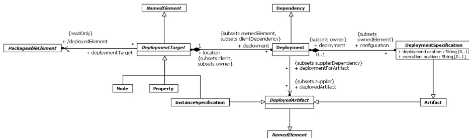
Figure 19.1 Deployments
