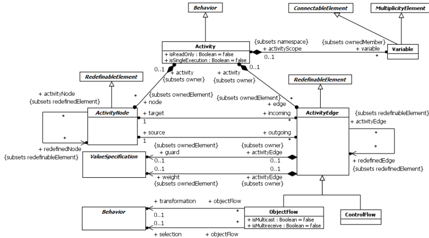
Figure 15.1 Activities
