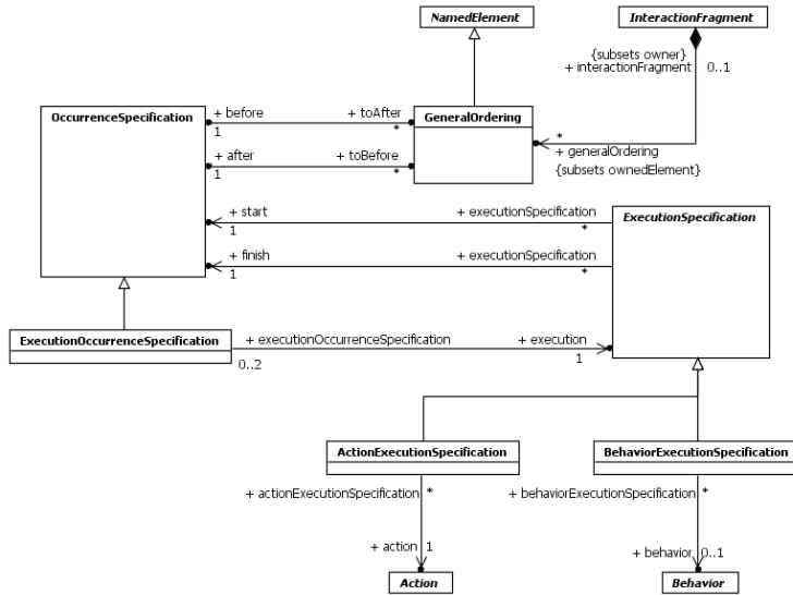
Figure 17.9 Occurrences
