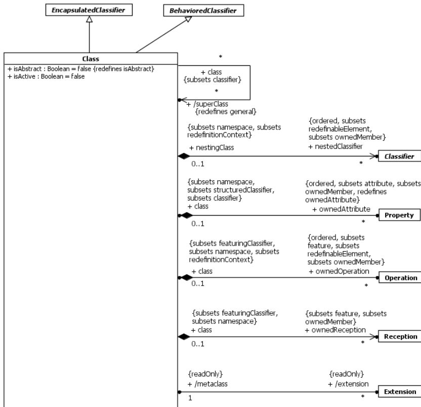
Figure 11.15 Classes
