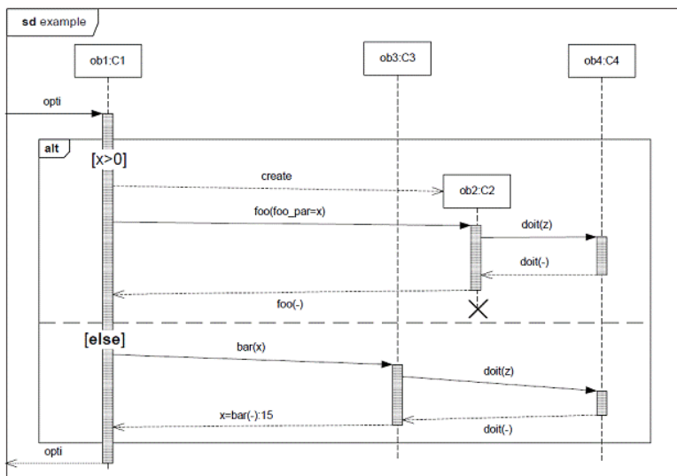
Figure 17.14 CombinedFragment
