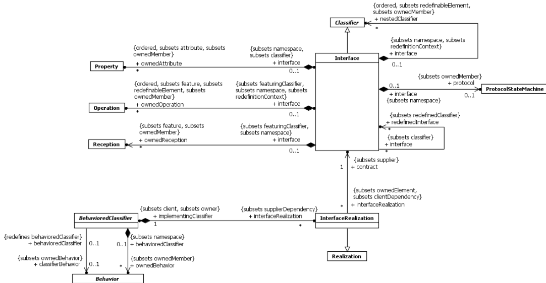
Figure 10.7 Interfaces
