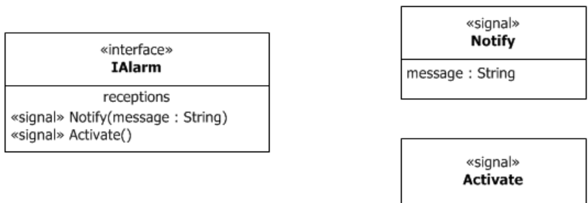
Figure 10.6 Reception Notation
