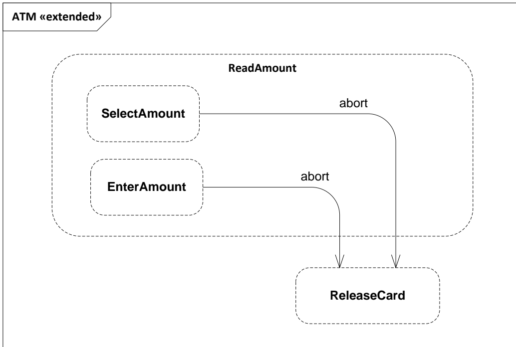
Figure 14.40 Adding Transitions
