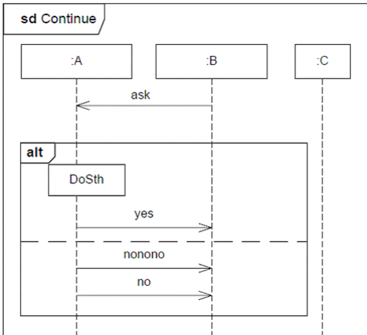
Figure 17.16 Continuation interpretation
