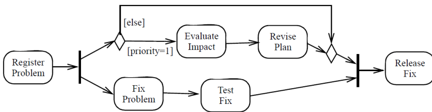
Figure 15.20 Equivalent model
