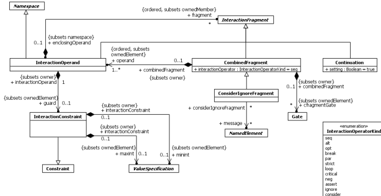
Figure 17.11 Fragments
