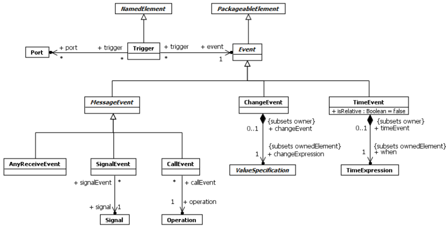
Figure 13.2 Events
