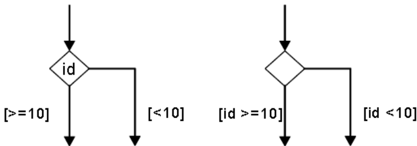
Figure 14.25 choice Pseudostates
