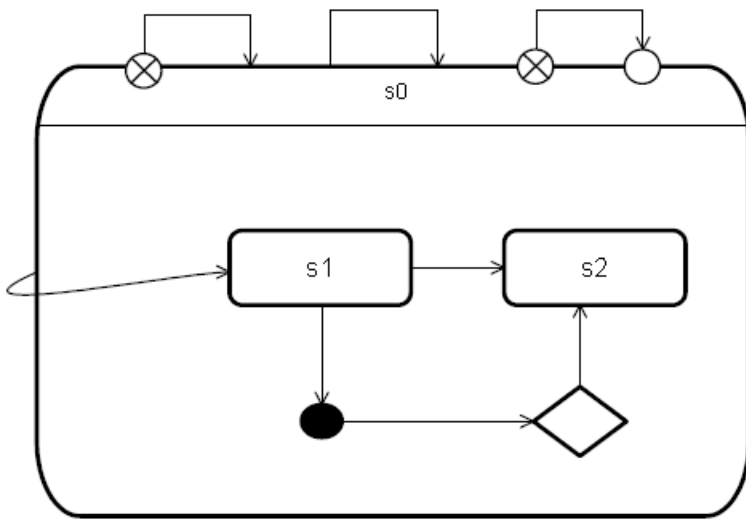
Figure 14.35 External Transitions
