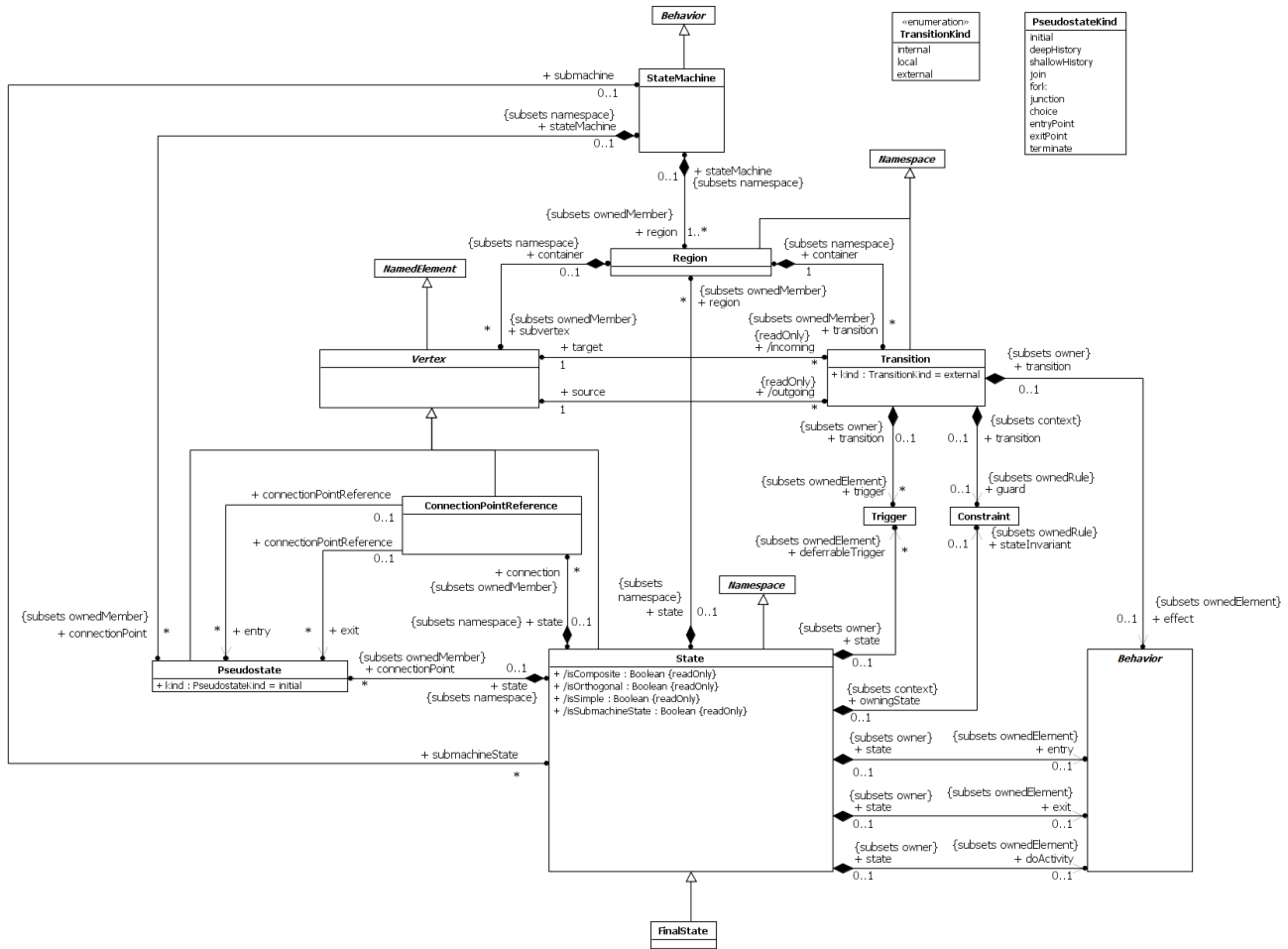
Figure 14.1 Behavior StateMachines
