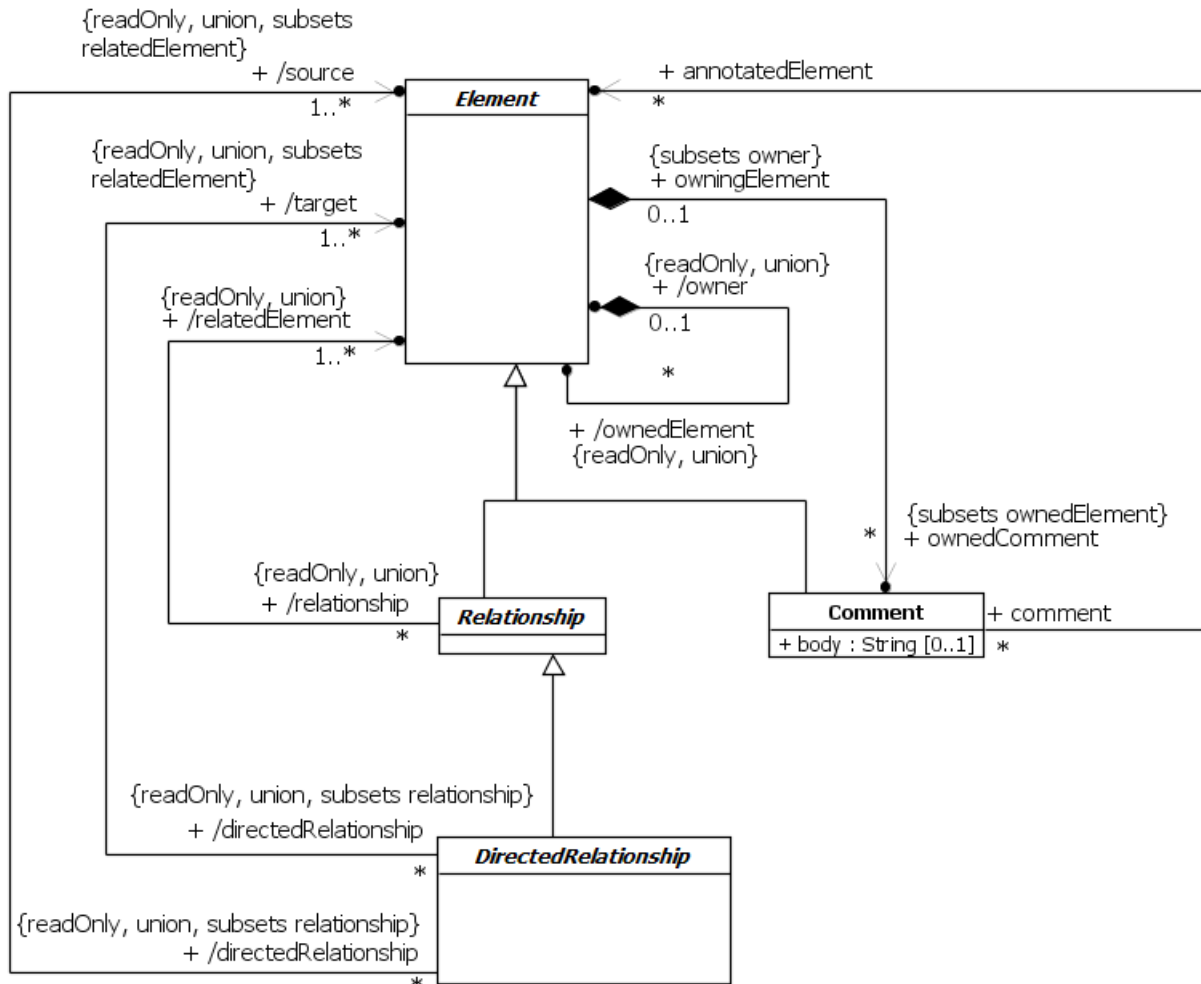
Figure 7.1 Root
