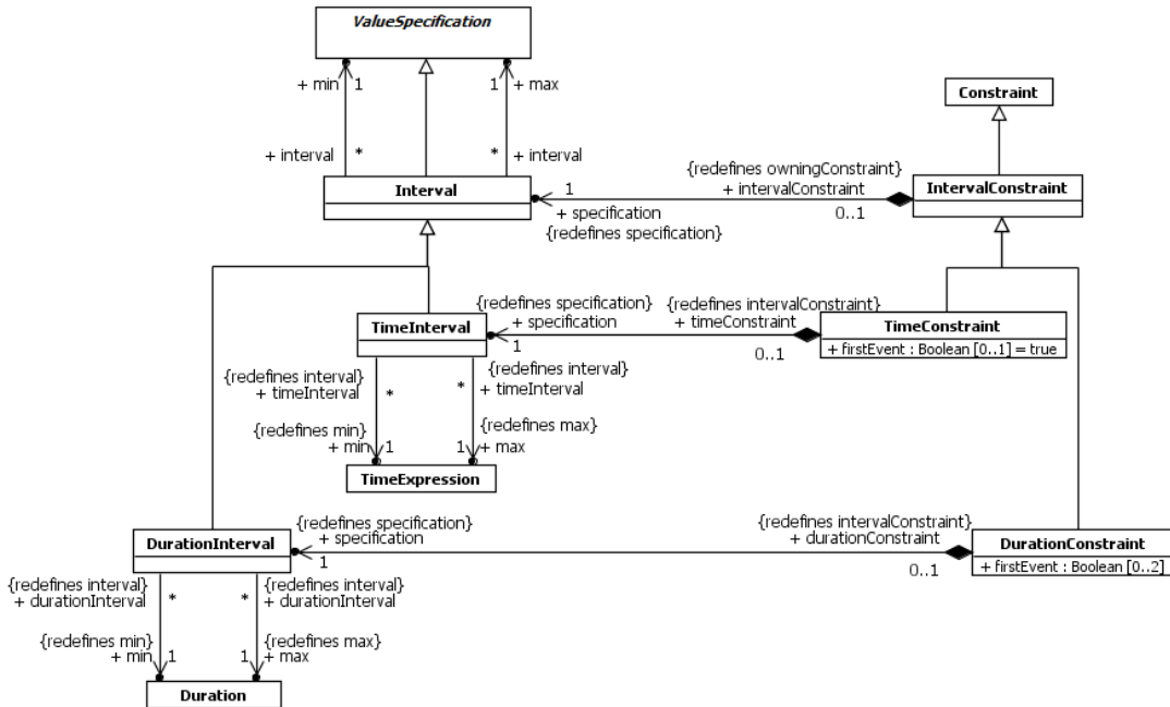
Figure 8.4 Intervals
