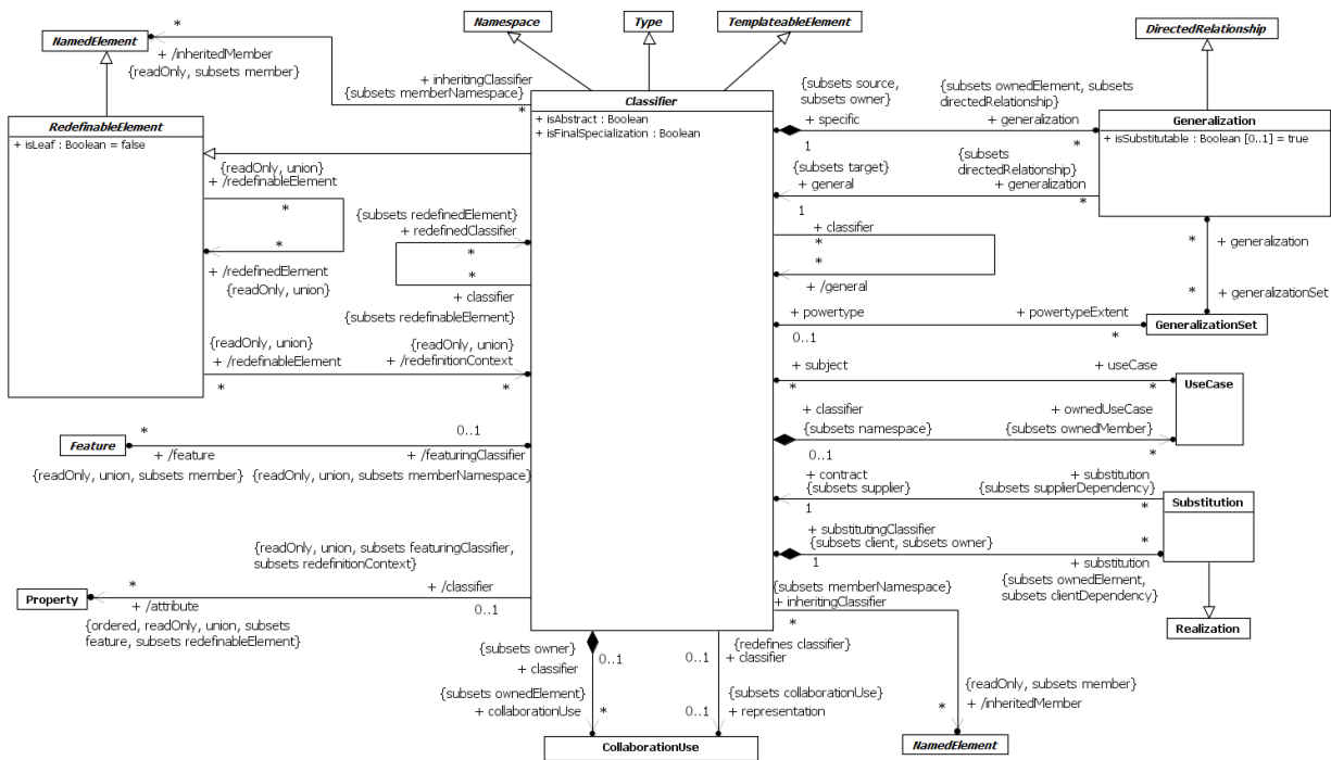
Figure 9.1 Classifiers
