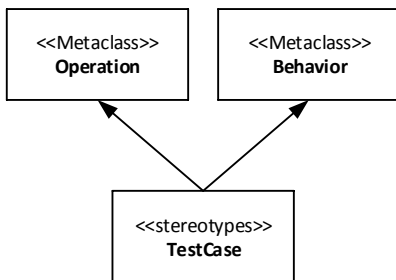
Figure 12.16 Example of Multiple Metaclass Extension
