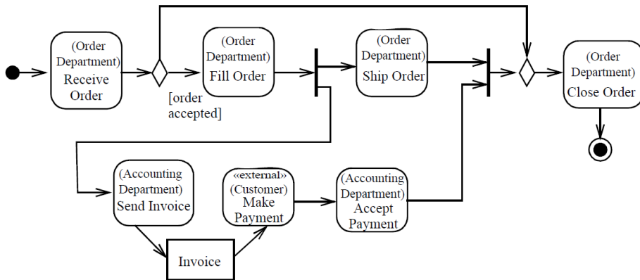
Figure 15.71 ActivityPartitions using annotation
