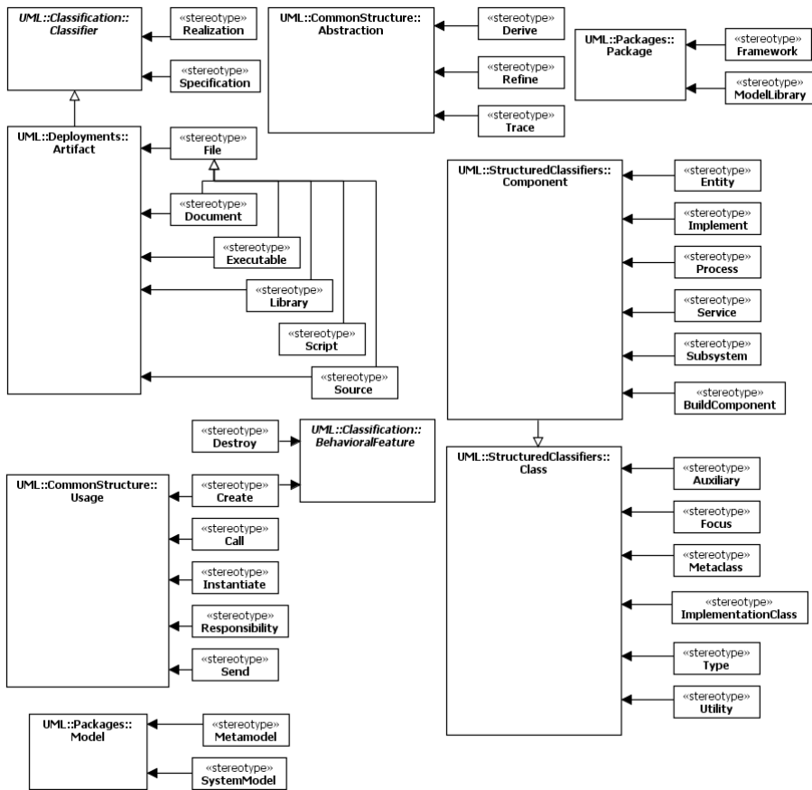
Figure 22.1 Model of StandardProfile
