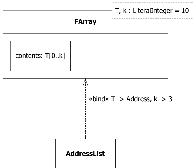
Figure 9.5 Template Class and Bound Class
