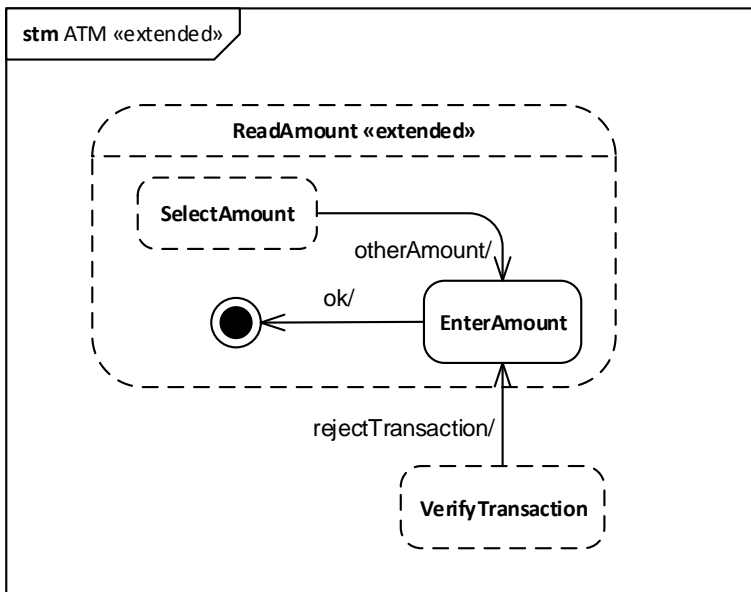
Figure 14.39 An extended StateMachine
