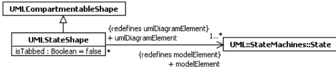
Figure B.14 State Shapes
