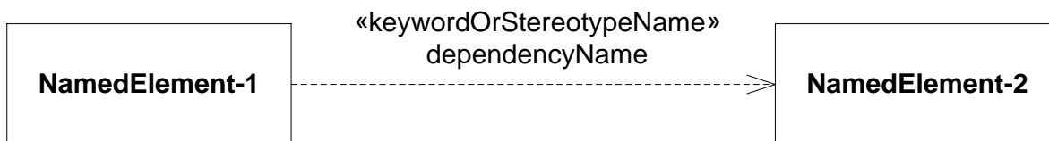
Figure 7.18 Notation for a Dependency between two elements
