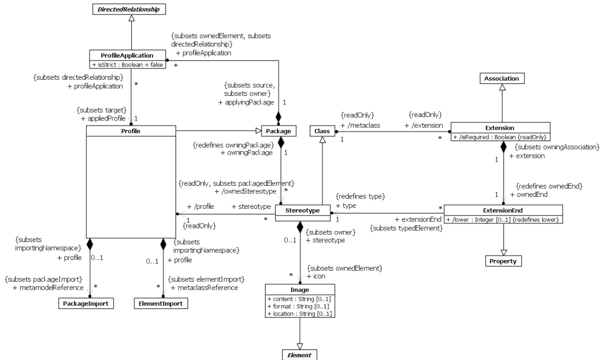
Figure 12.12 Profiles
