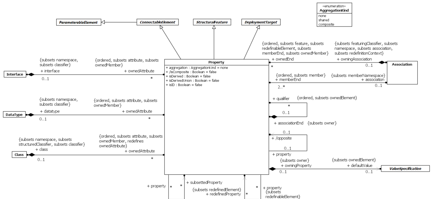
Figure 9.10 Properties
