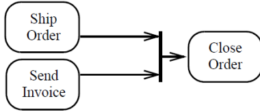
Figure 15.37 JoinNode example
