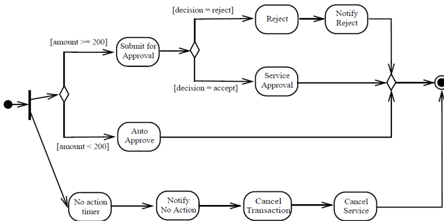
Figure 15.43 ActivityFinalNode example
