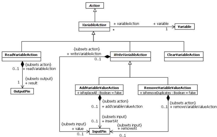
Figure 16.37 Variable Actions
