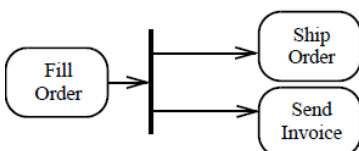
Figure 15.36 ForkNode example
