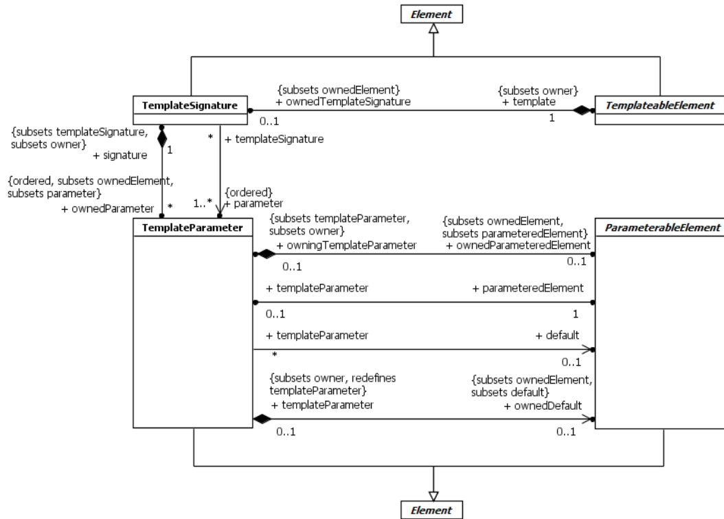
Figure 7.3 Templates
