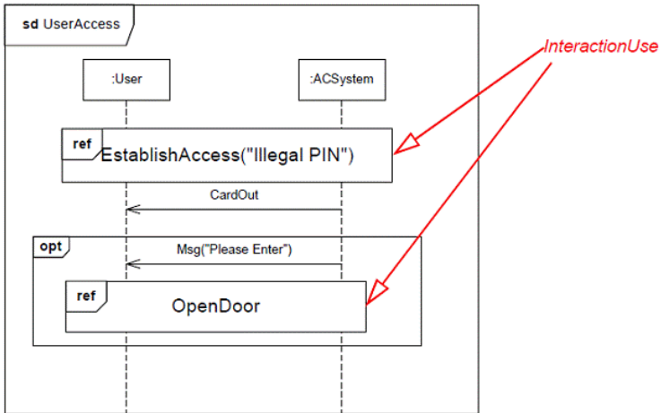
Figure 17.19 InteractionUse
