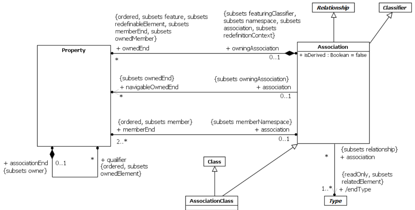
Figure 11.25 Associations
