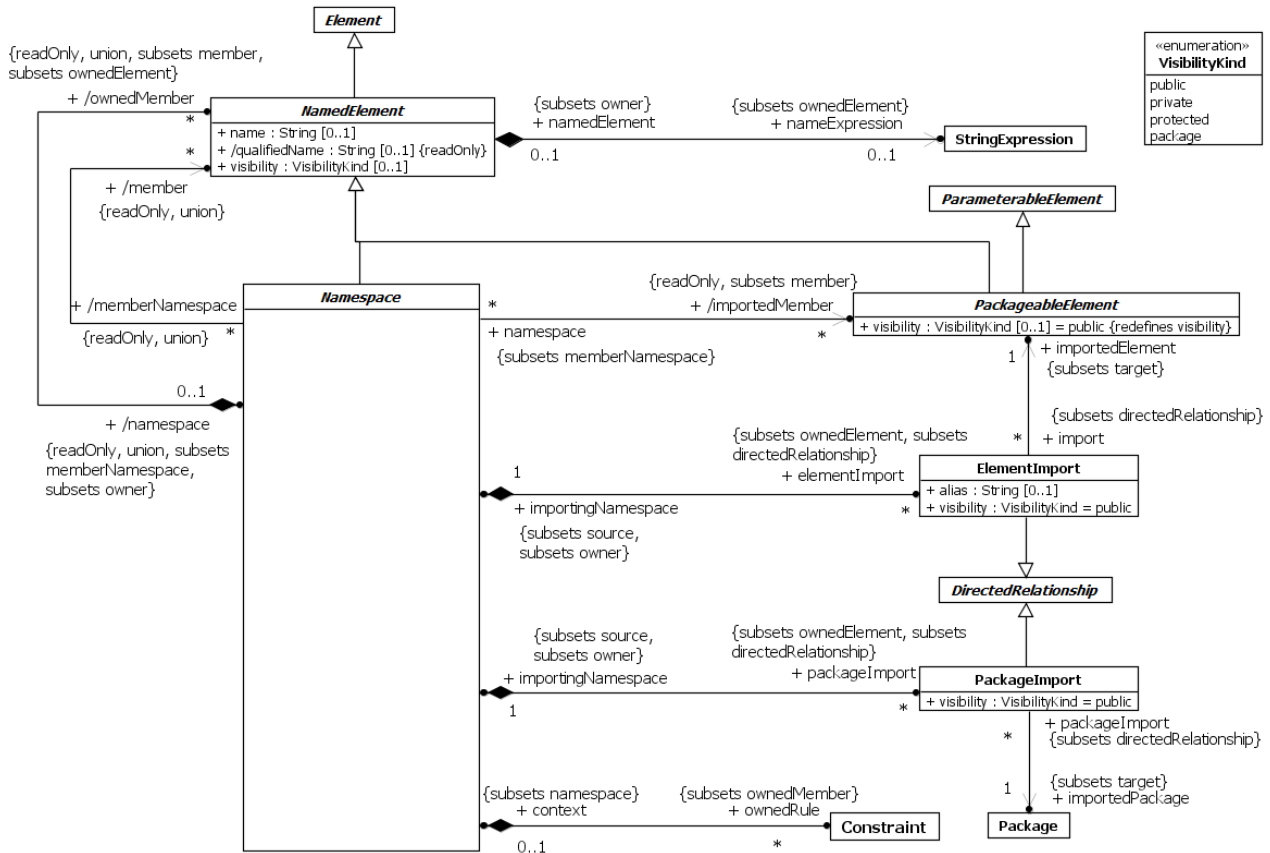
Figure 7.5 Namespaces
