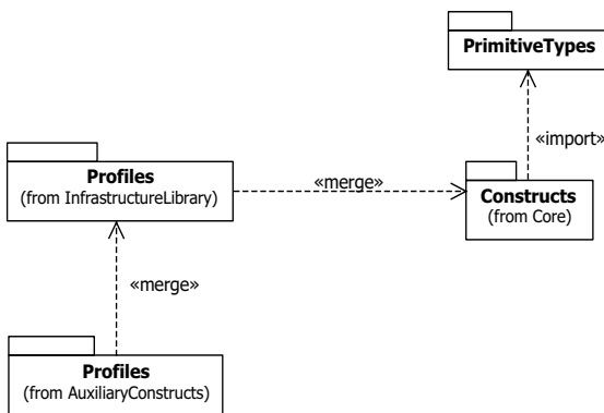
Figure 18.1 - Dependencies between packages described in this clause
