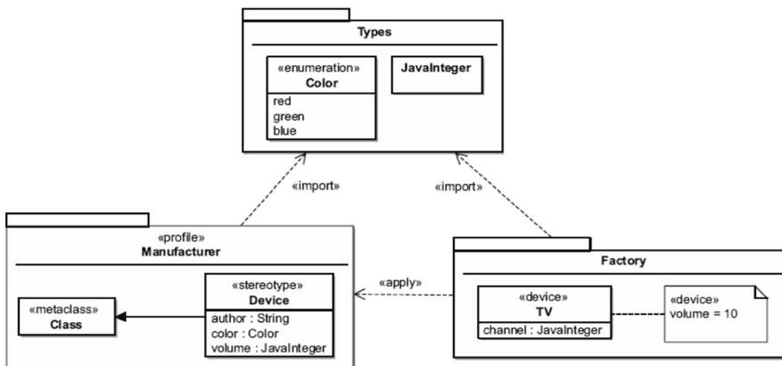
Figure 13.11 - Importing a package from a profile
