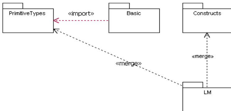
Figure 2.2 - Level M package diagram
