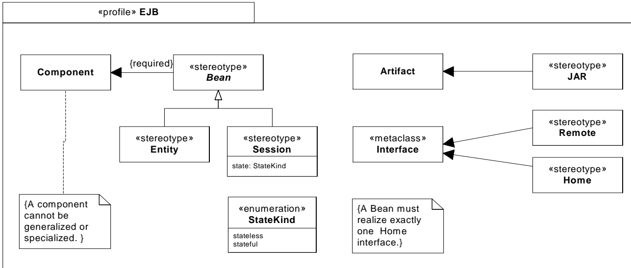
Figure 13.10 - Defining a simple EJB profile
