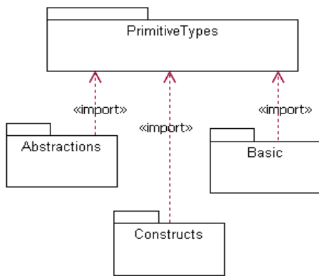
Figure 10.1 - The Core package is owned by the InfrastructureLibrary package, and contains several subpackages
