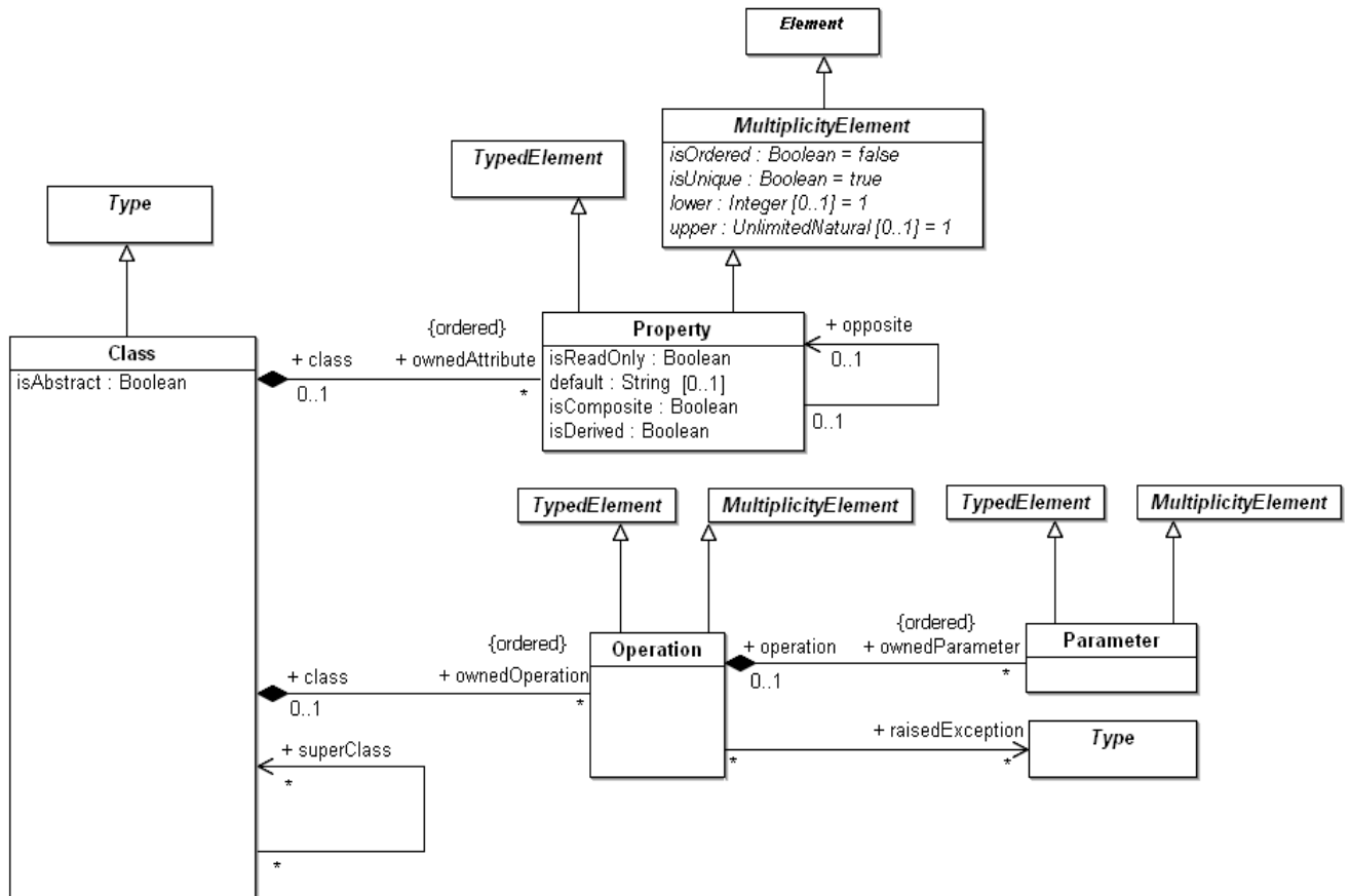
Figure 10.3 - The classes defined in the Classes diagram
