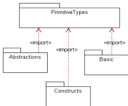
Part II, Figure 2 - The Core package contains the packages PrimitiveTypes, Abstractions, Basic, and Constructs
