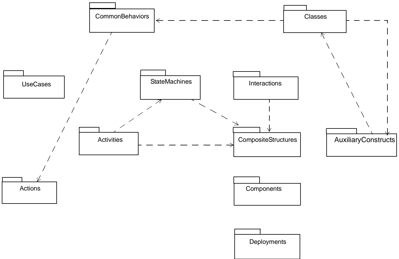
Figure 7.5 - The top-level package structure of the UML 2.3 Superstructure
