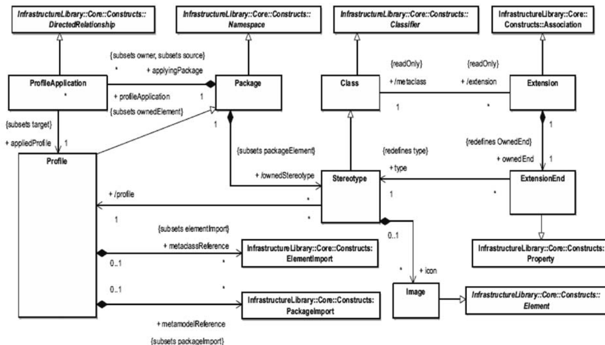
Figure 13.2 - The classes defined in the Profiles package
