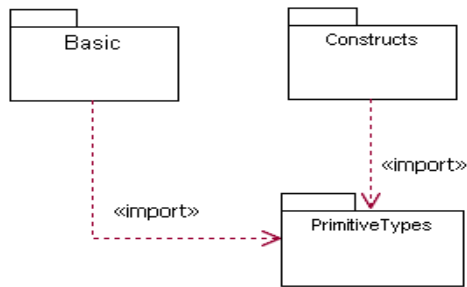
Figure 11.1 -The Core package is owned by the InfrastructureLibrary package, and contains several subpackages
