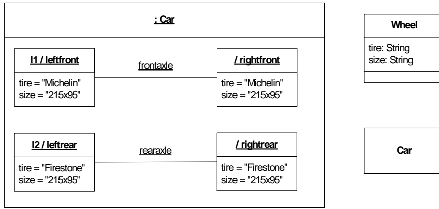
Figure 9.26 - A instance of the Car class
