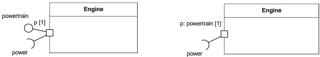
Figure 9.16 - Port notation
