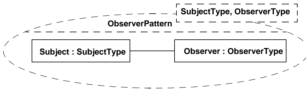
Figure 17.23 - Template Collaboration
