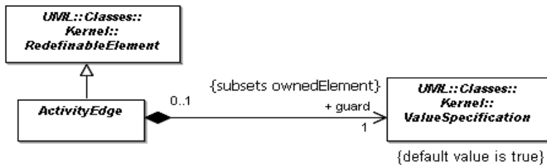
Figure 12.11 - Flows (IntermediateActivities)
