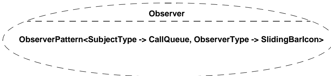
Figure 17.24 - Bound Collaboration
