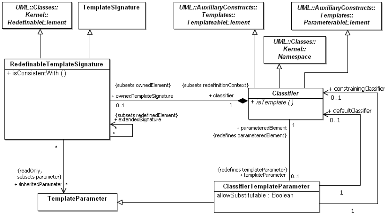
Figure 17.18 - Classifier templates
