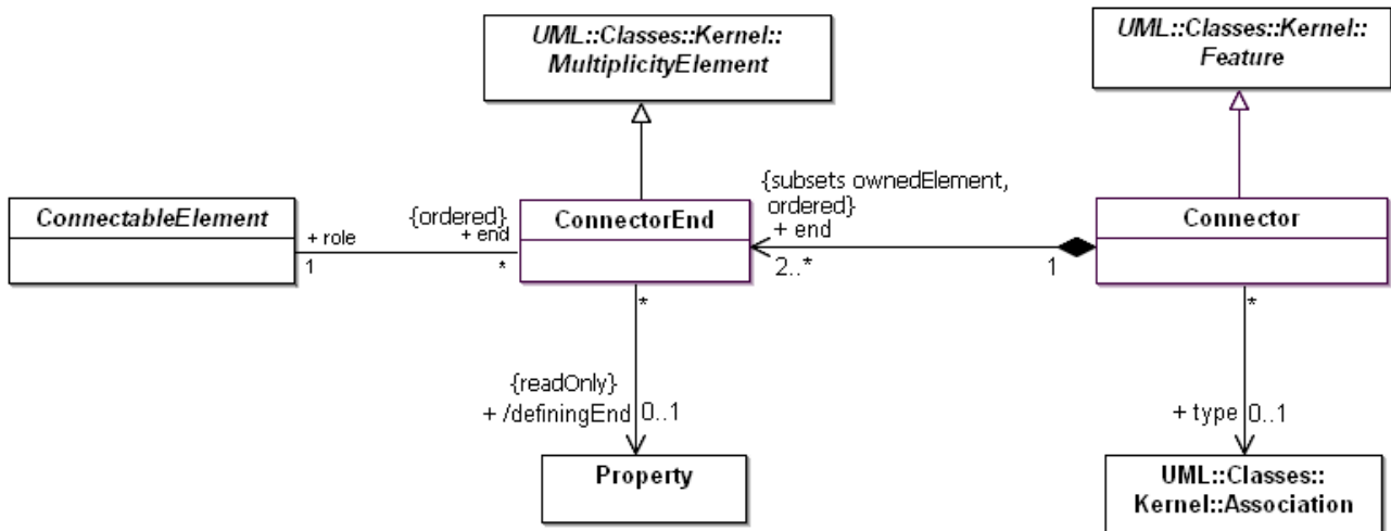
Figure 9.3 - Connectors
