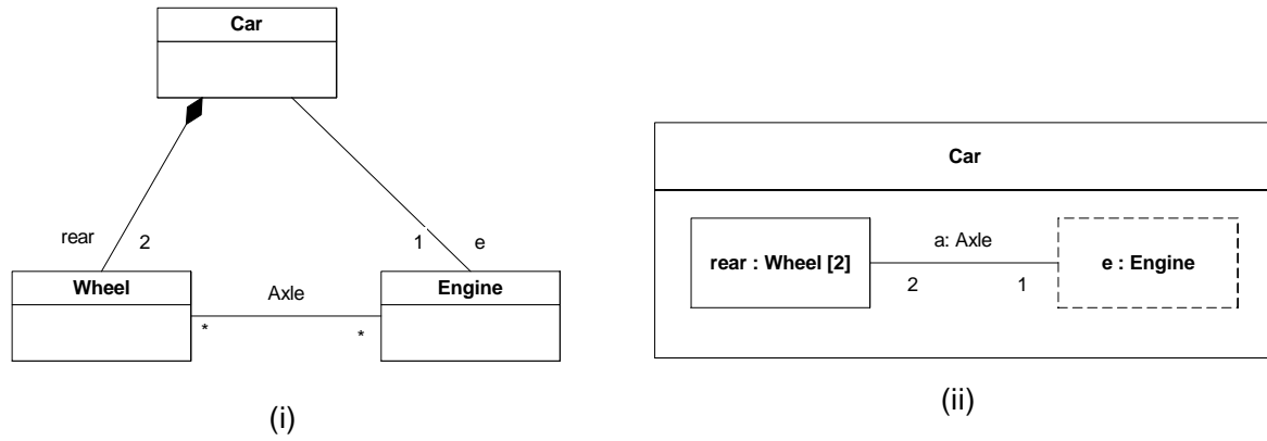
Figure 9.20 - Properties
