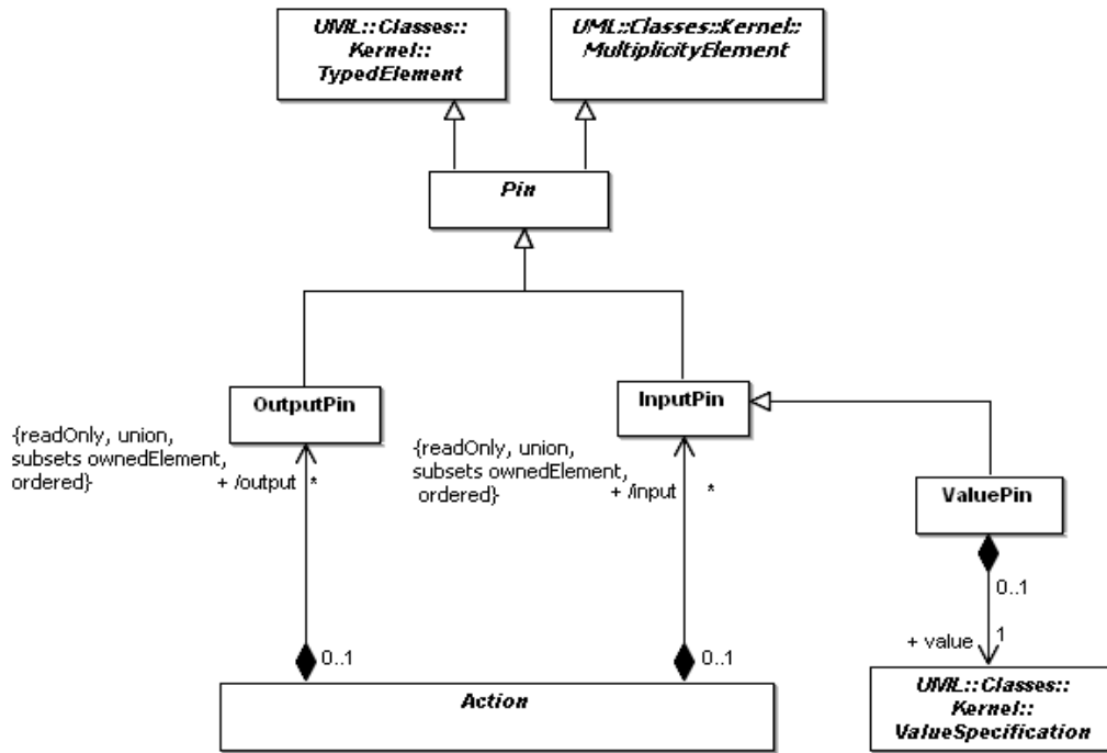
Figure 11.3 - Basic pins
