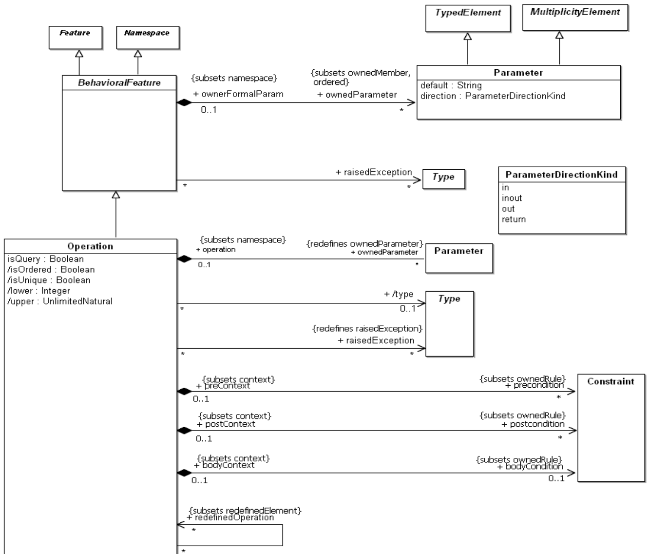
Figure 11.25 - The Operations diagram of the Constructs package
