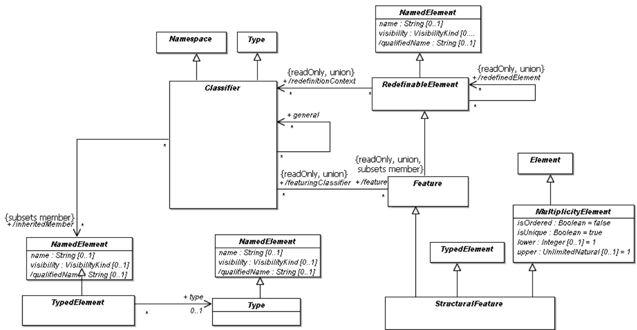
Figure 11.16 - The Classifiers diagram of the Constructs package
