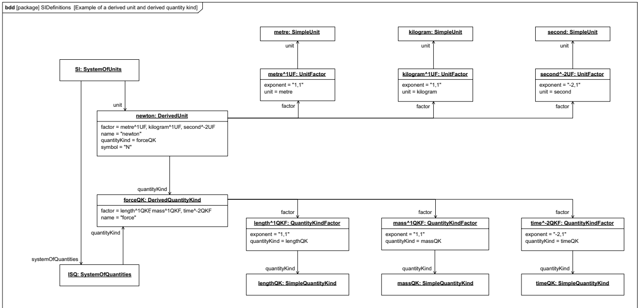
Figure C.12 - Example of a derived unit and derived quantity kind
