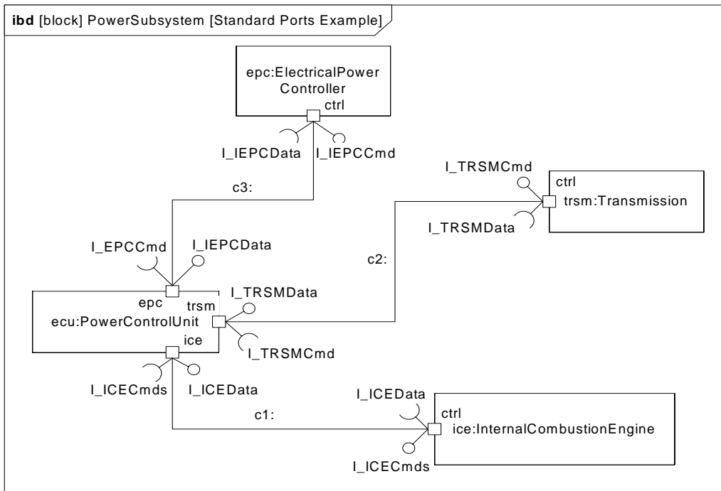
Figure 9.3 - Usage example of standard ports
