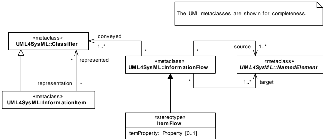
Figure 9.2 - ItemFlow Stereotype
