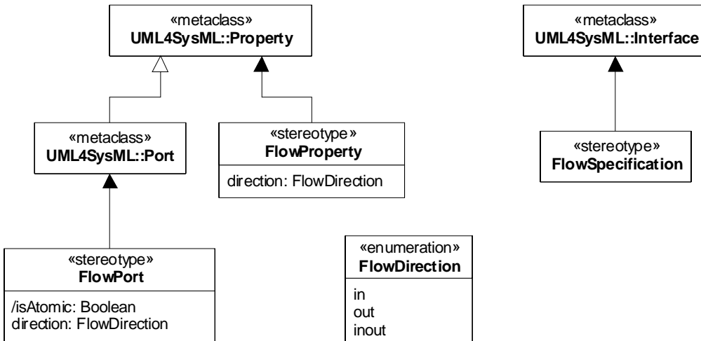
Figure 9.1 - Port Stereotypes
