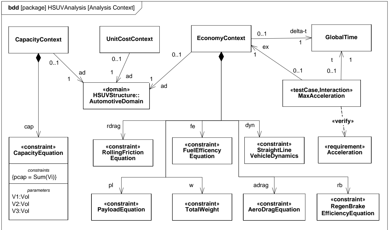
Figure B.26 - Defining Analyses for Hybrid SUV Engineering Development (Block Definition Diagram)
