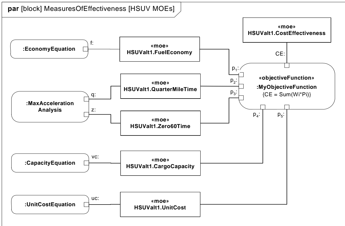
Figure B.28 - Defining Measures of Effectiveness and Key Relationships (Parametric Diagram)
