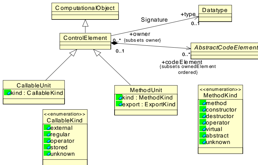
Figure 12.4 - ControlElements Class Diagram
