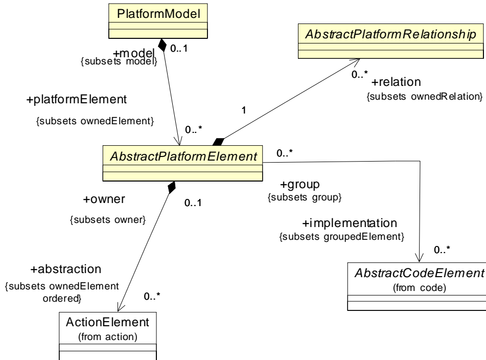
Figure 15.1 - PlatformModel Class Diagram
