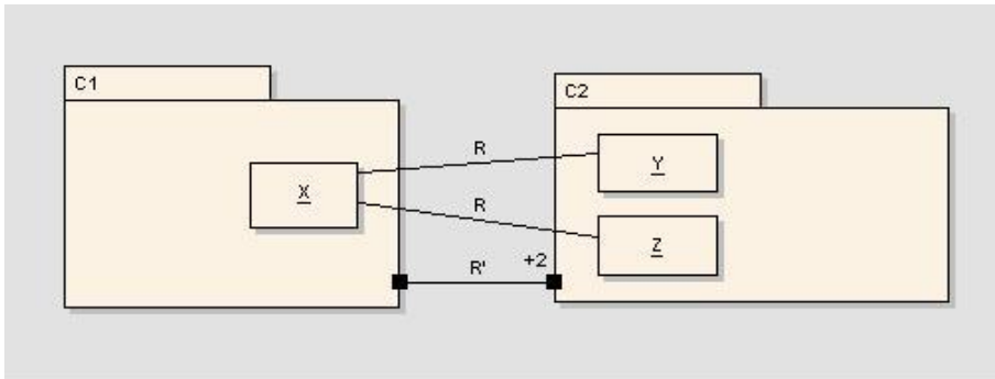
Figure 9.4 - AggregatedRelations illustrated
