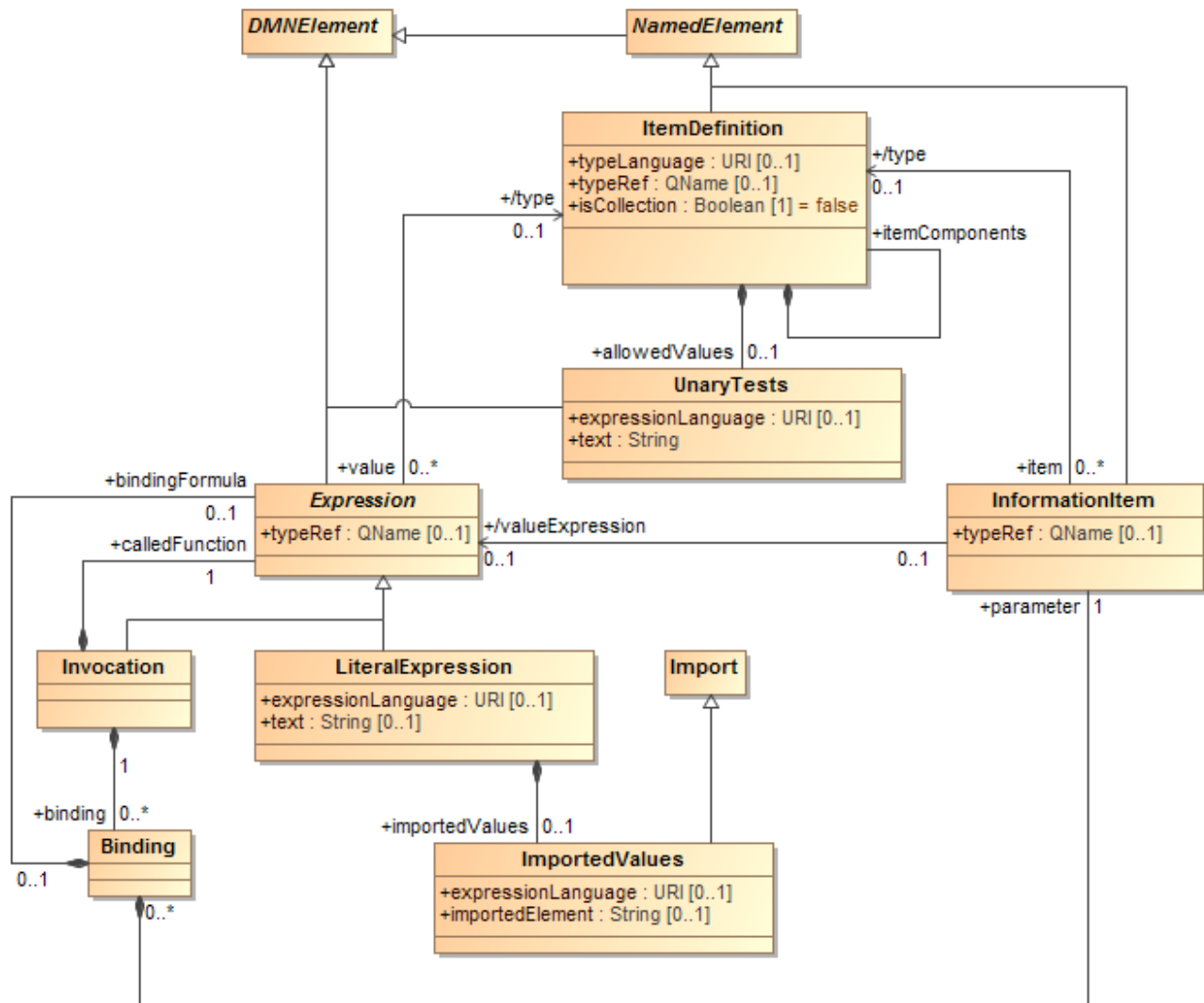
Figure 7.6: Expression class diagram
