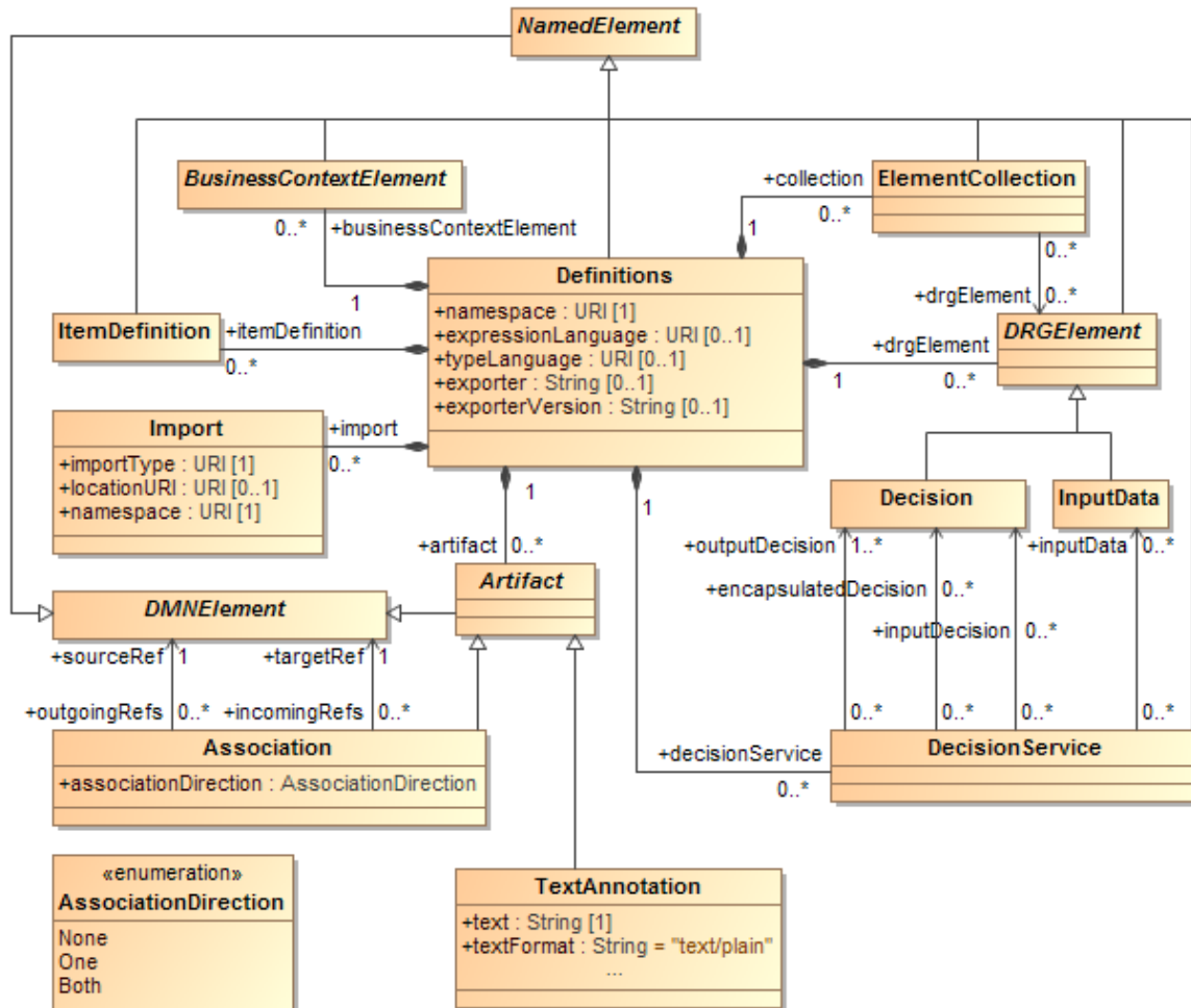
Figure 6.8: Definitions Class Diagram
