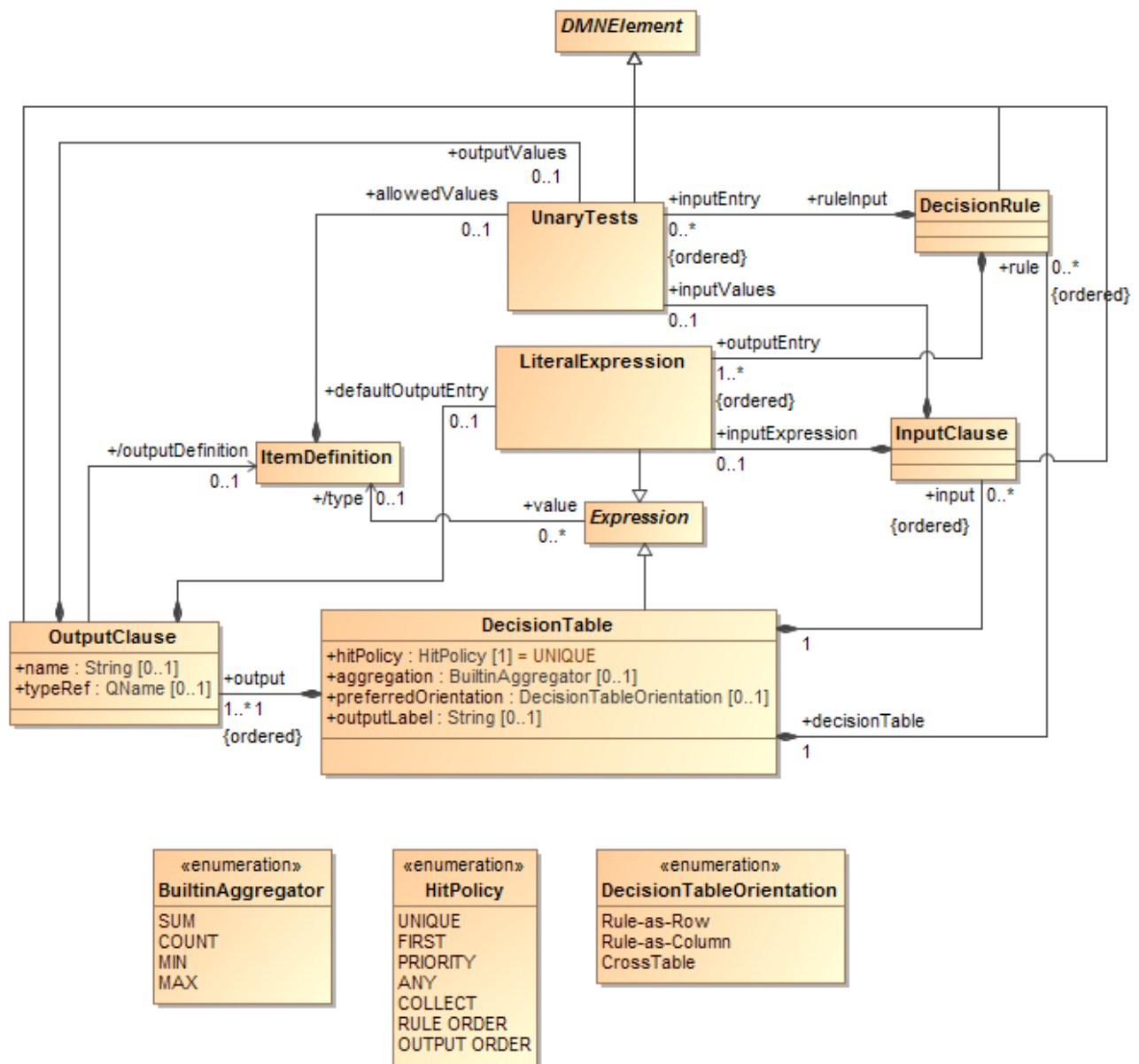
Figure 8.20: DecisionTable class diagram
