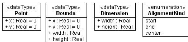
Figure 8.2 - The layout data types
