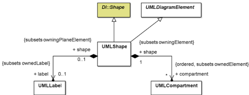
Figure A.2 - UML Shape
