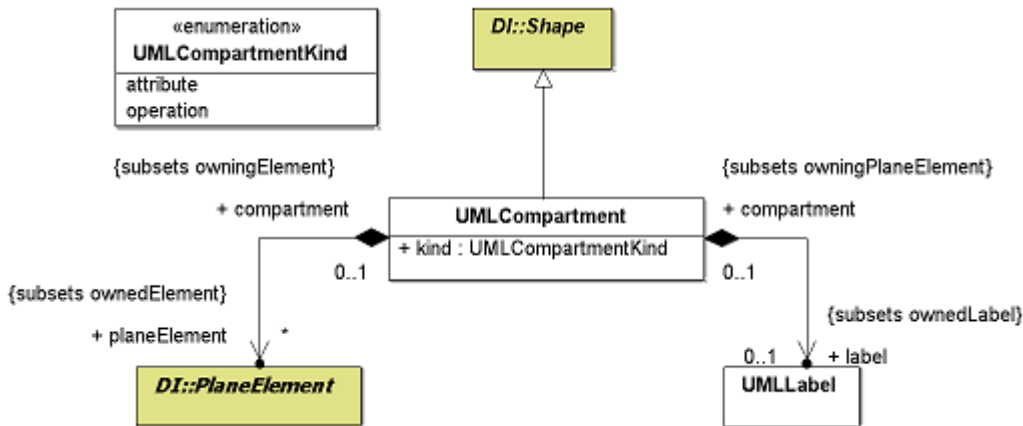
Figure A.5 - UML Compartment
