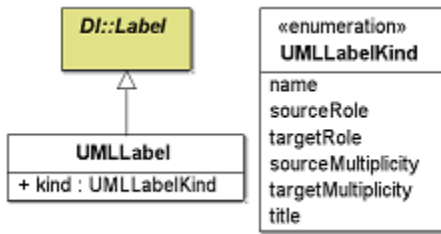
Figure A.6 - UML Label
