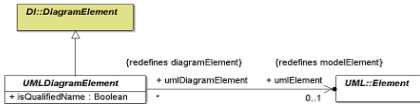
Figure A.4 - UML DiagramElement
